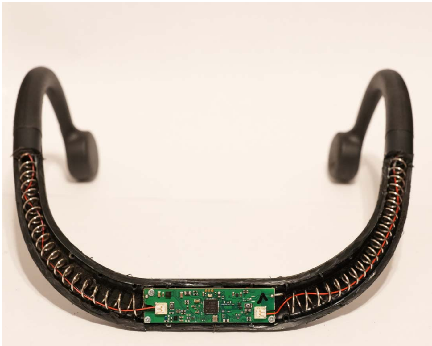
Figure 1 – Internal photo of Zygo2 Headset
