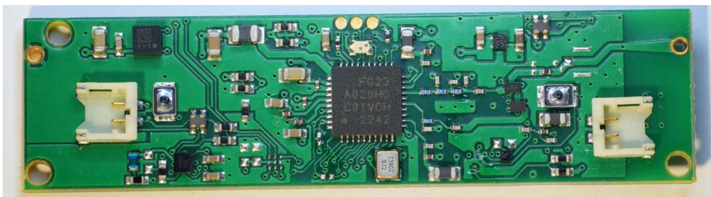
Figure 2 – PWB Front of Zygo2 Headset
