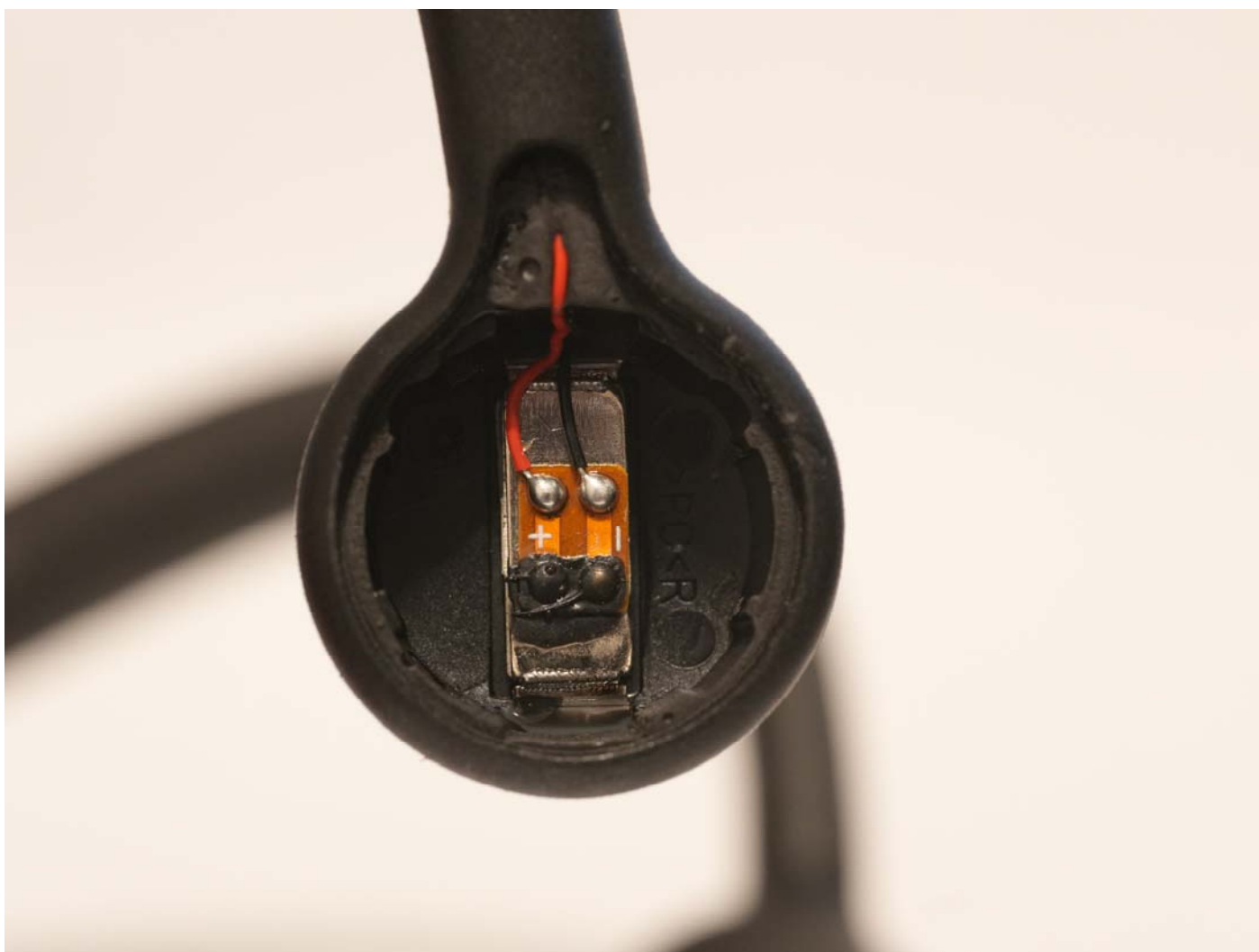
Figure 4 – Internal photo of Zygo2 Headset ear piece
