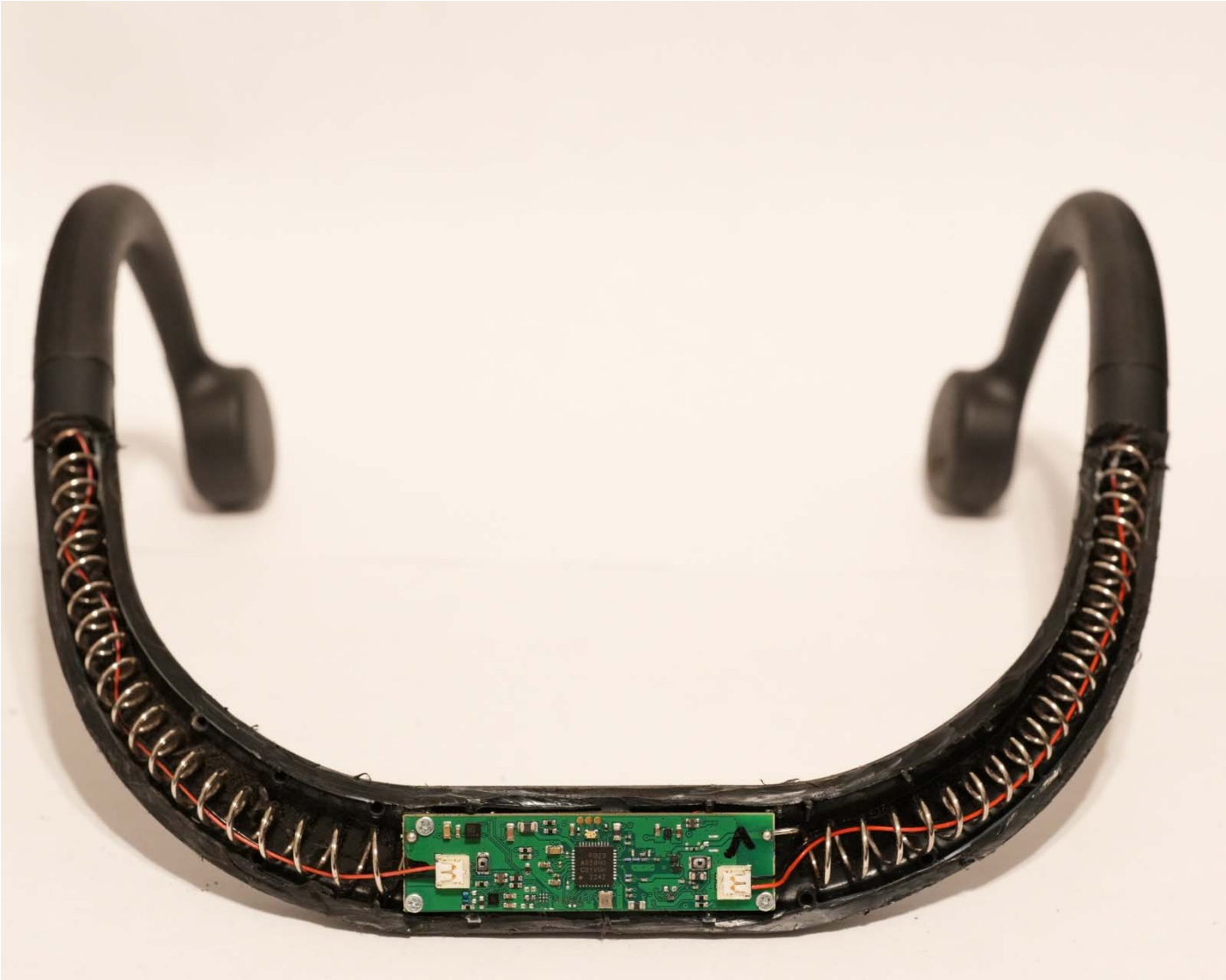
Figure 1 – Internal photo of Zygo2 Headset antenna
