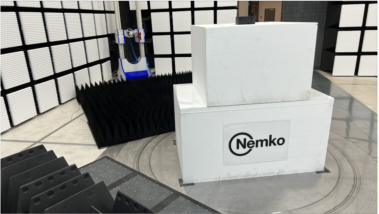
Radiated Emissions, 1 GHz to 26.5 GHz
