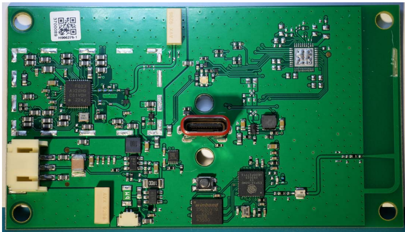
Figure 4 – Bluetooth RF Section of Zygo2 Transmitter
