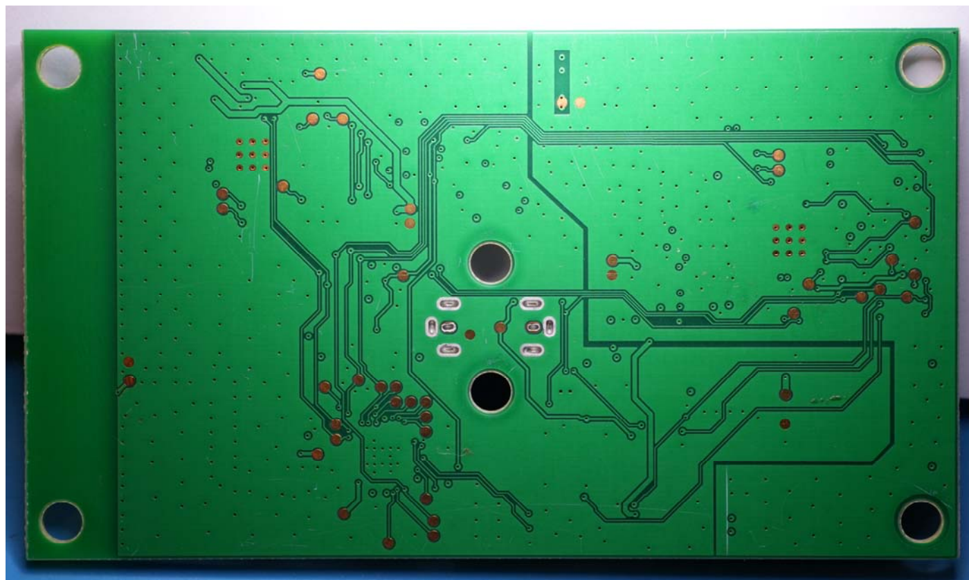
Figure 3 - PWB back of Zygo2 Transmitter
