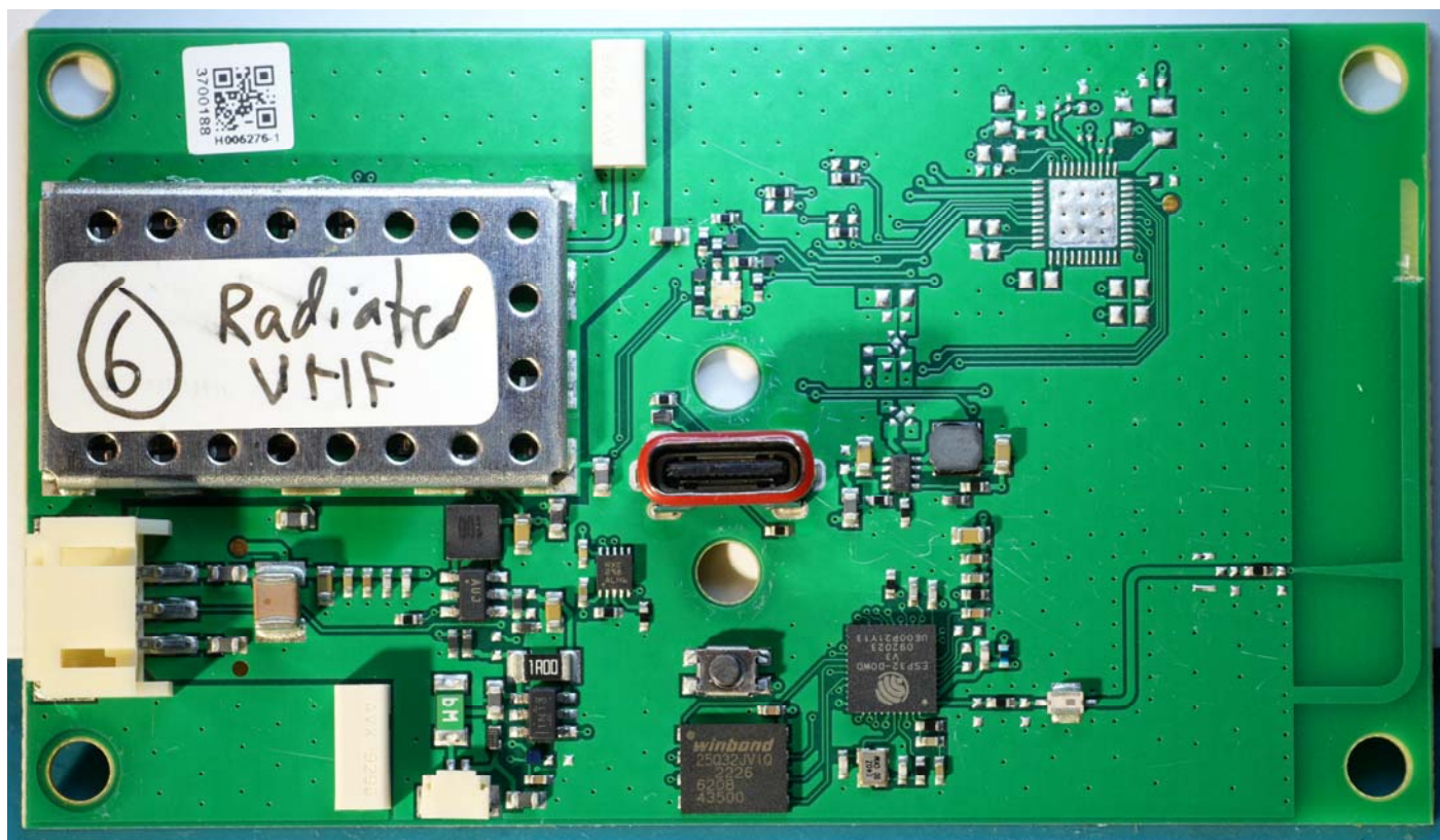
Figure 2 – PWB Front of Zygo2 Transmitter
