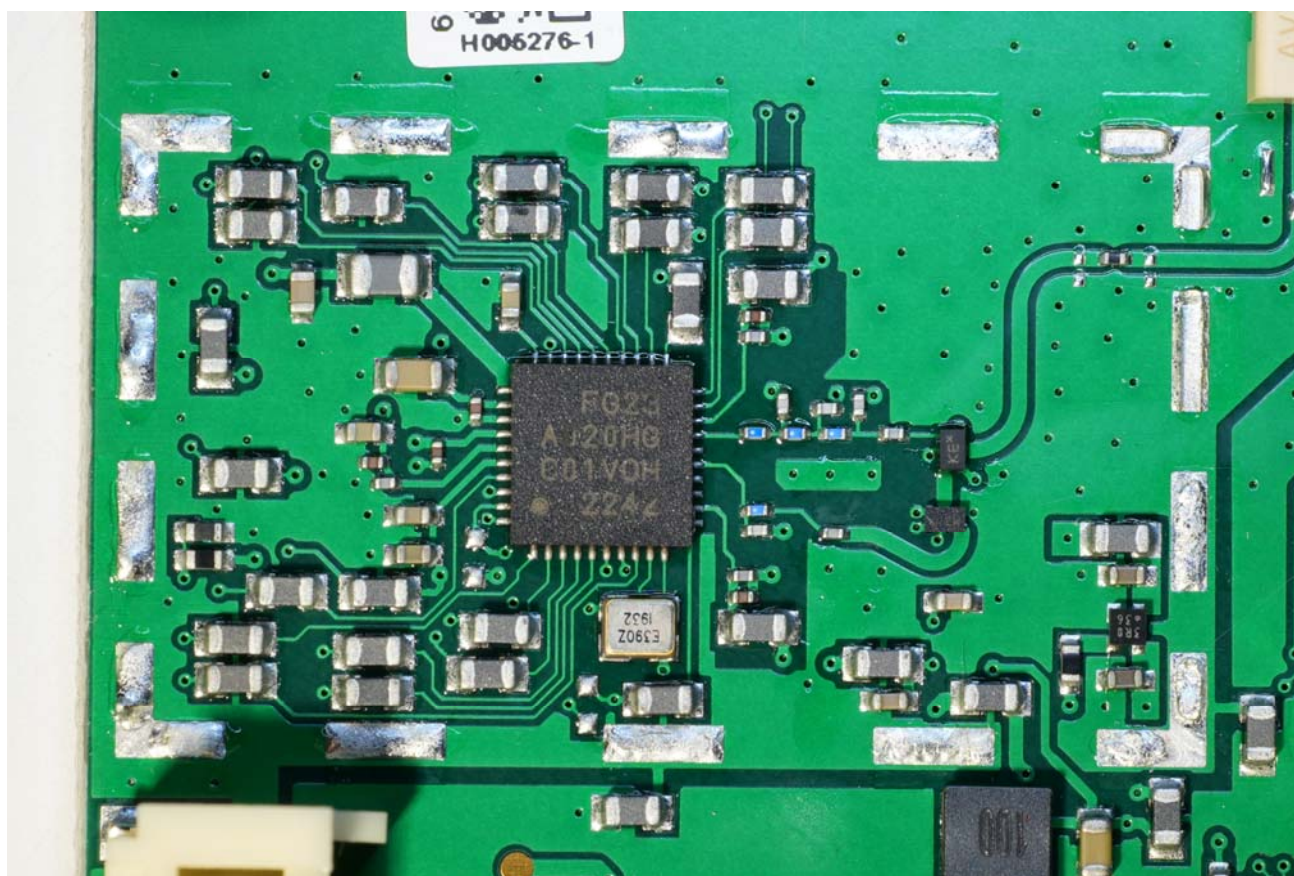
Figure 5 – Bluetooth Low Frequency Radio RF Section of Zygo2 Transmitter
