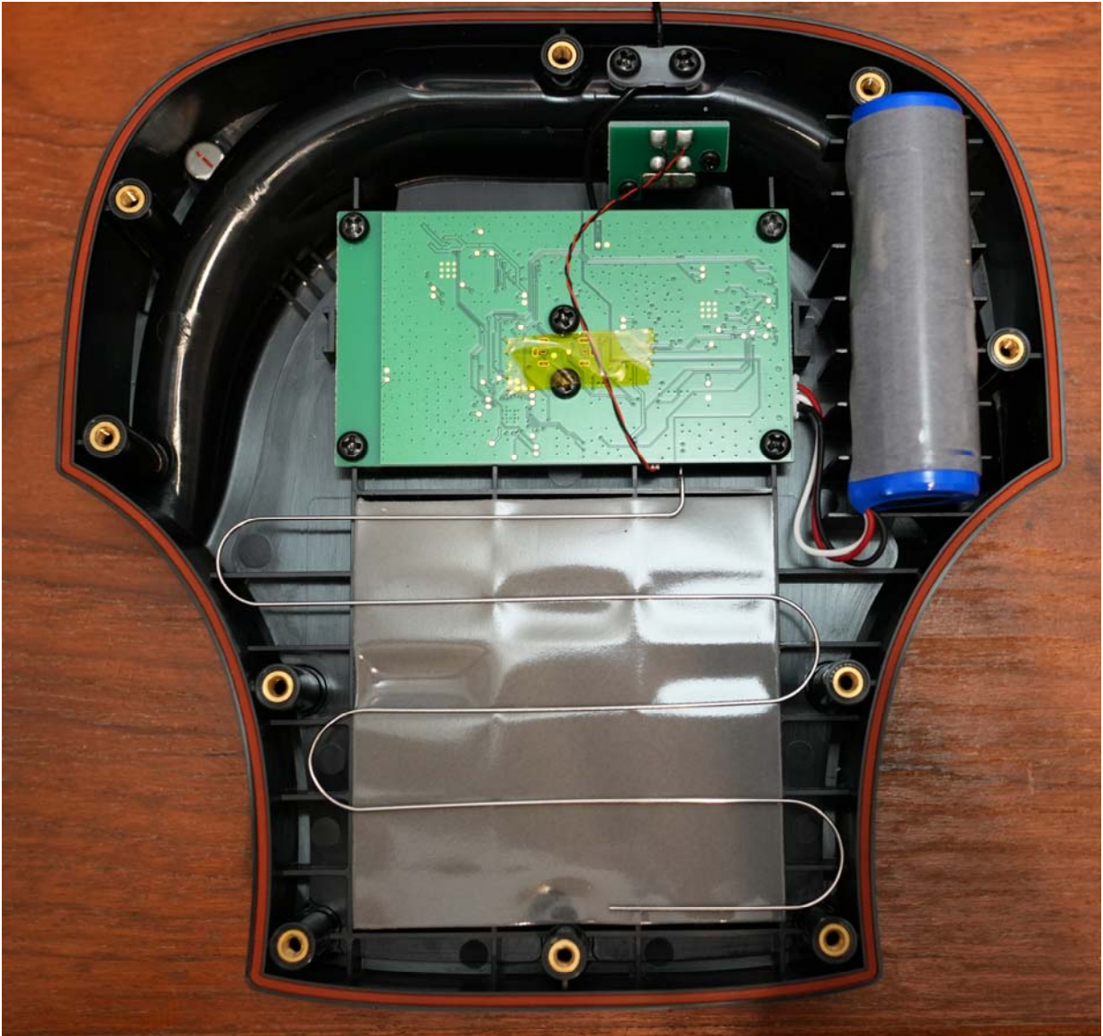
Figure 1 – Interior of Zygo2 Transmitter
