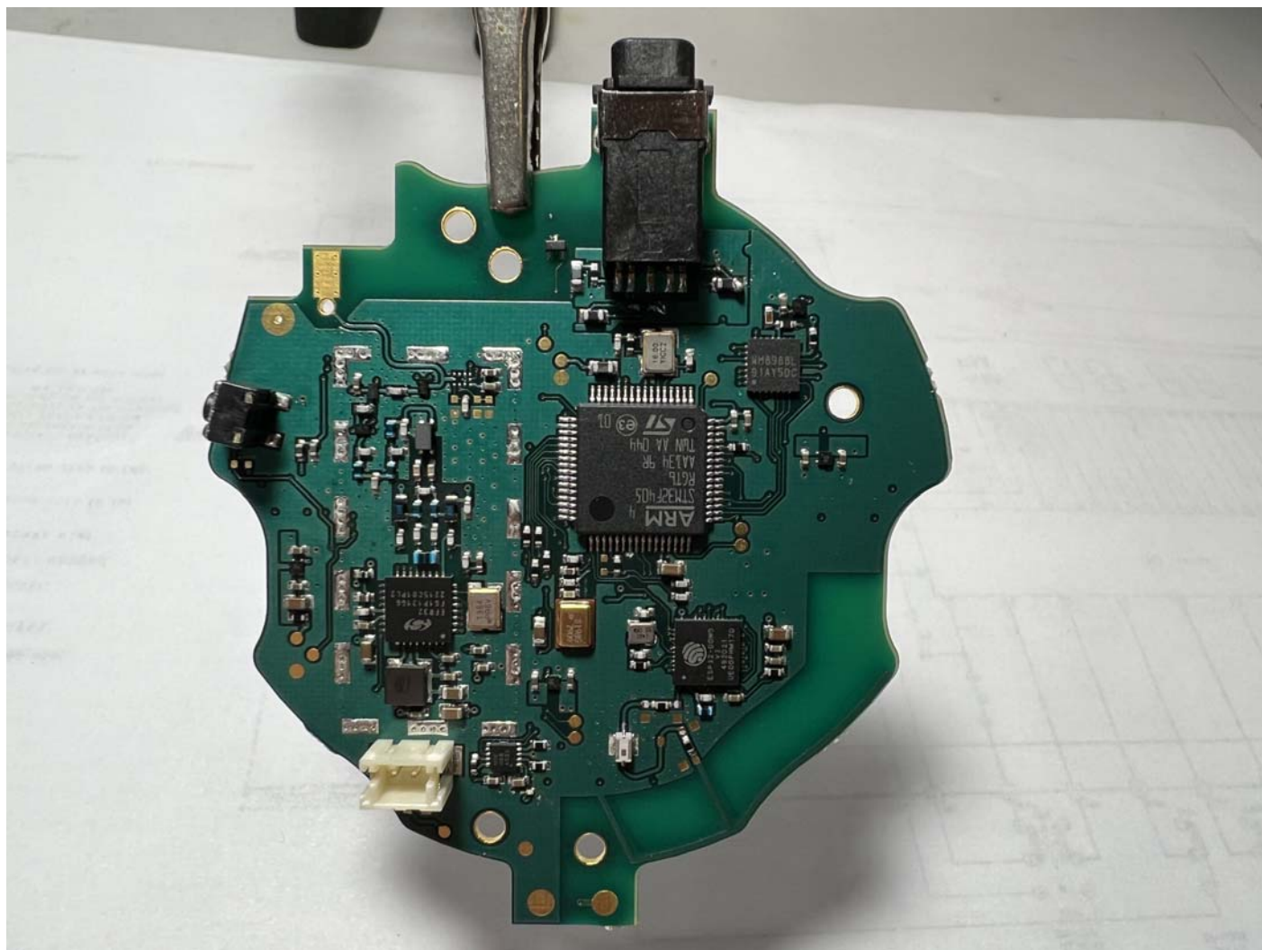
Figure 2 - PWB front side with shield removed
