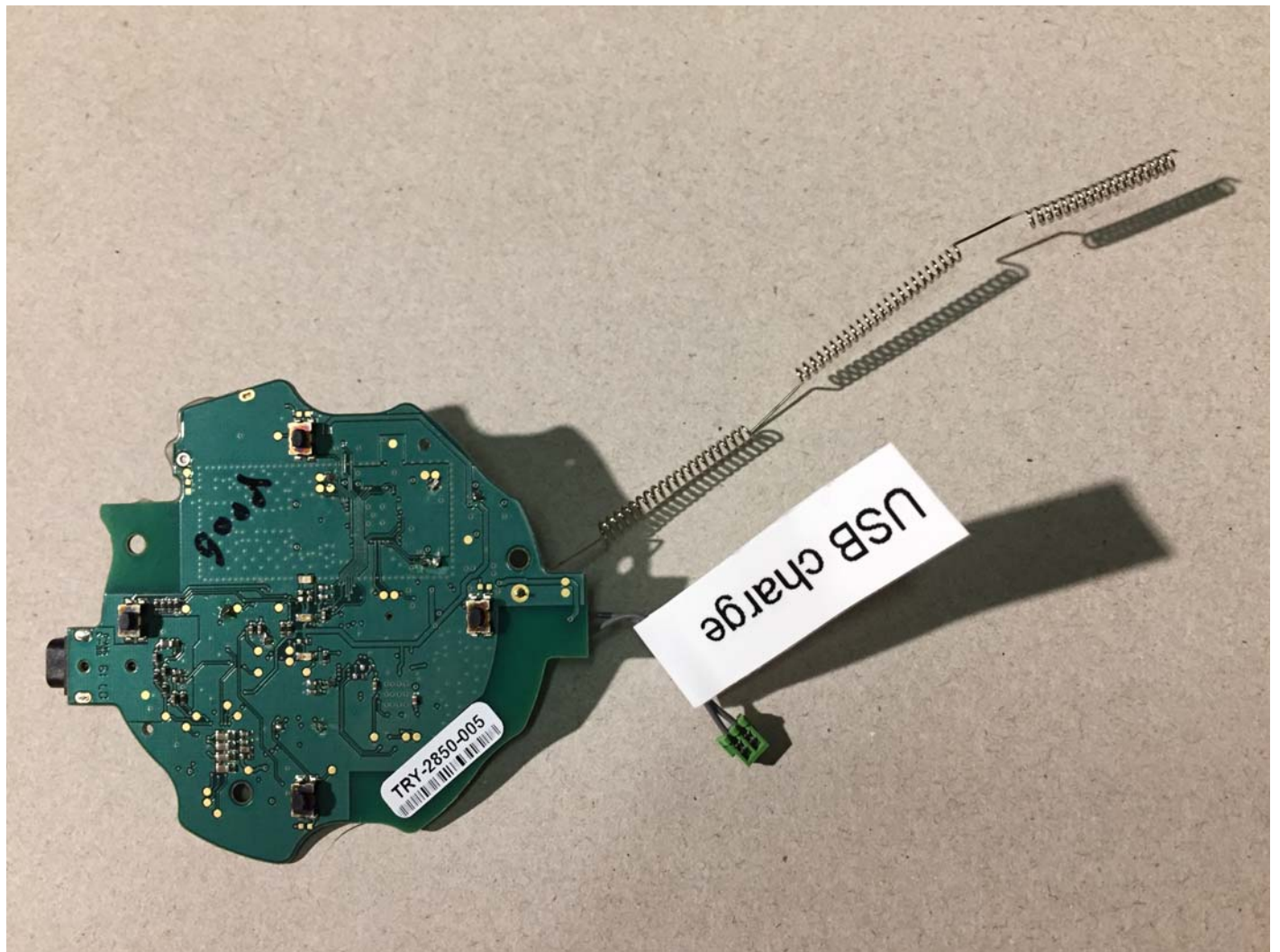
Figure 3 - PWB back side with shield removed
