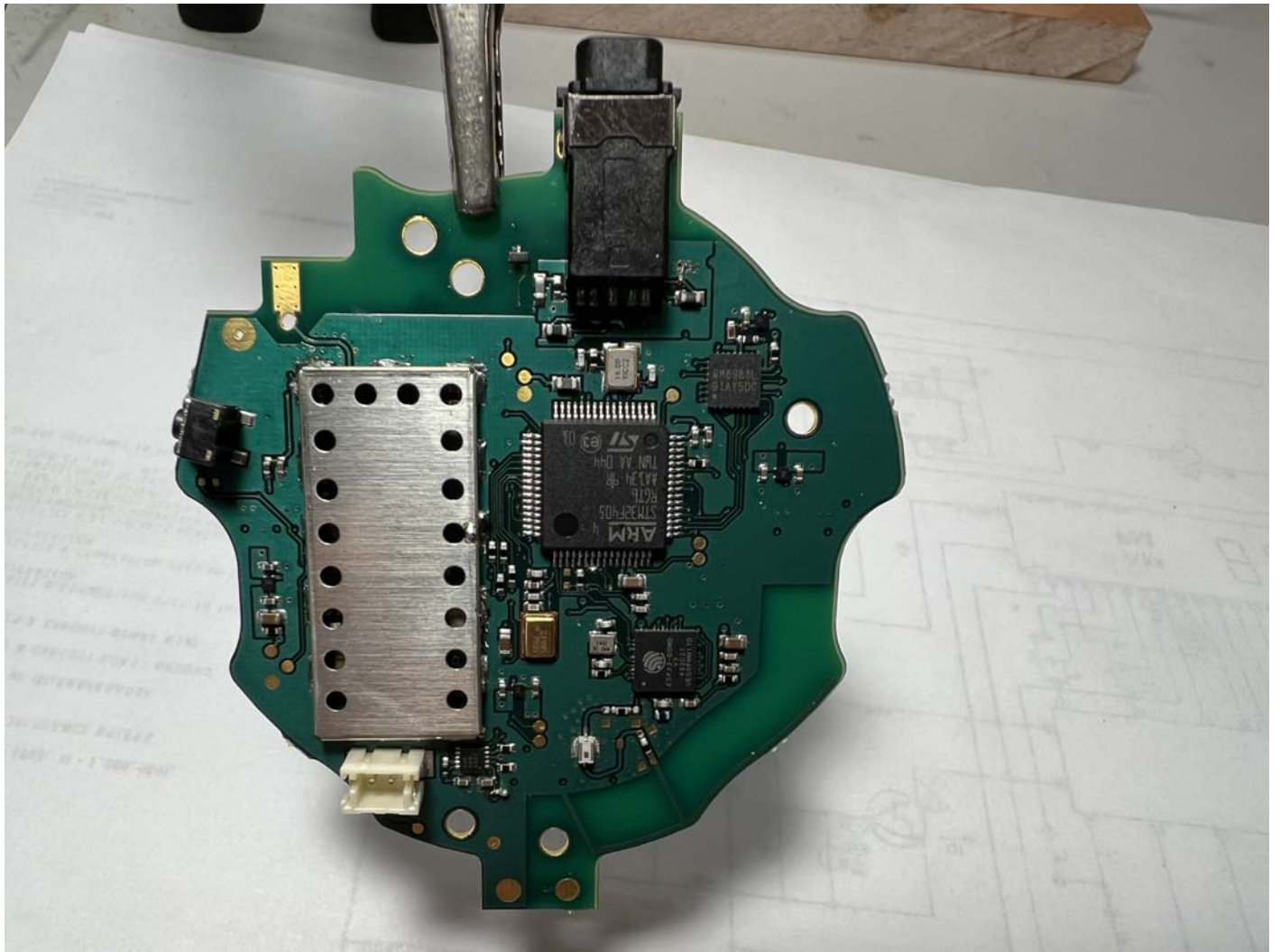
Figure 4 - RF Section with Shield in Place
