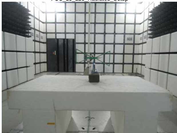
FCC 15 225 Radiated Setup
