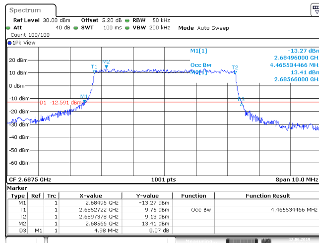
Band41_5MHz_QPSK_41565_25RB#0
