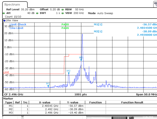
Band41_5MHz_QPSK_39675_1RB#0
