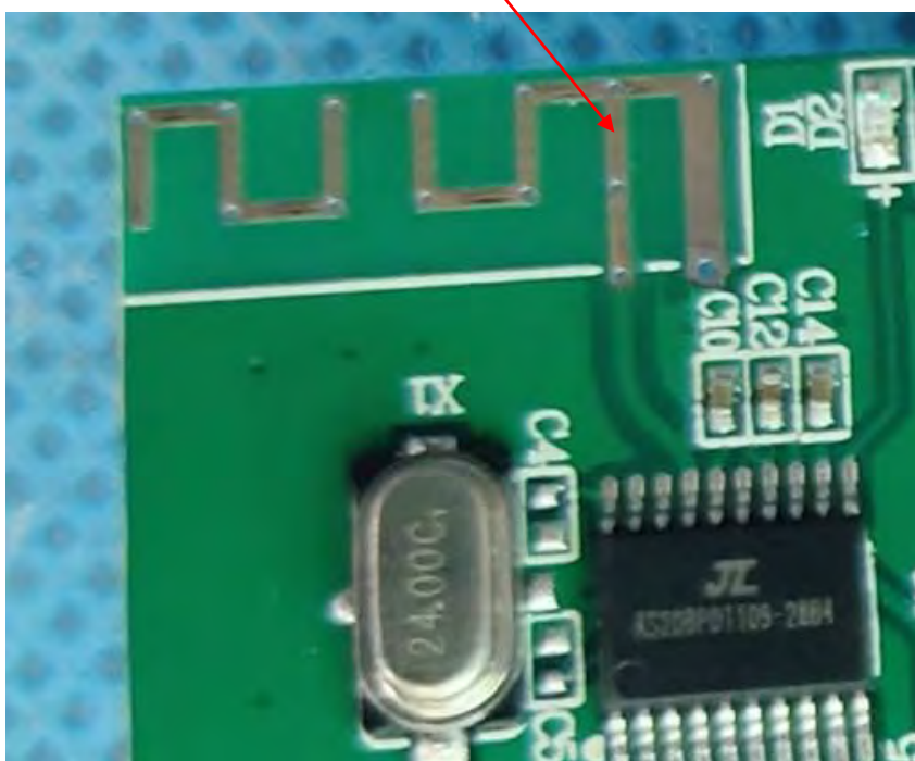
PCB Antenna
