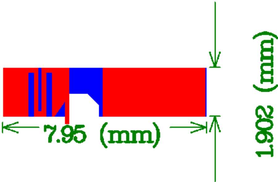
Antenna Photo & Length (mm)
