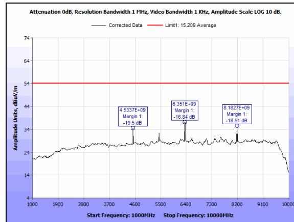
Plot 28. Radiated Spurious Emissions - 908.1 MHz - 1-10 GHz - Average – Vertical
