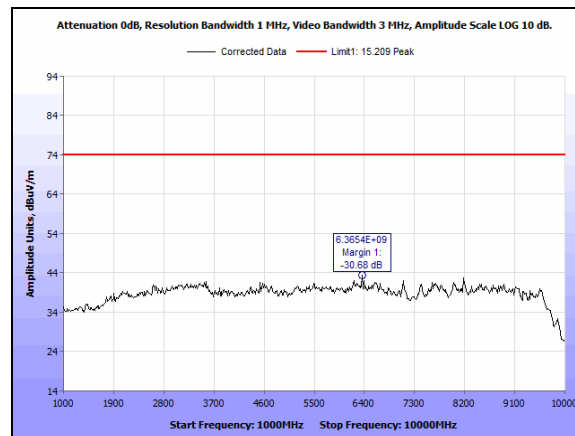
Plot 30. Radiated Spurious Emissions - 908.1 MHz - 1-10 GHz - Peak – Vertical
