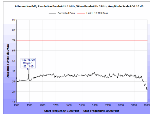
Plot 29. Radiated Spurious Emissions - 908.1 MHz - 1-10 GHz - Peak – Horizontal
