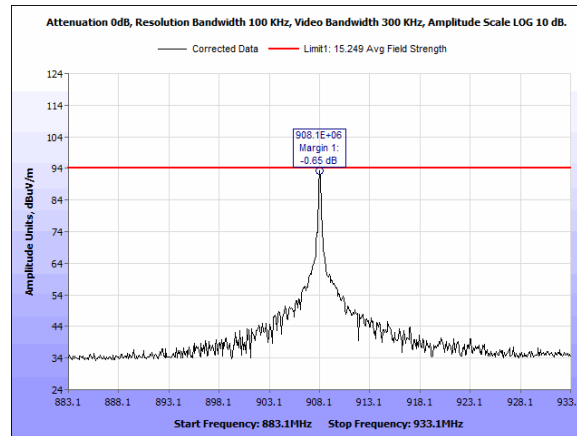
Plot 4. Output Power - 908.1 MHz - Peak – Horizontal
