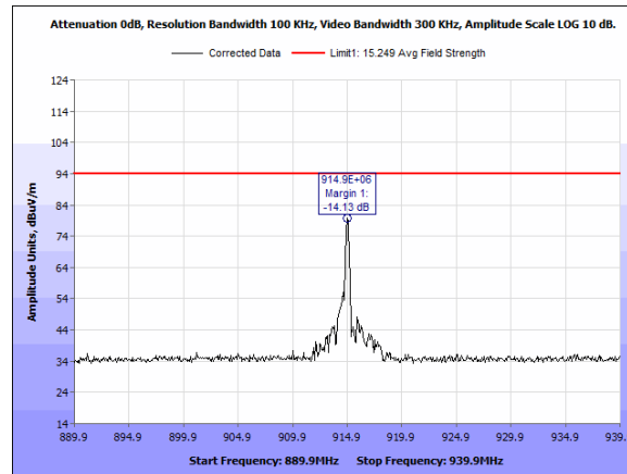
Plot 5. Output Power - 914.9 MHz - Peak – Vertical
