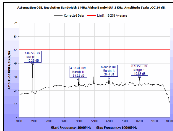
Plot 27. Radiated Spurious Emissions - 908.1 MHz - 1-10 GHz - Average – Horizontal
