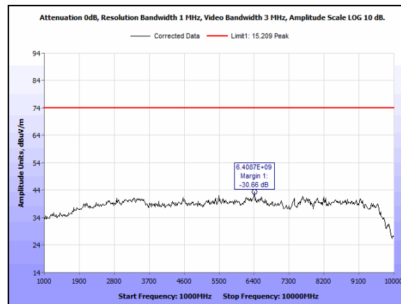
Plot 18. Harmonic Spurious Emissions - 914.9 MHz - 1-10 GHz - Peak – Vertical
