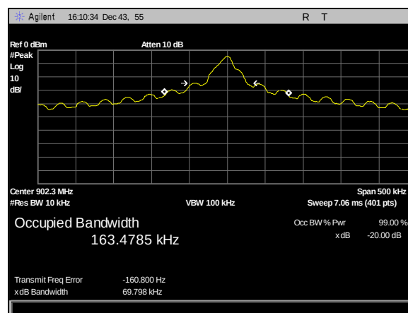
Plot 45. Occupied BW - 902.3MHz
