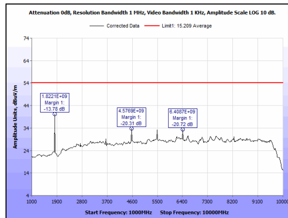
Plot 33. Radiated Spurious Emissions - 914.9 MHz - 1-10 GHz - Average – Horizontal
