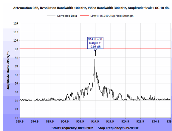
Plot 6. Output Power - 914.9 MHz - Peak – Horizontal
