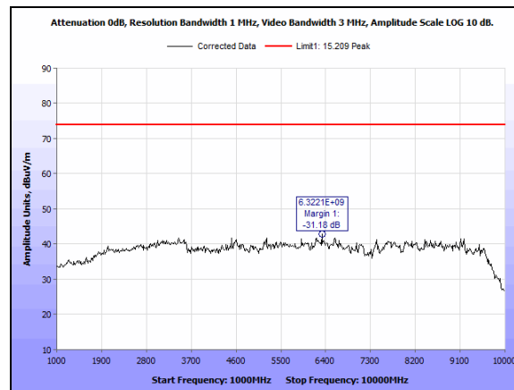
Plot 24. Radiated Spurious Emissions - 902.3 MHz - 1-10 GHz - Peak – Vertical
