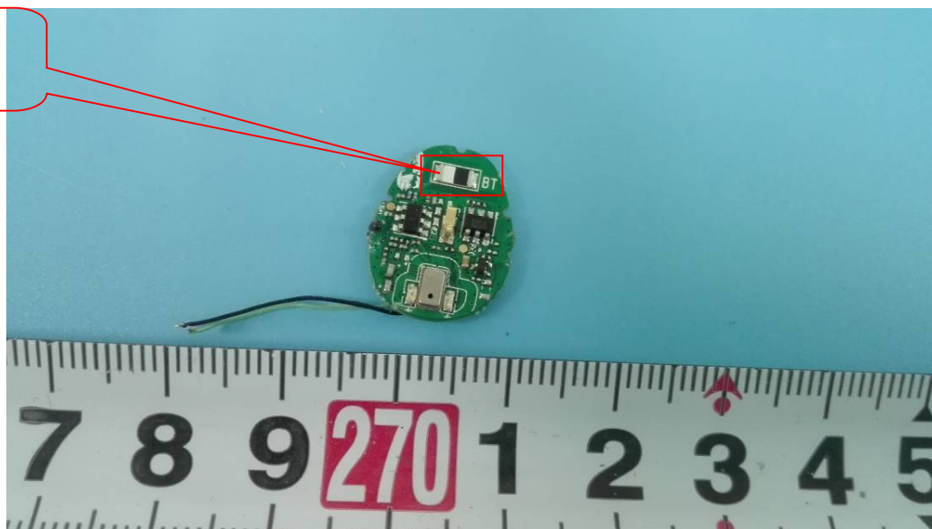
Bluetooth Antenna
