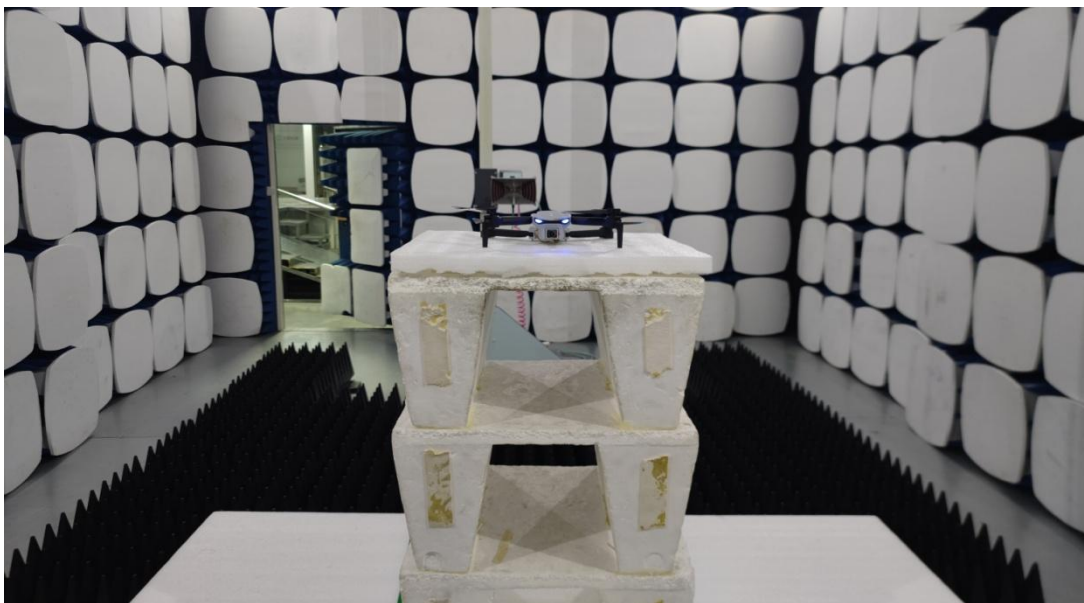
Radiated Emission (Above 1GHz)
