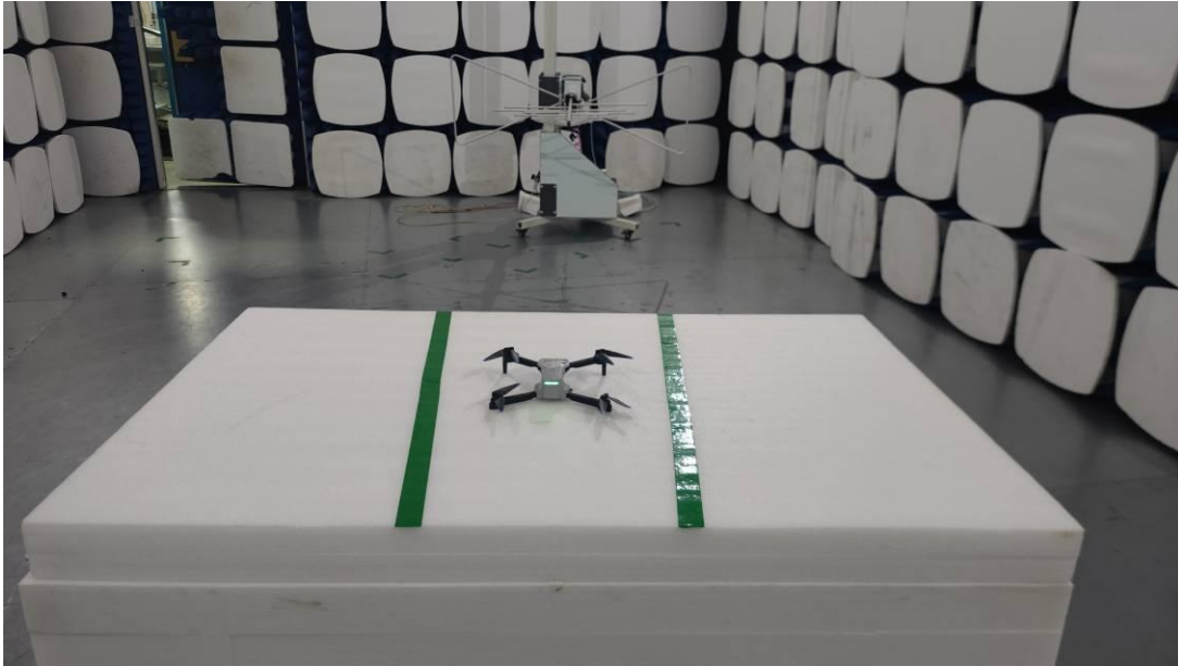
Radiated Emission (Above 1GHz)
