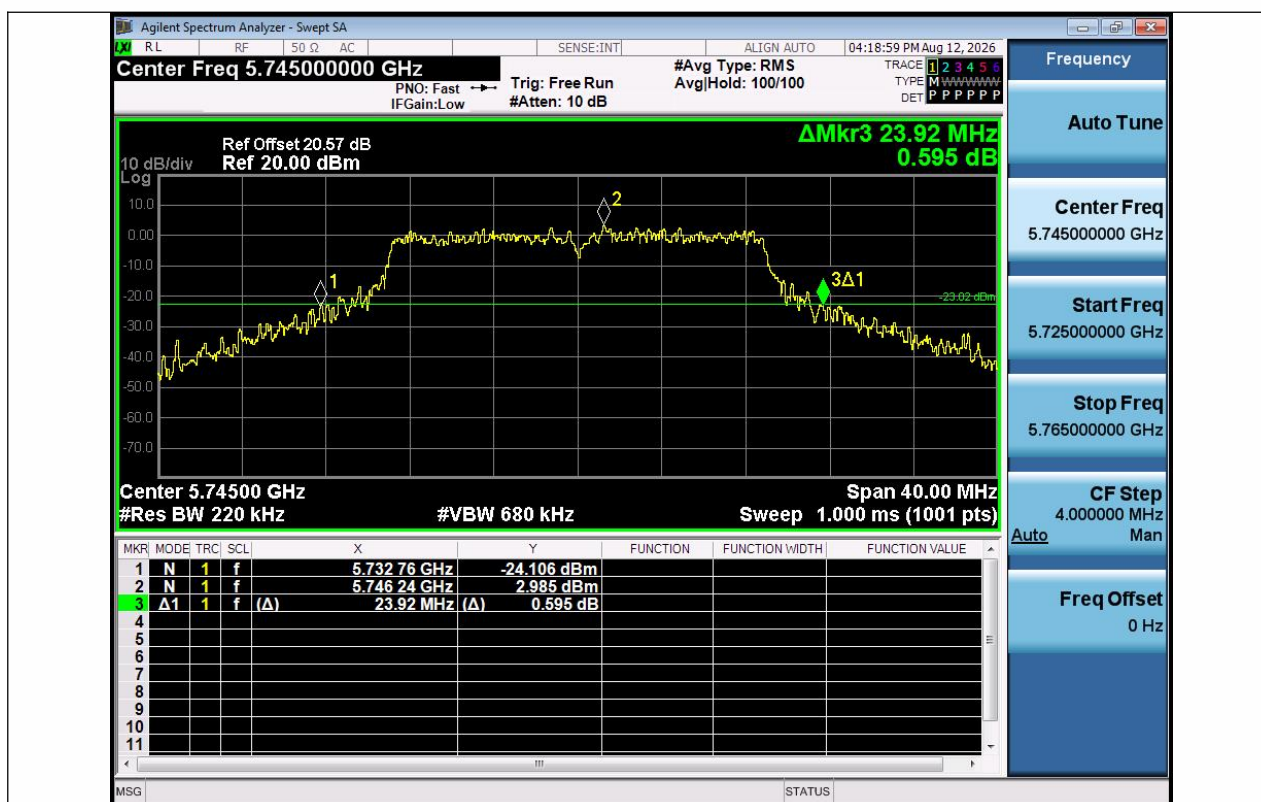
11AC20SISO-Ant1-5745
