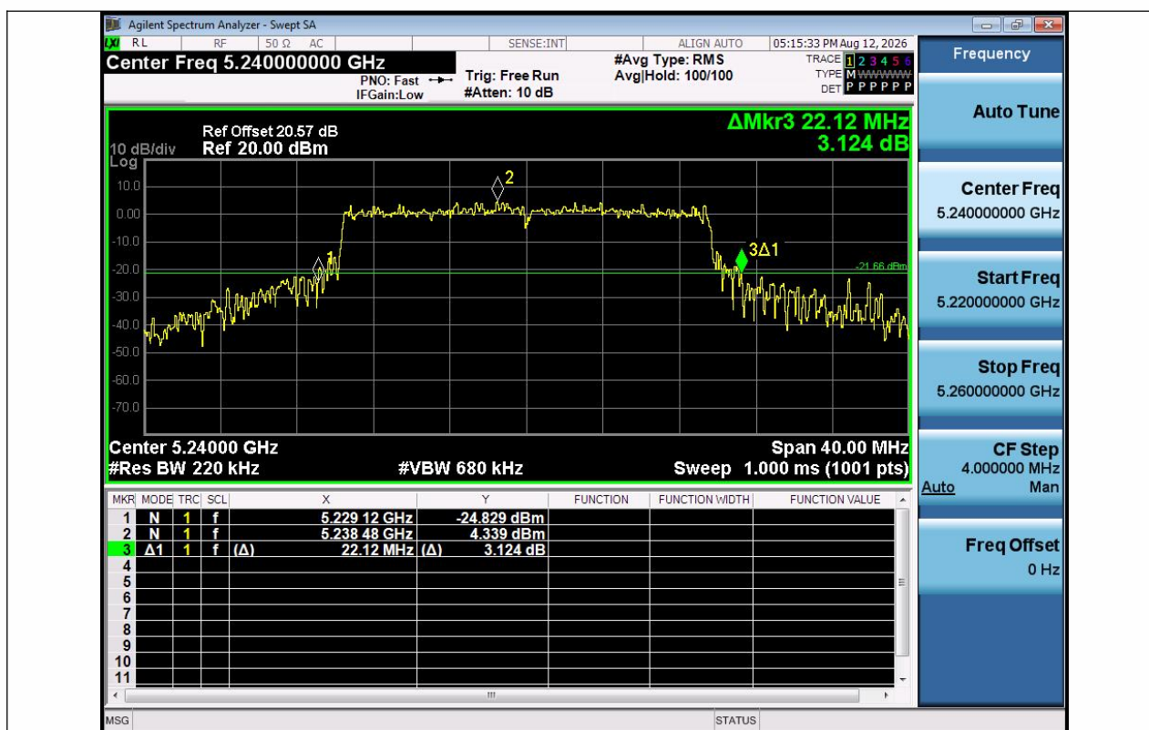
11AX20SISO-Ant1-5240
