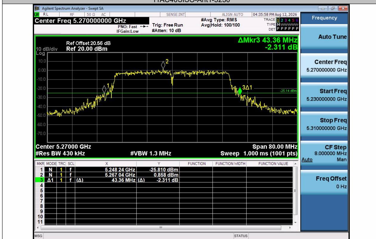
11AC40SISO-Ant1-5270
