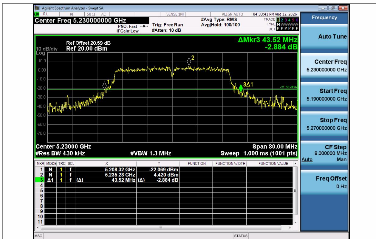
11AC40SISO-Ant1-5230
