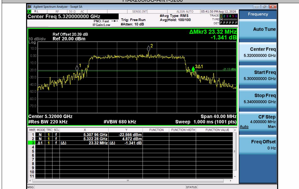
11AX20SISO-Ant1-5320
