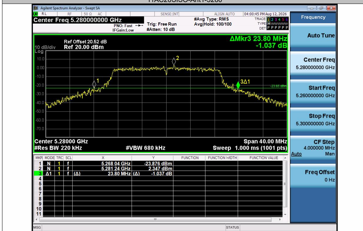
11AC20SISO-Ant1-5280
