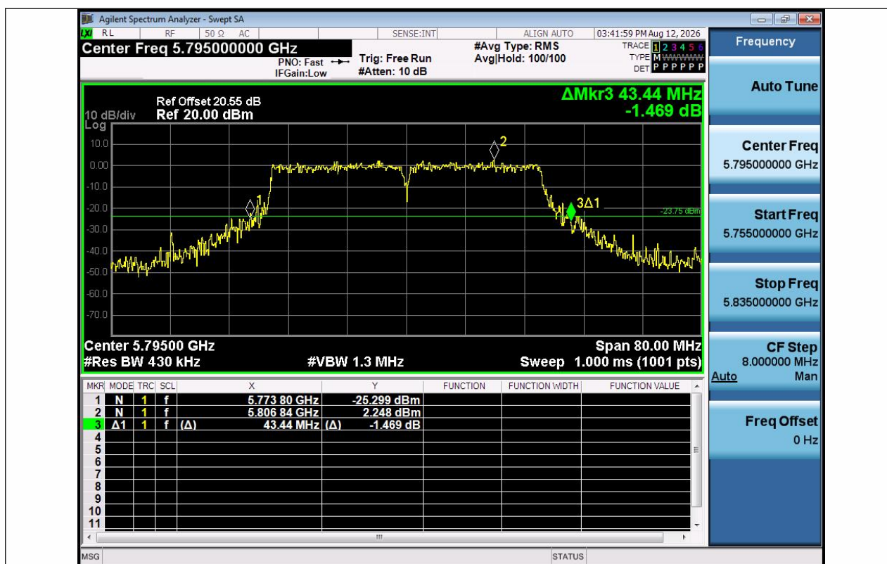
11N40SISO-Ant1-5795
