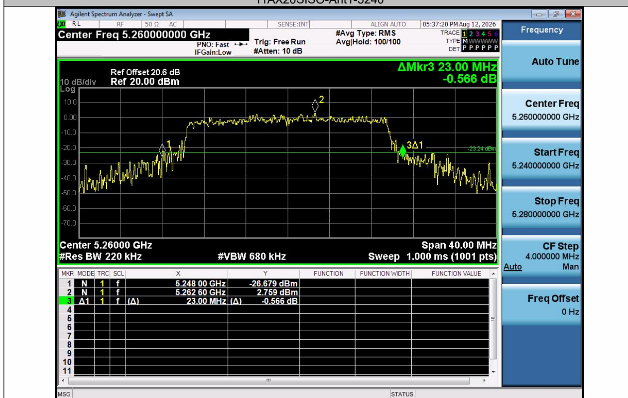
11AX20SISO-Ant1-5260
