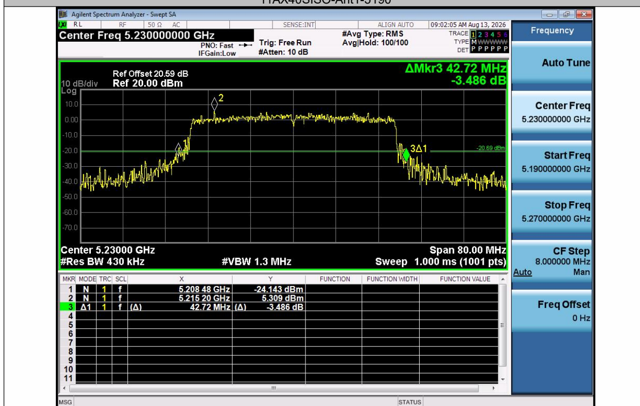
11AX40SISO-Ant1-5230
