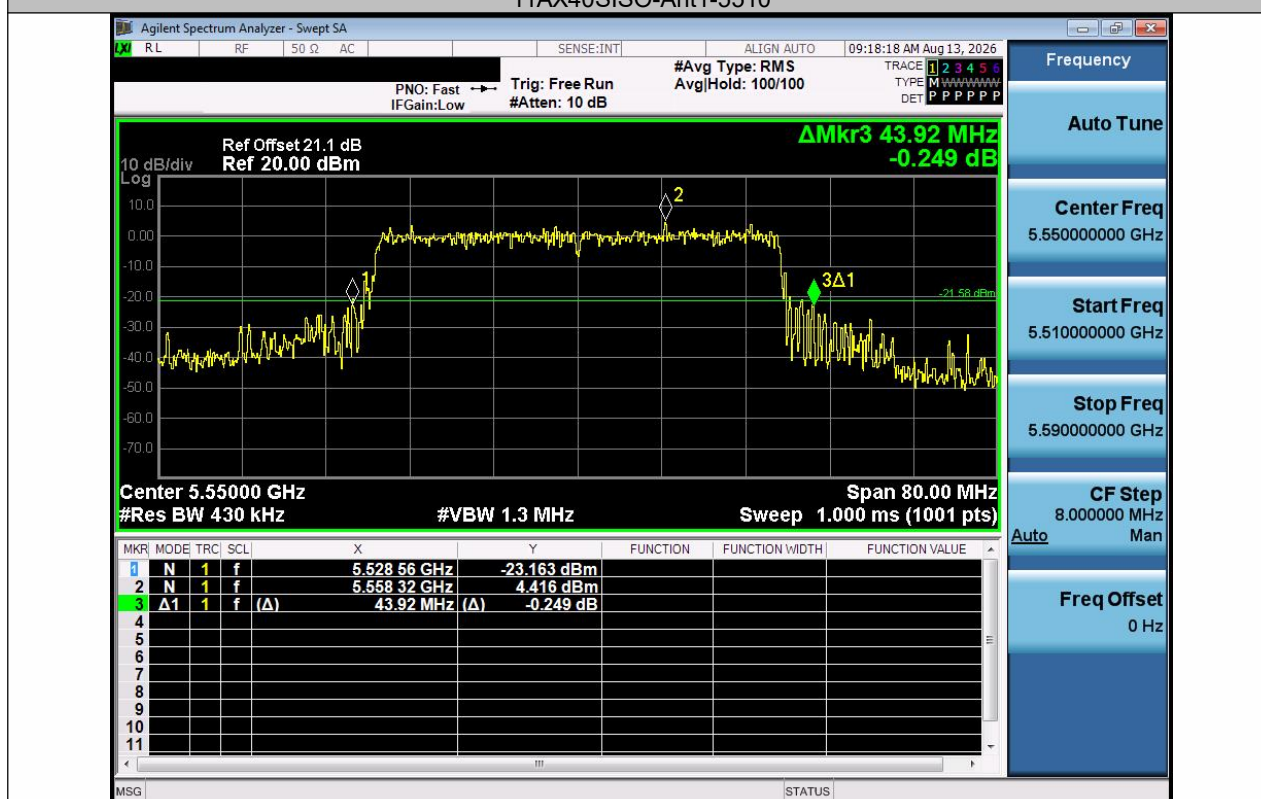
11AX40SISO-Ant1-5550
