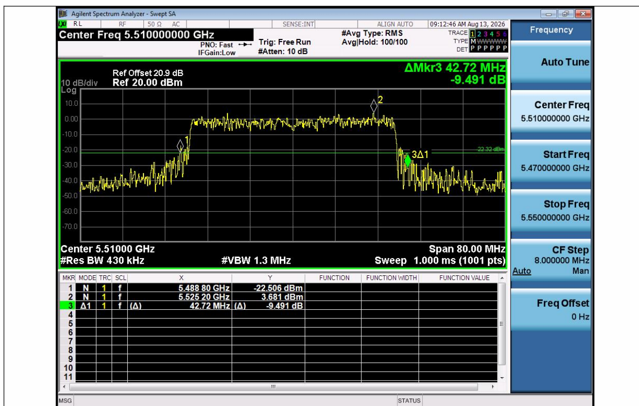
11AX40SISO-Ant1-5510
