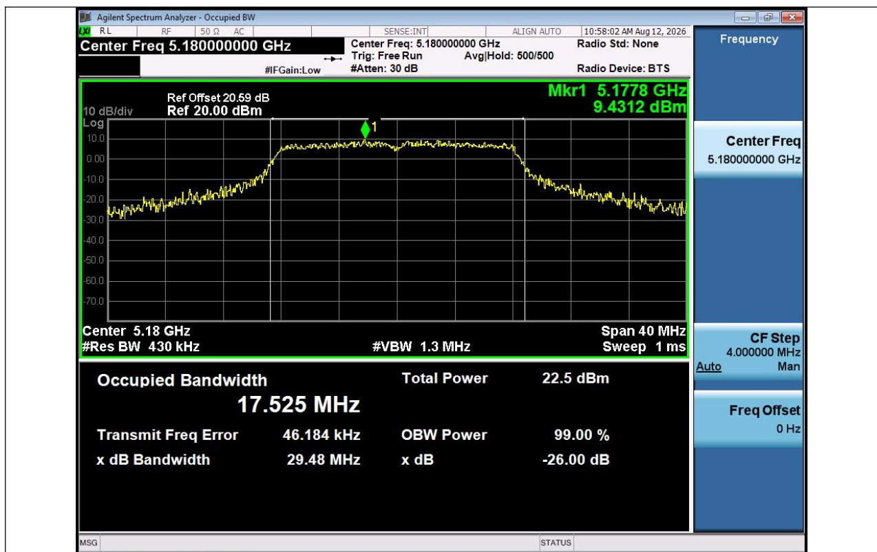
11A-Ant1-5180
