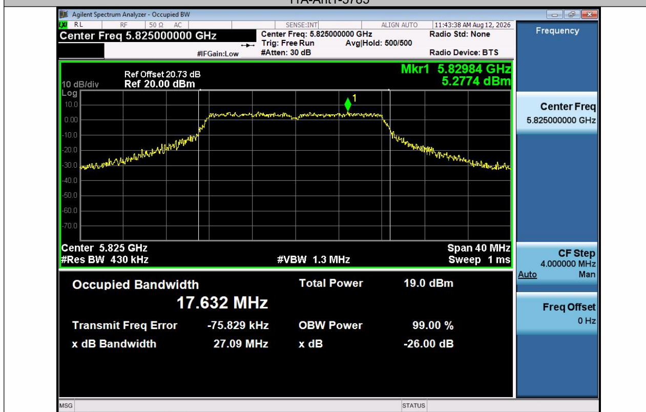
11A-Ant1-5825
