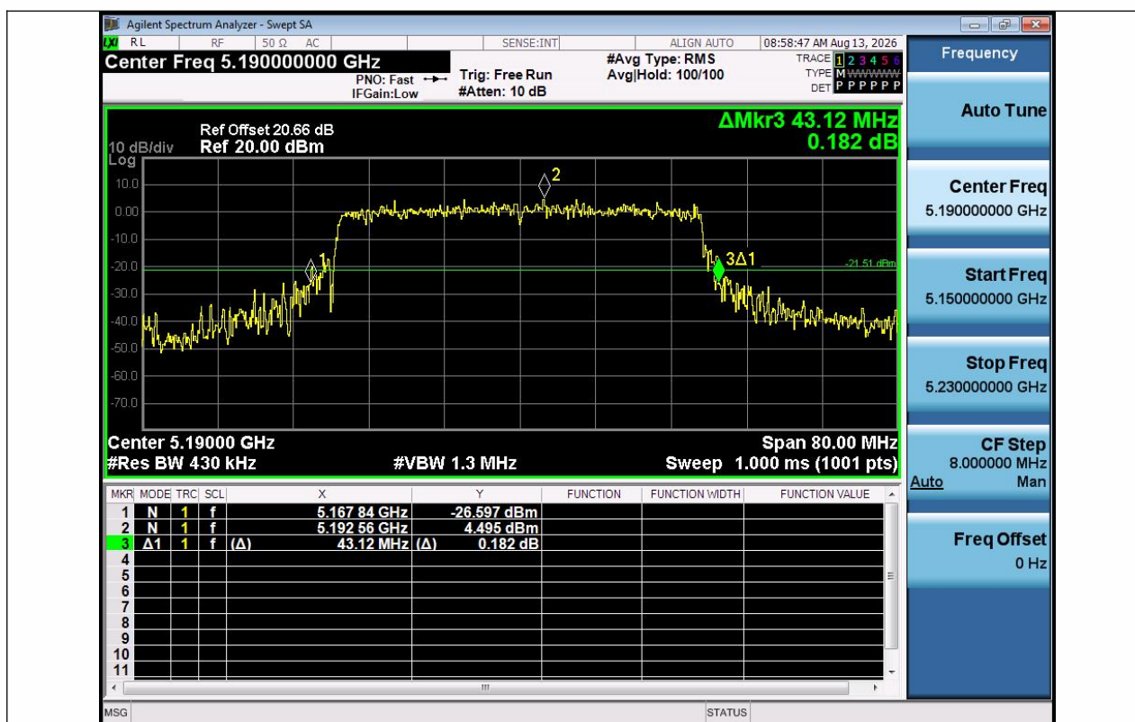
11AX40SISO-Ant1-5190
