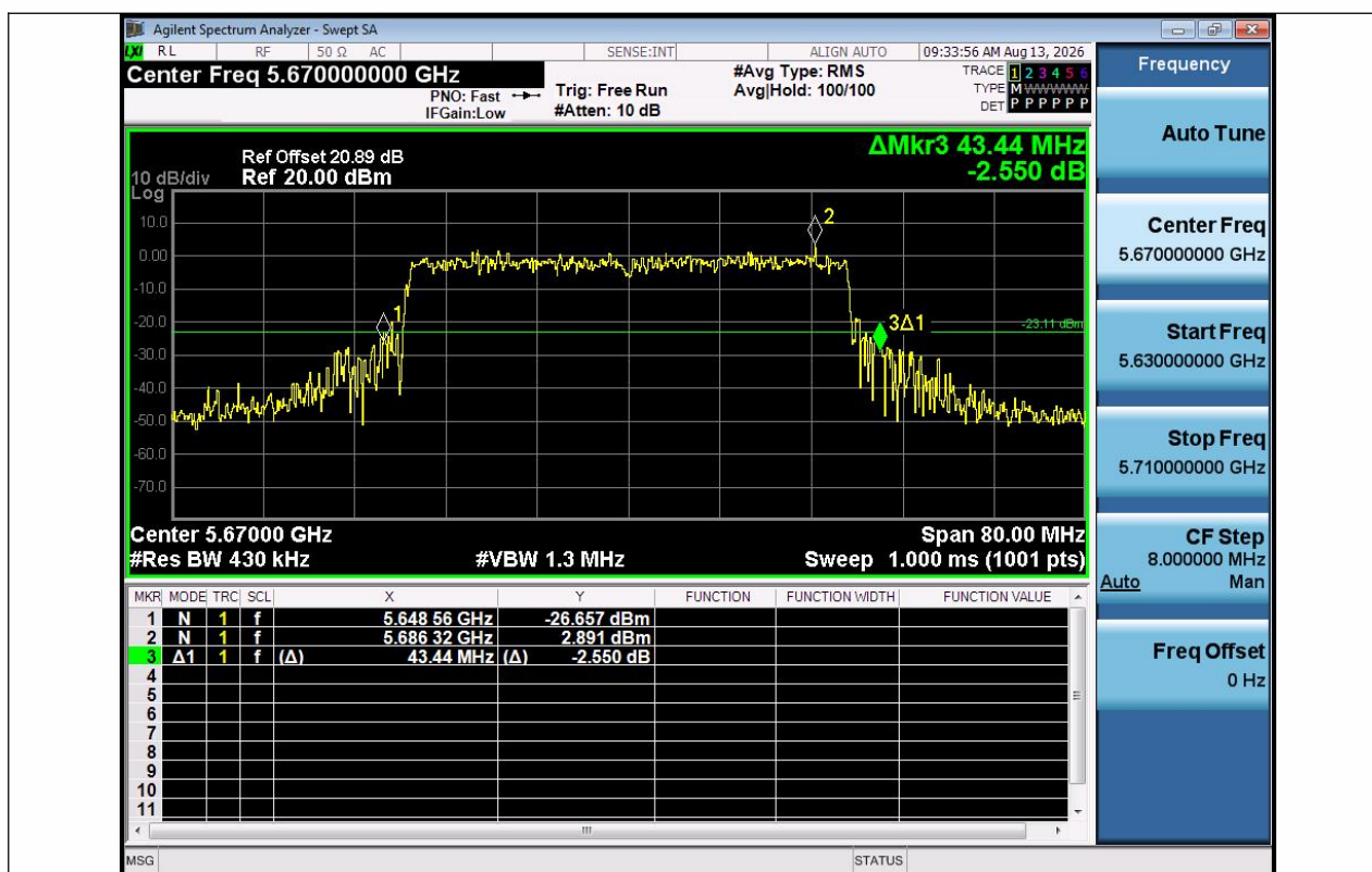
11AX40SISO-Ant1-5670
