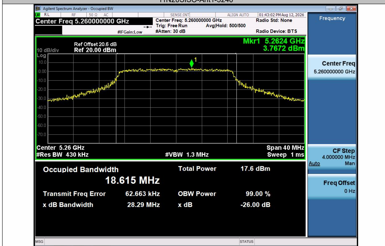
11N20SISO-Ant1-5260
