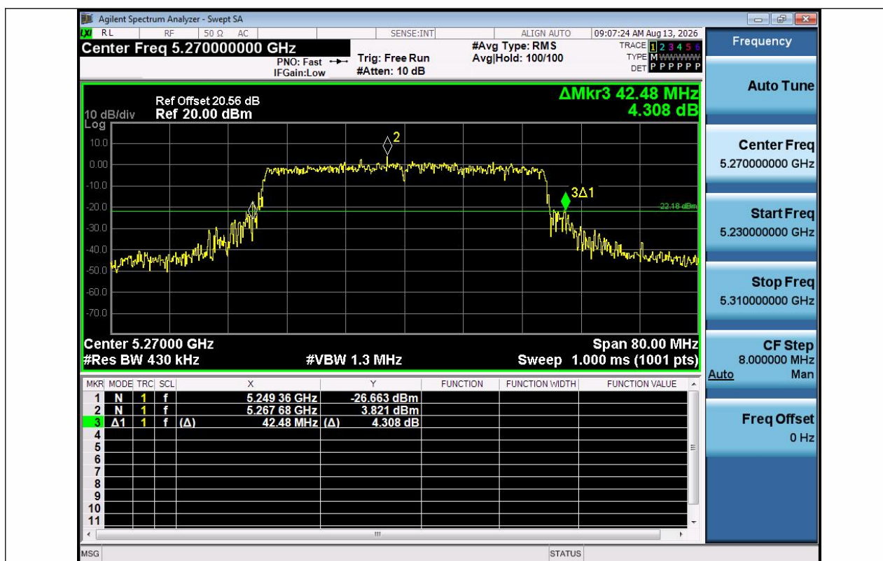
11AX40SISO-Ant1-5270
