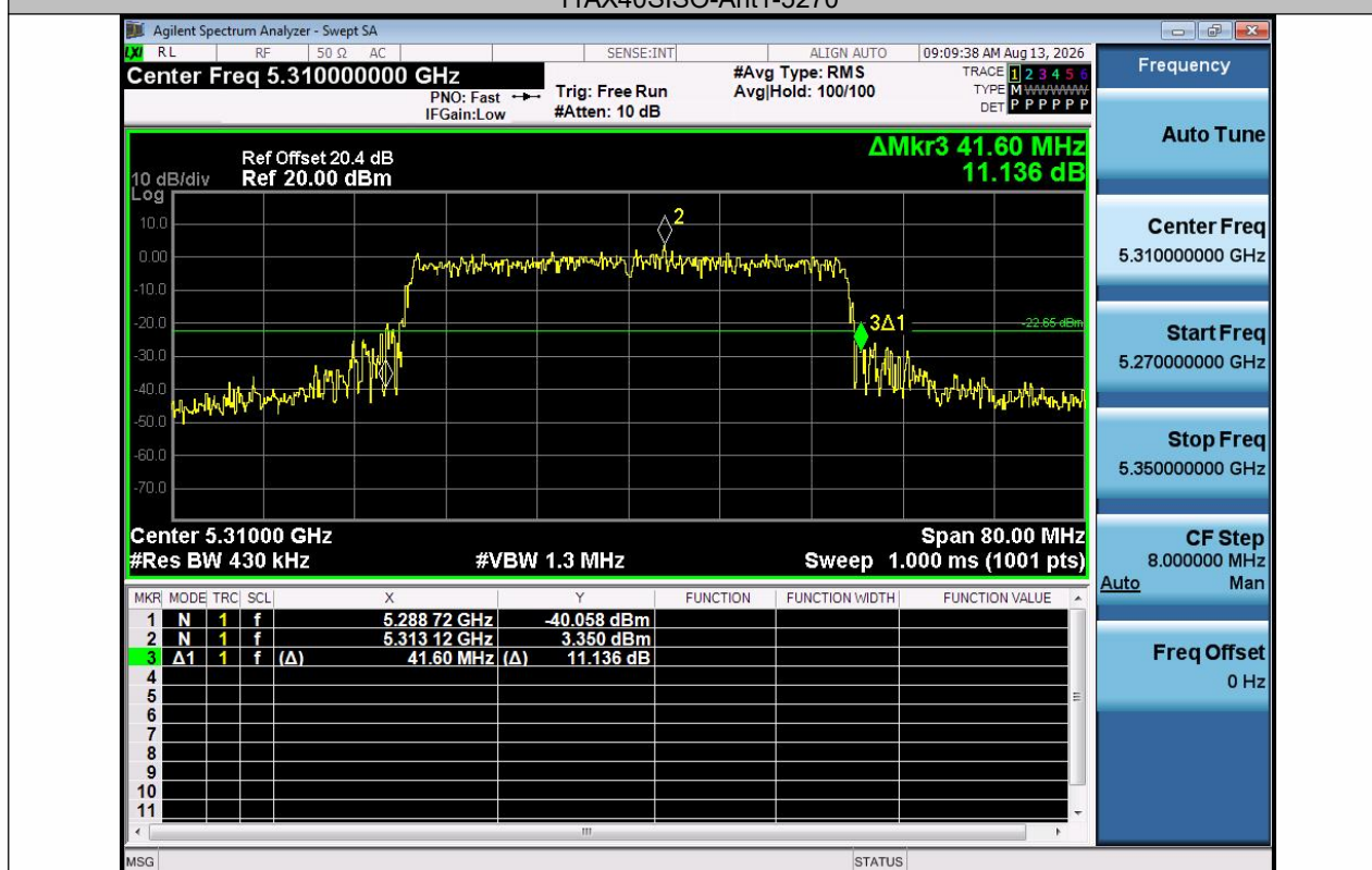
11AX40SISO-Ant1-5310
