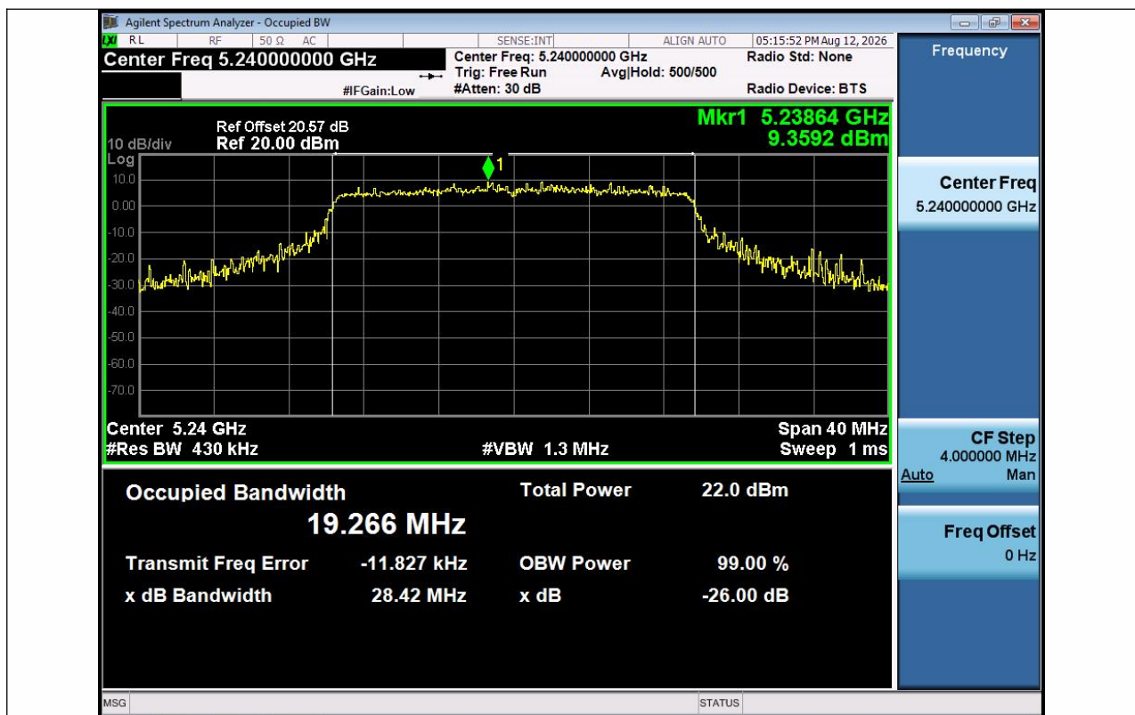
11AX20SISO-Ant1-5240
