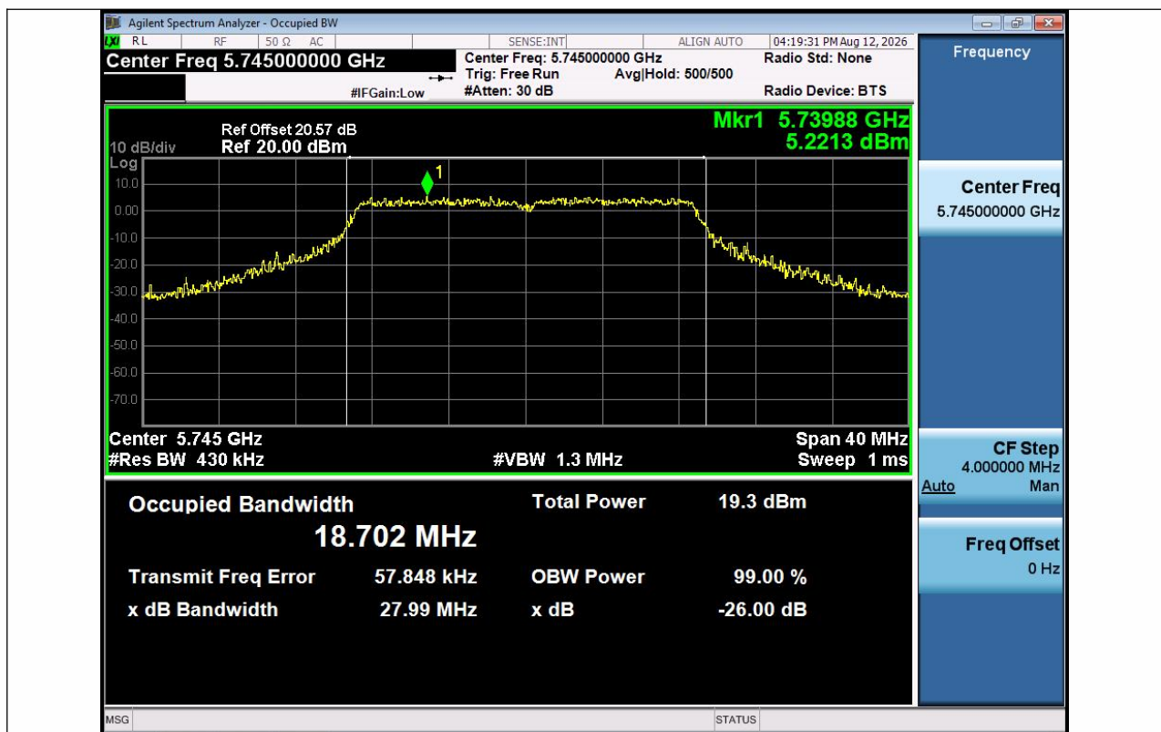
11AC20SISO-Ant1-5745
