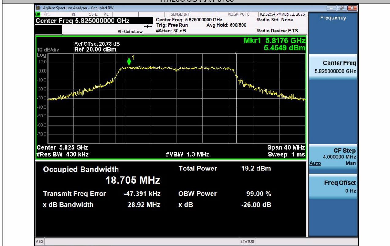
11N20SISO-Ant1-5825
