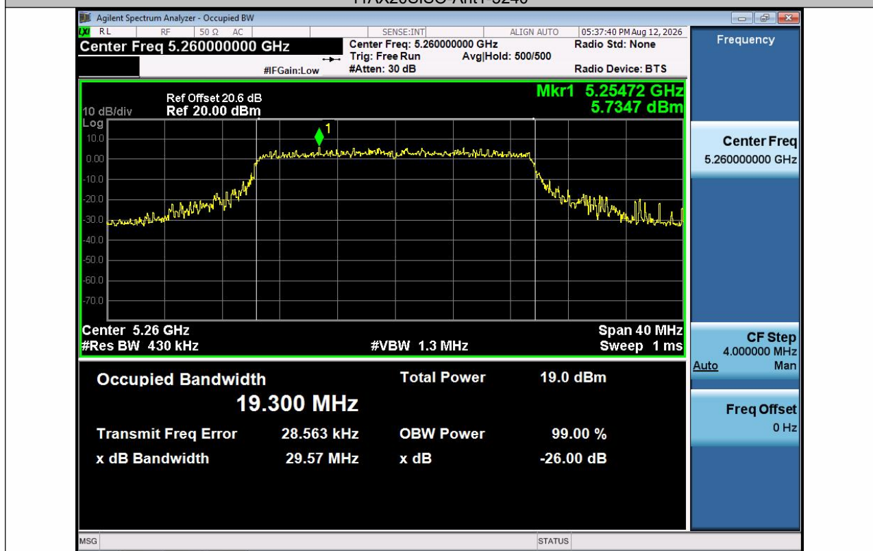
11AX20SISO-Ant1-5260
