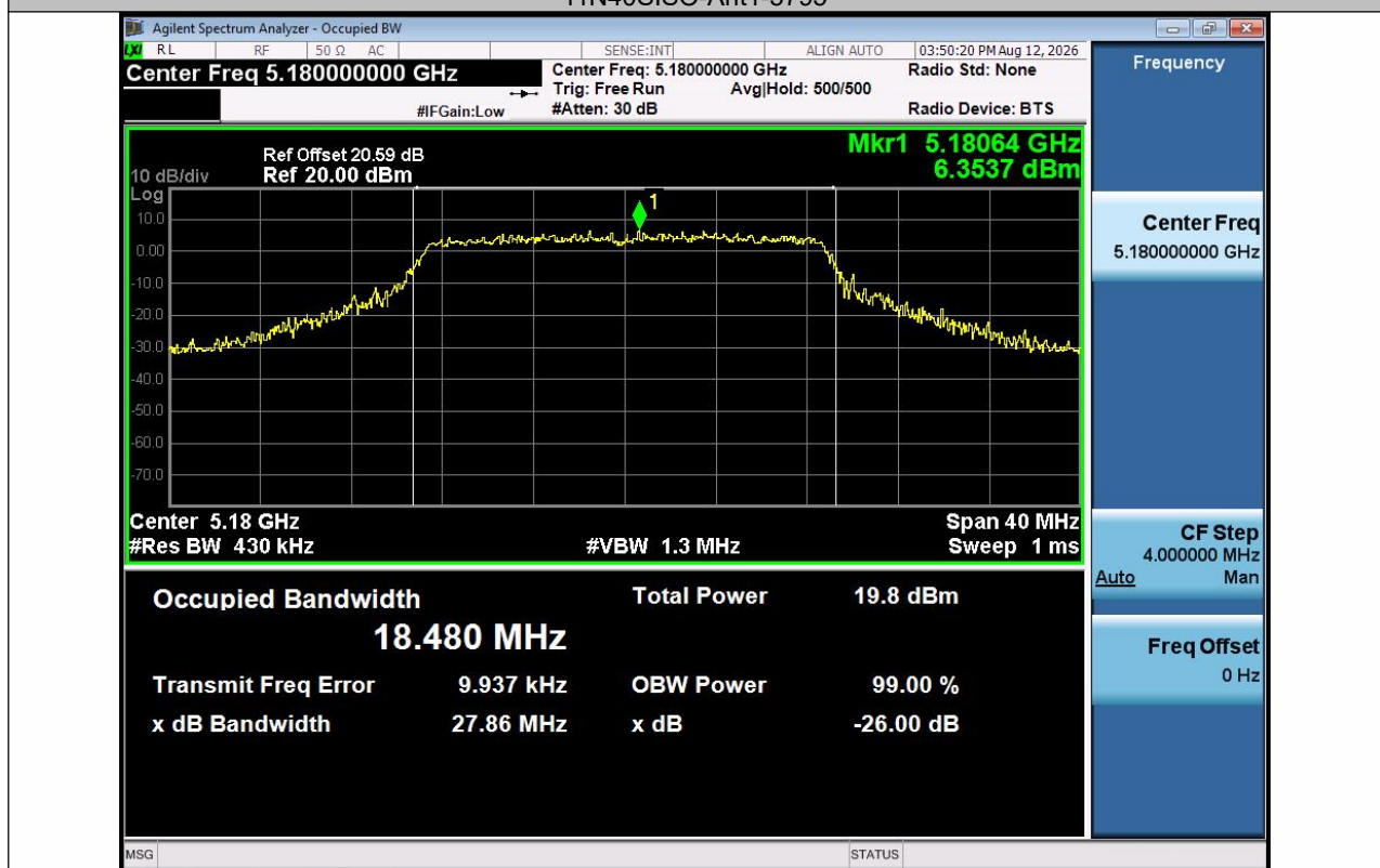
11AC20SISO-Ant1-5180
