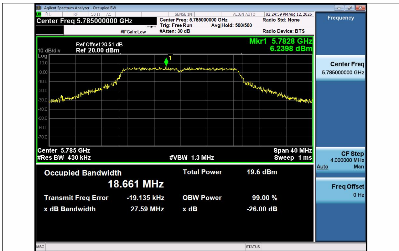
11N20SISO-Ant1-5785
