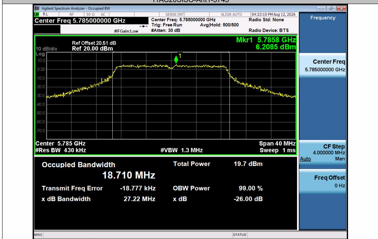
11AC20SISO-Ant1-5785
