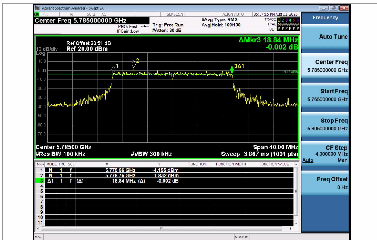
11AX20SISO-Ant1-5785-PASS
