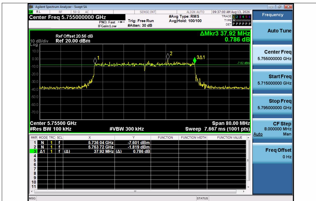
11AX40SISO-Ant1-5755-PASS
