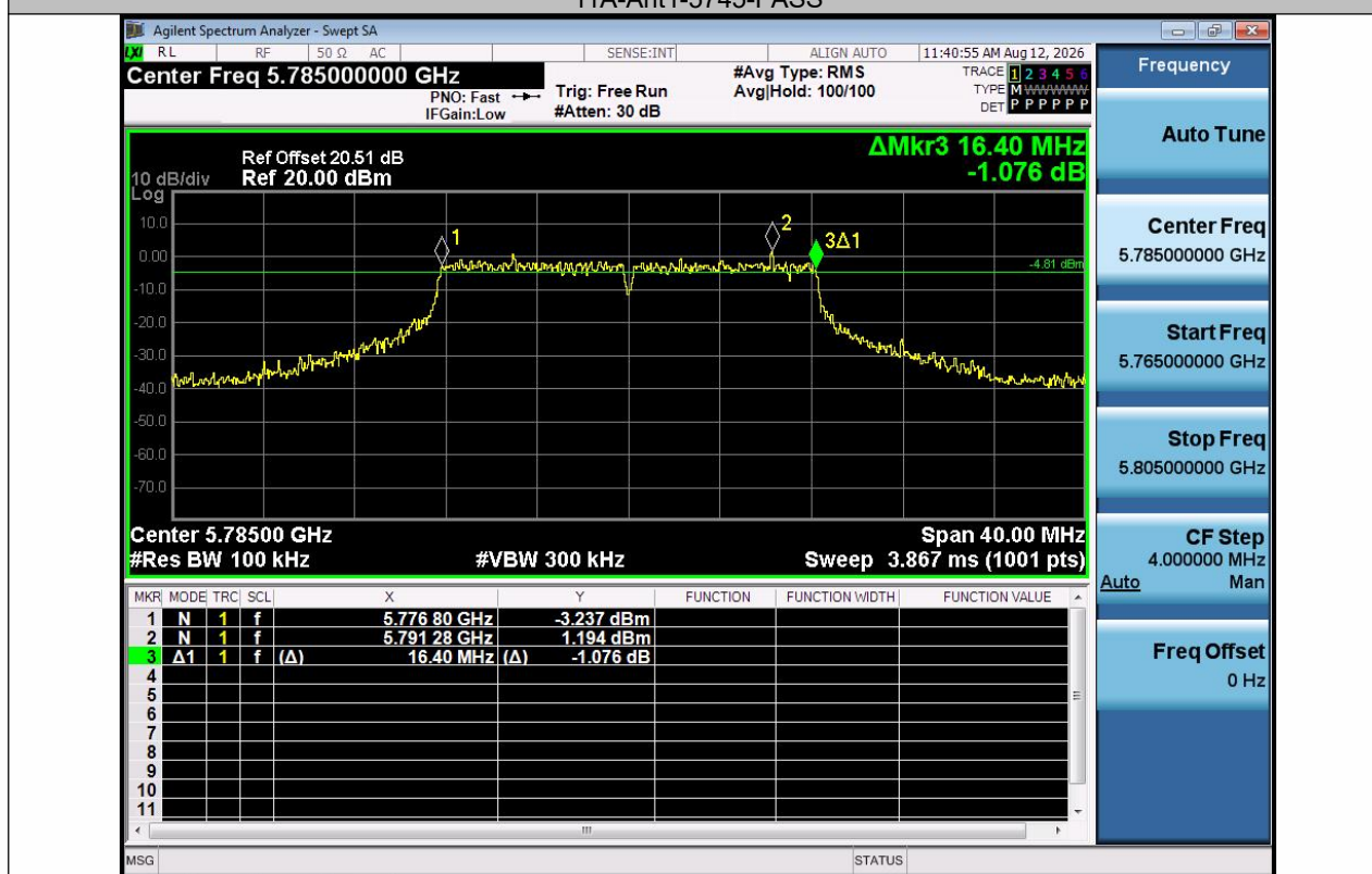
11A-Ant1-5785-PASS
