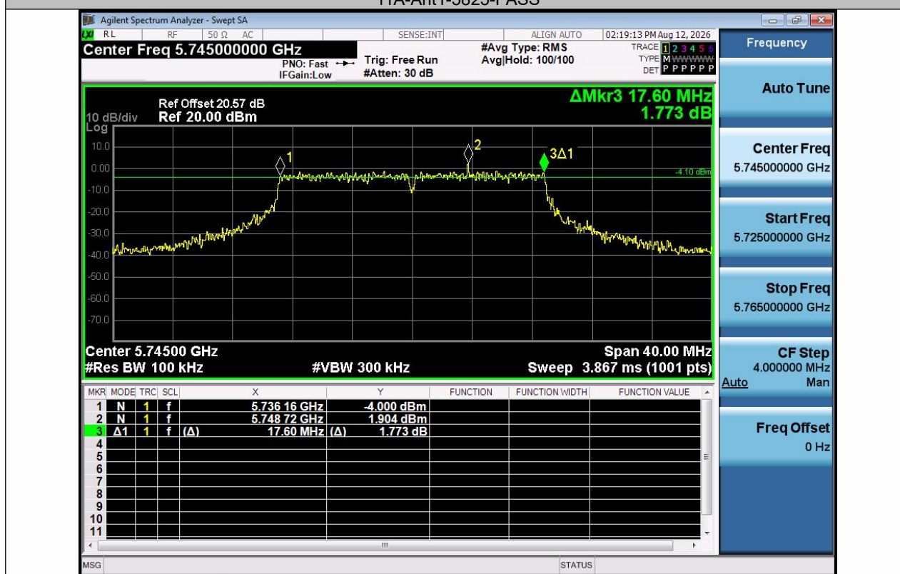
11N20SiSO-Ant1-5745-PASS
