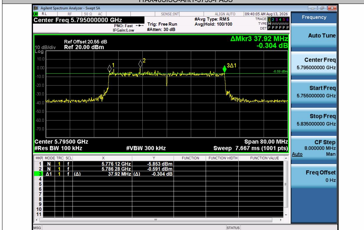
11AX40SISO-Ant1-5795-PASS
