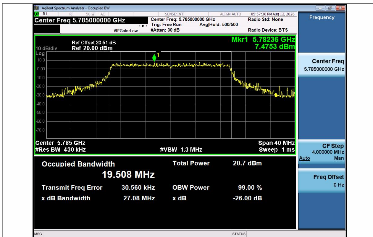
11AX20SISO-Ant1-5785
