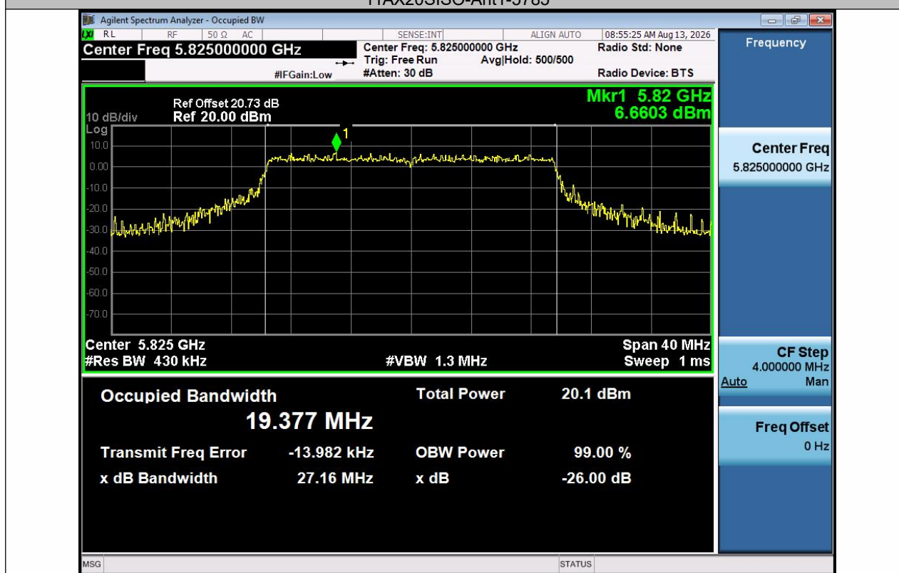
11AX20SISO-Ant1-5825
