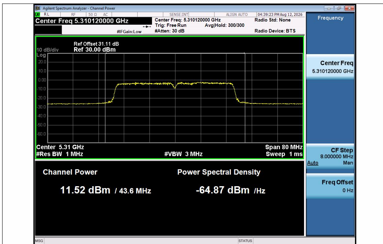
11AC40SISO-Ant1-5310-PASS
