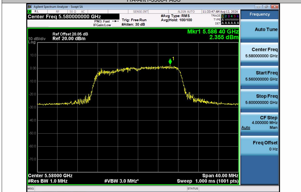
11A-Ant1-5580-PASS
