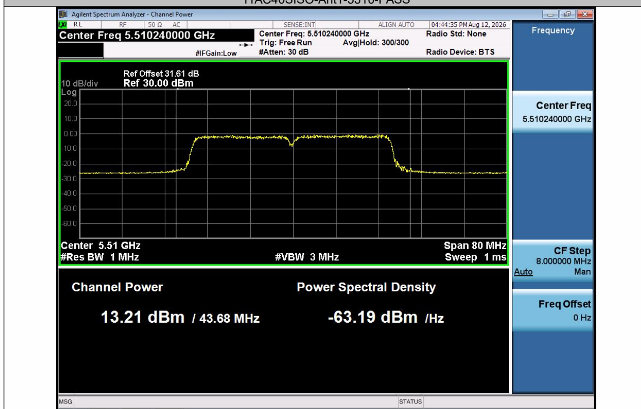
11AC40SISO-Ant1-5510-PASS
