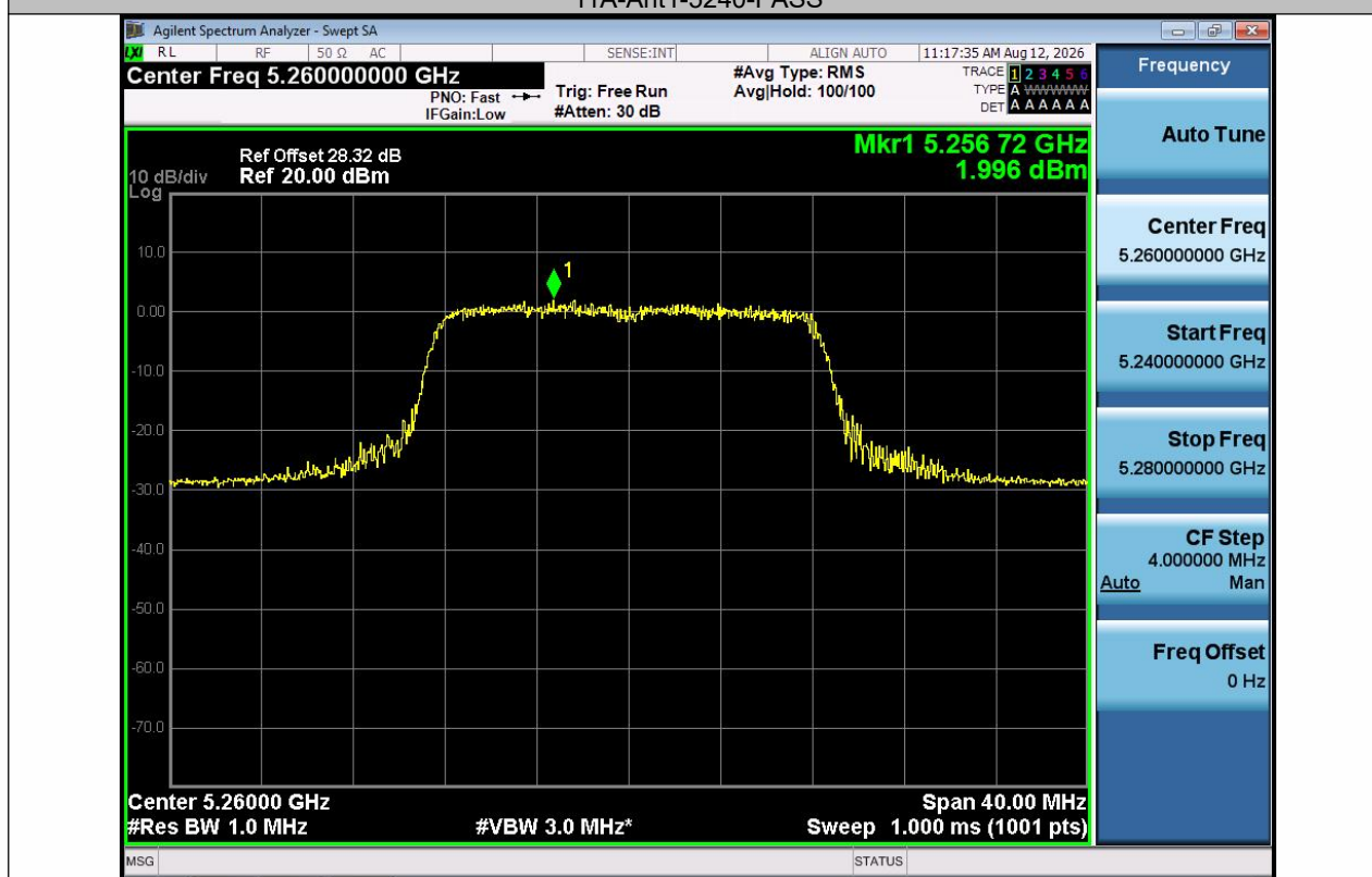
11A-Ant1-5260-PASS
