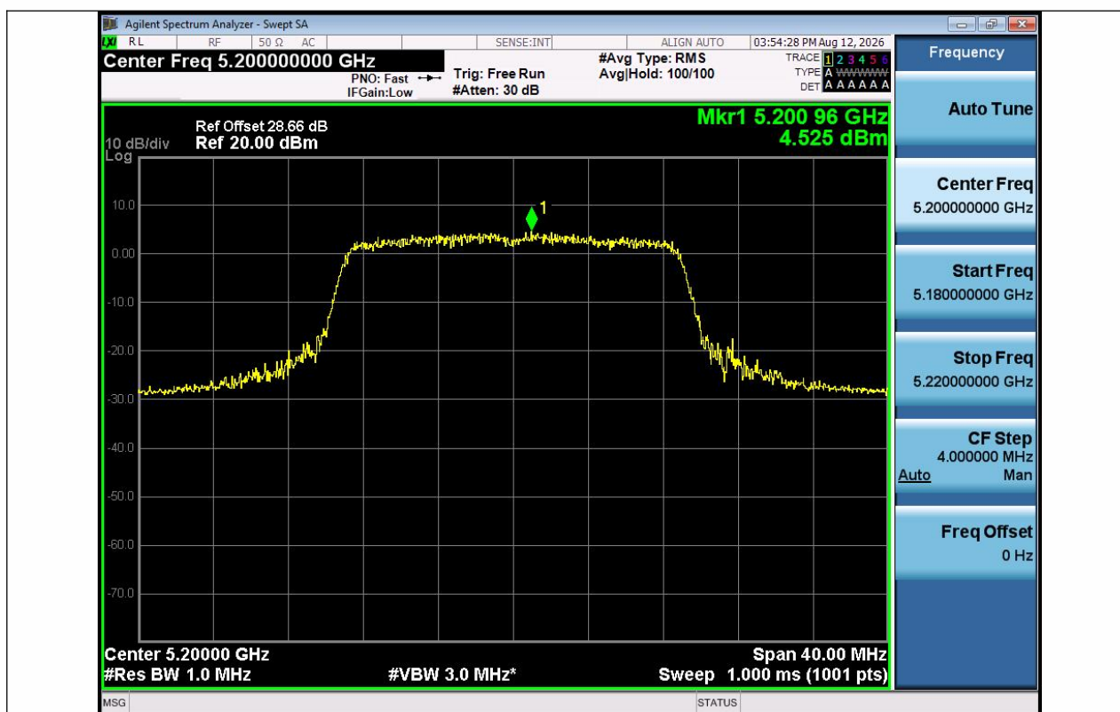
11AC20SISO-Ant1-5200-PASS
