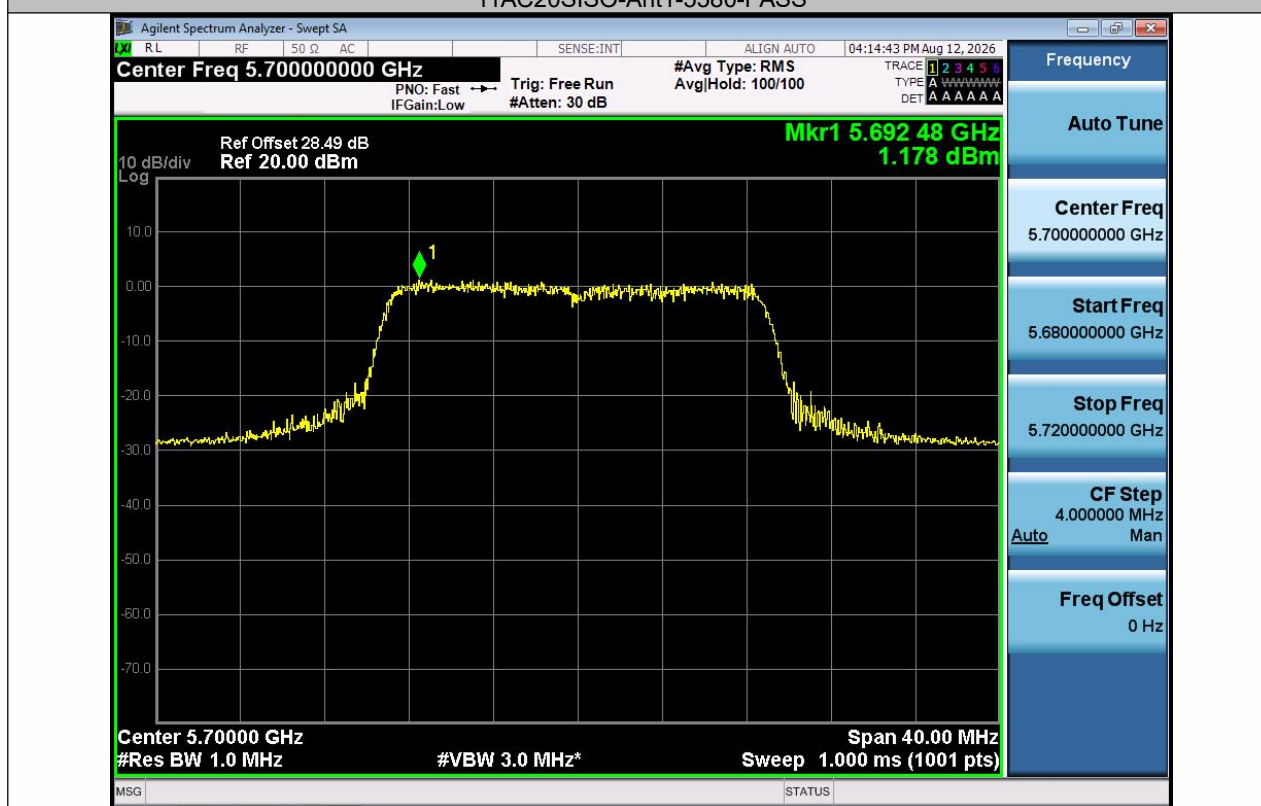
11AC20SISO-Ant1-5700-PASS
