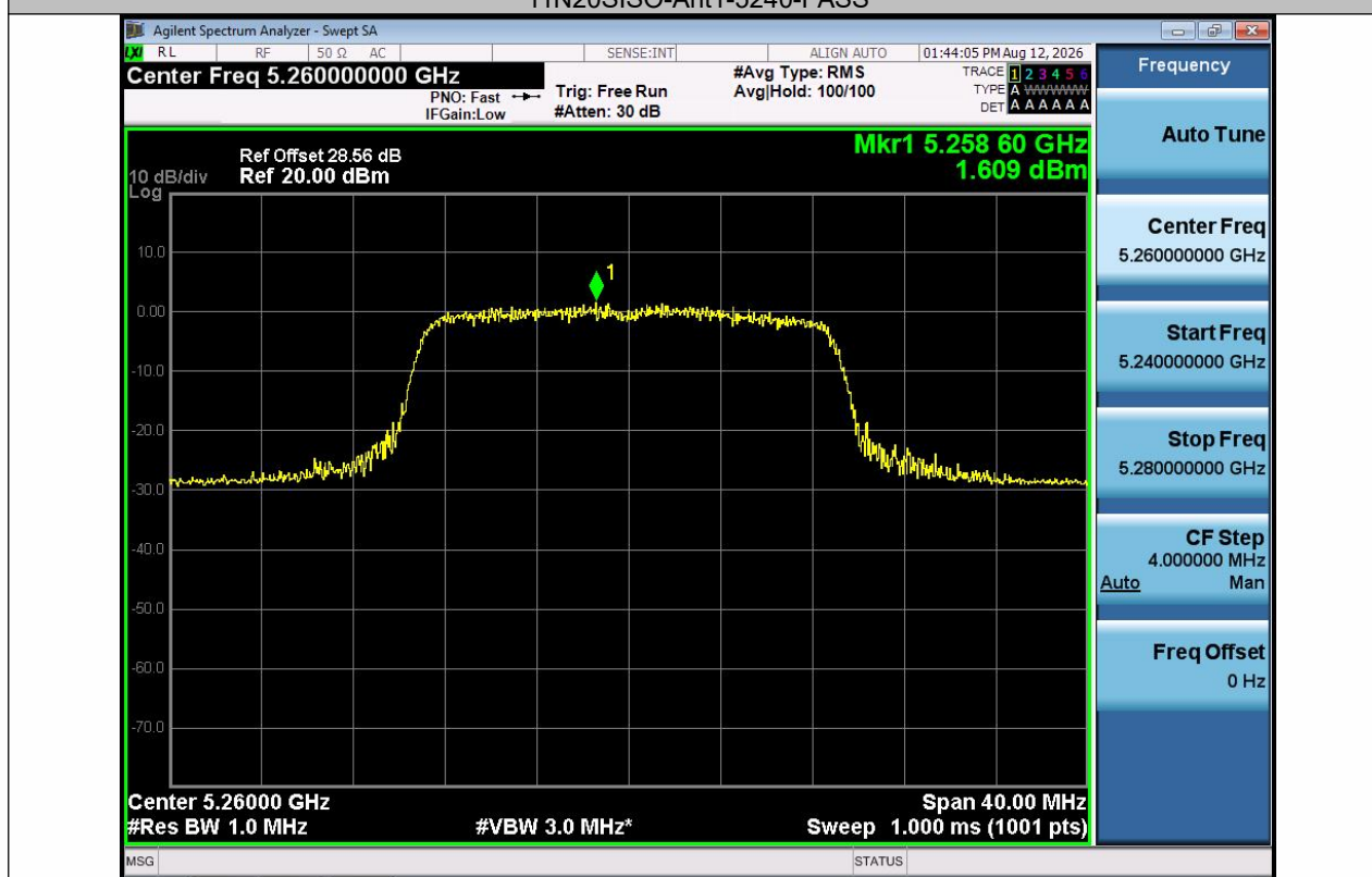
11N20SISO-Ant1-5260-PASS
