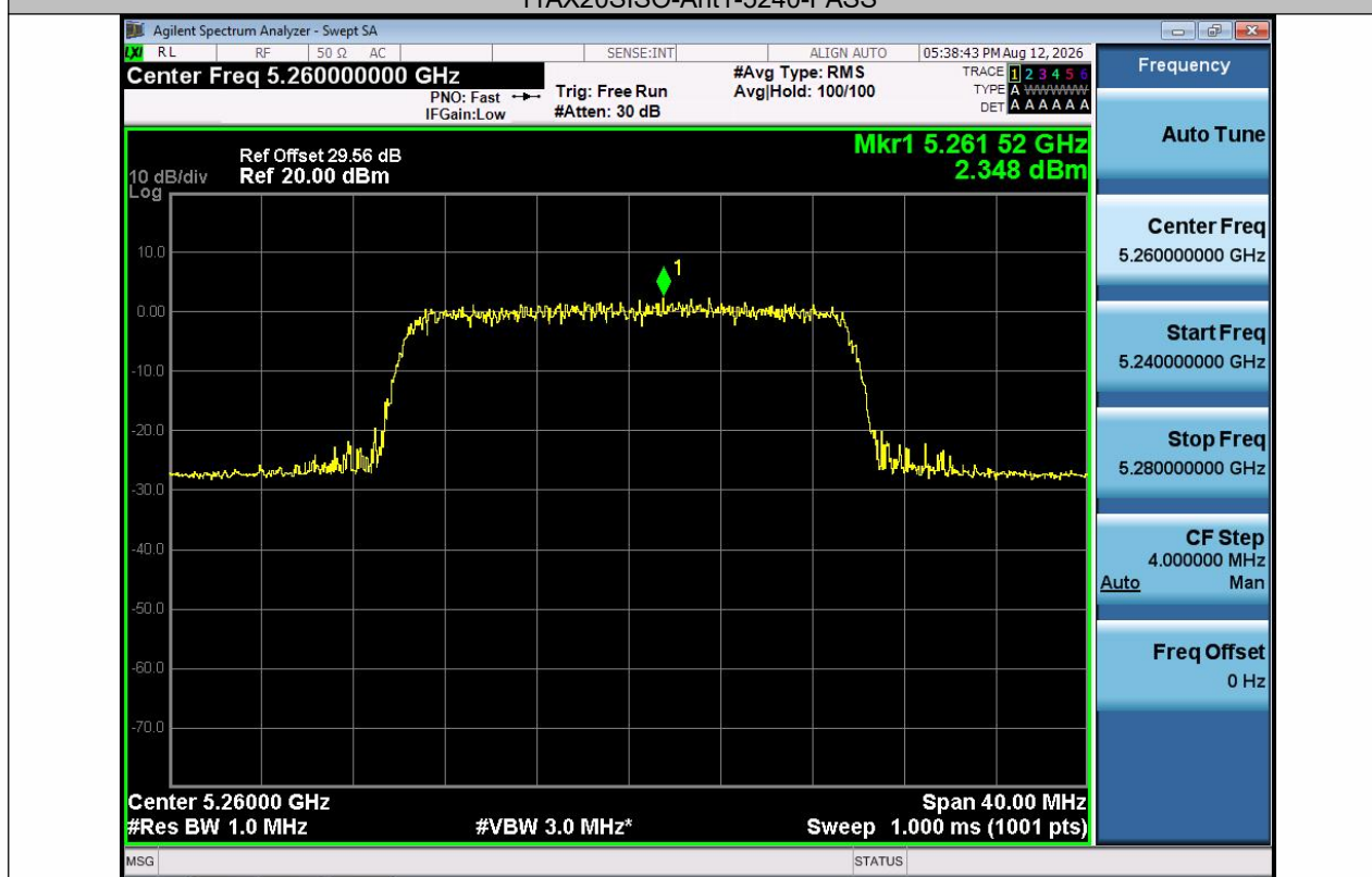
11AX20SISO-Ant1-5260-PASS
