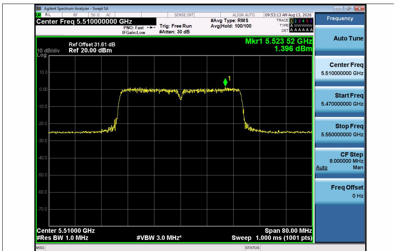
11N40SISO-Ant1-5510-PASS
