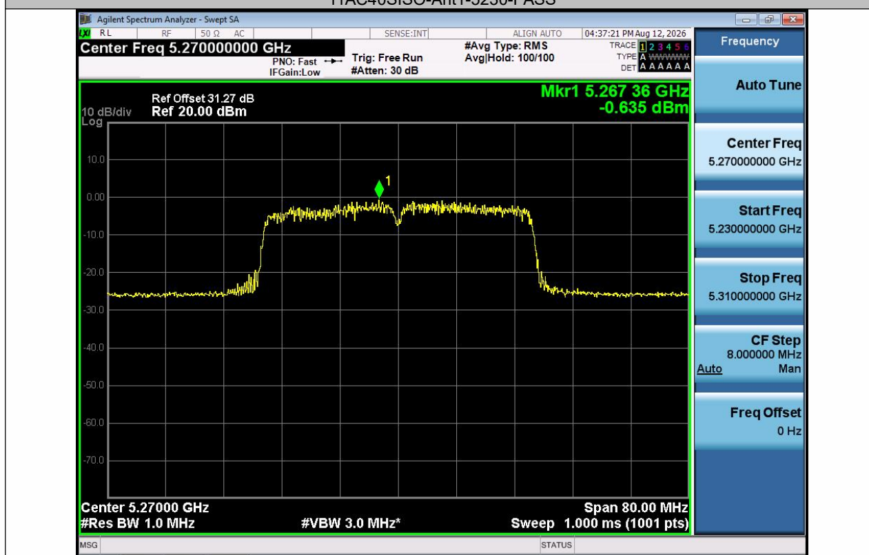
11AC40SISO-Ant1-5270-PASS
