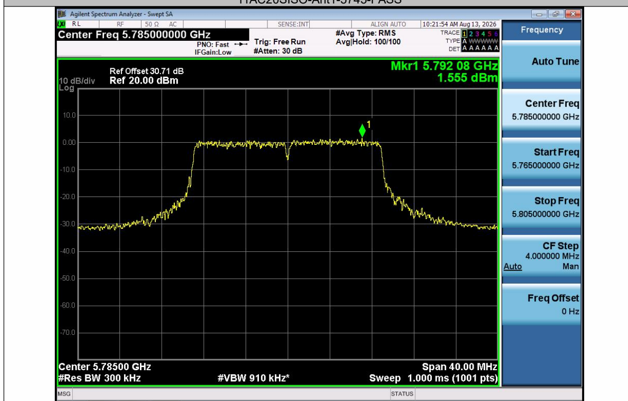
11AC20SISO-Ant1-5785-PASS
