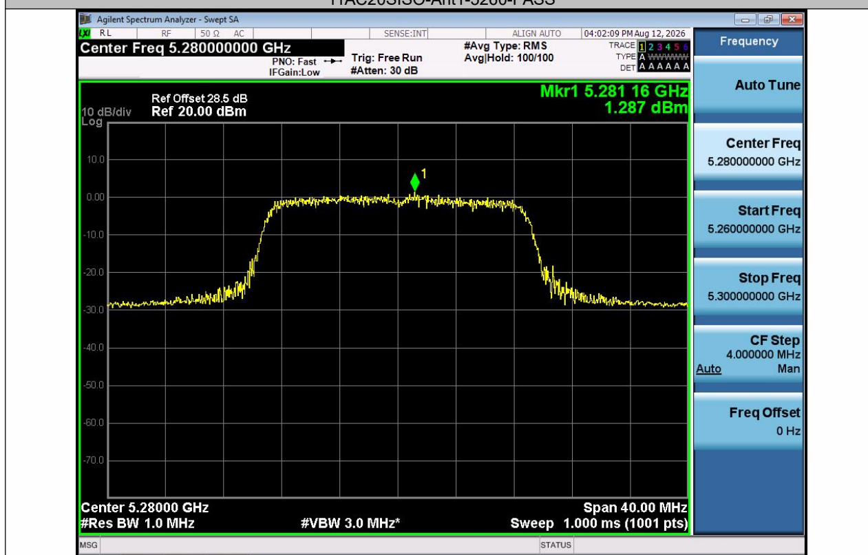
11AC20SISO-Ant1-5280-PASS
