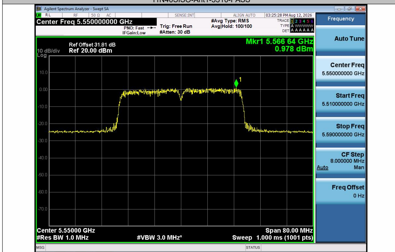
11N40SISO-Ant1-5550-PASS
