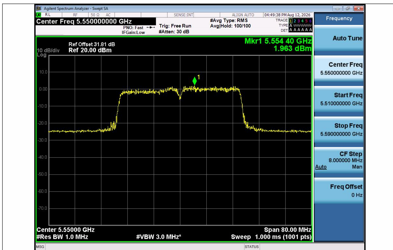
11AC40SISO-Ant1-5550-PASS
