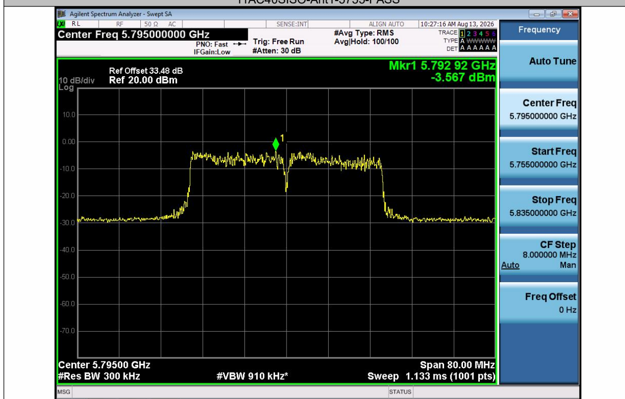
11AC40SISO-Ant1-5795-PASS
