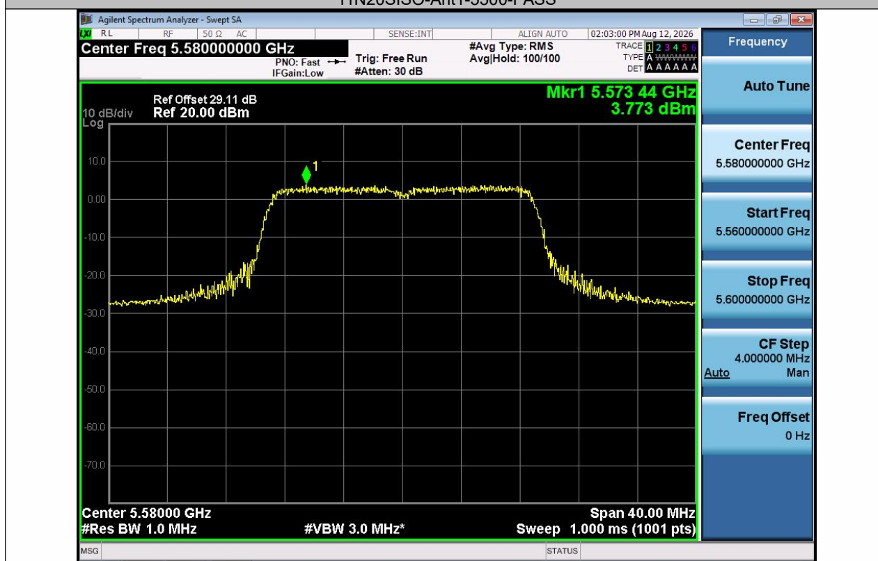
11N20SISO-Ant1-5580-PASS
