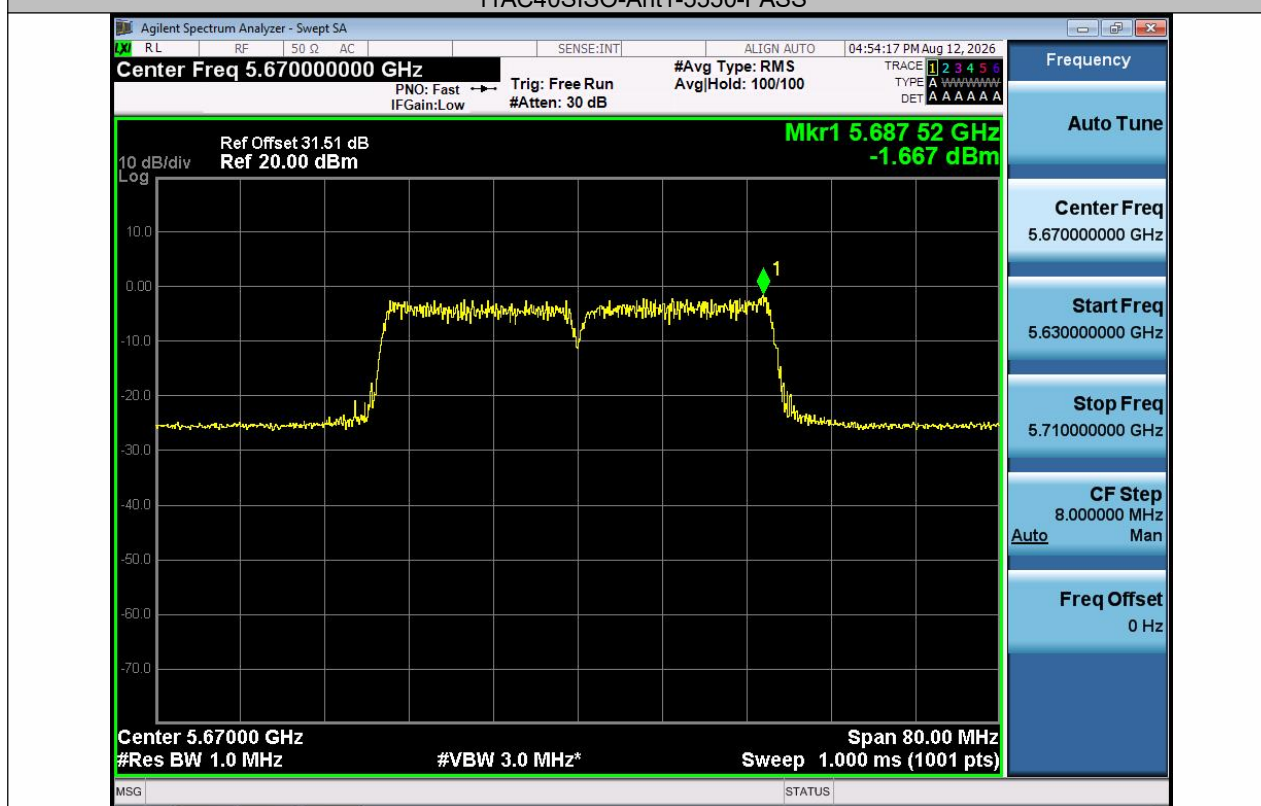
11AC40SISO-Ant1-5670-PASS
