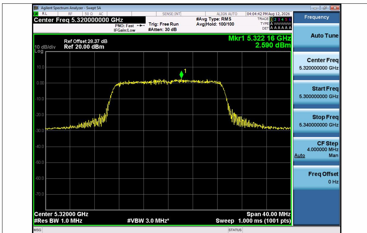
11AC20SISO-Ant1-5320-PASS
