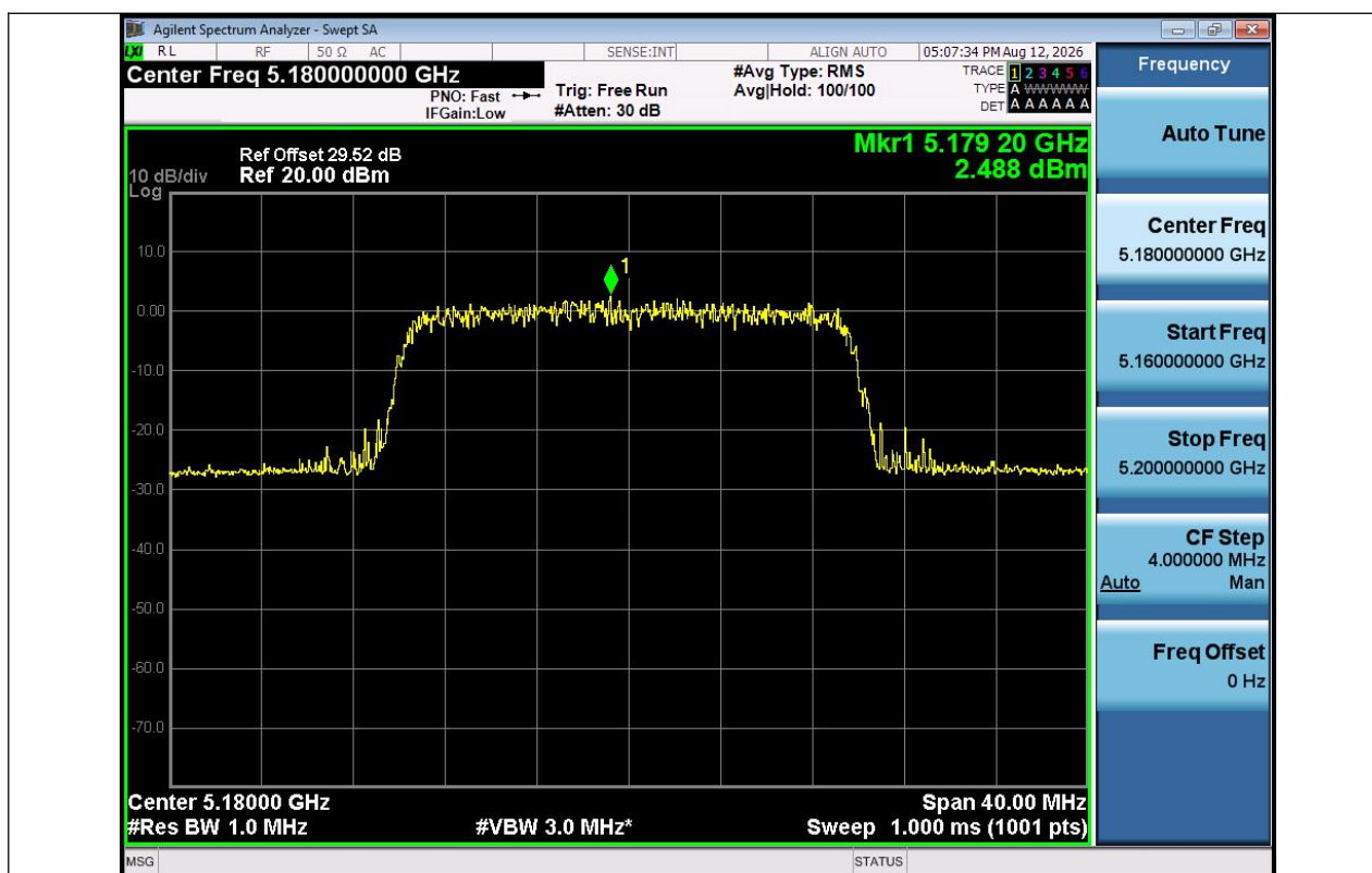
11AX20SISO-Ant1-5180-PASS
