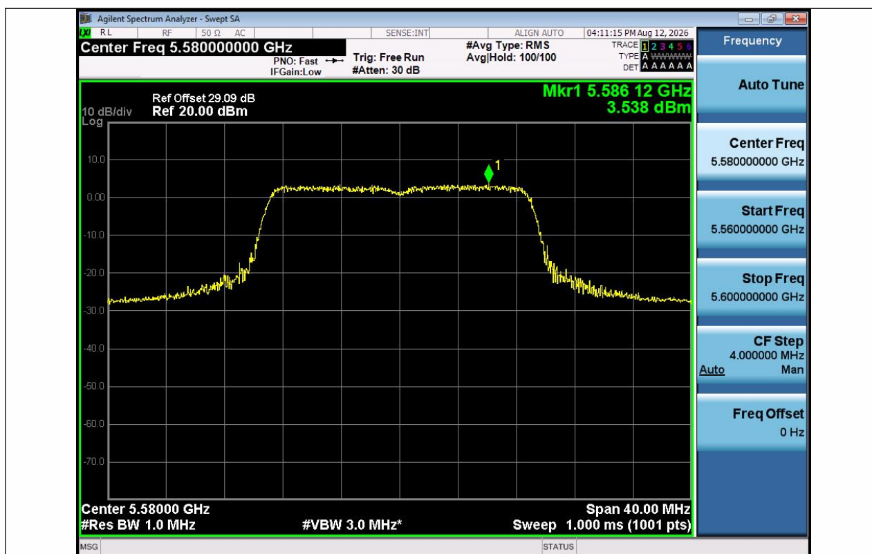
11AC20SISO-Ant1-5580-PASS
