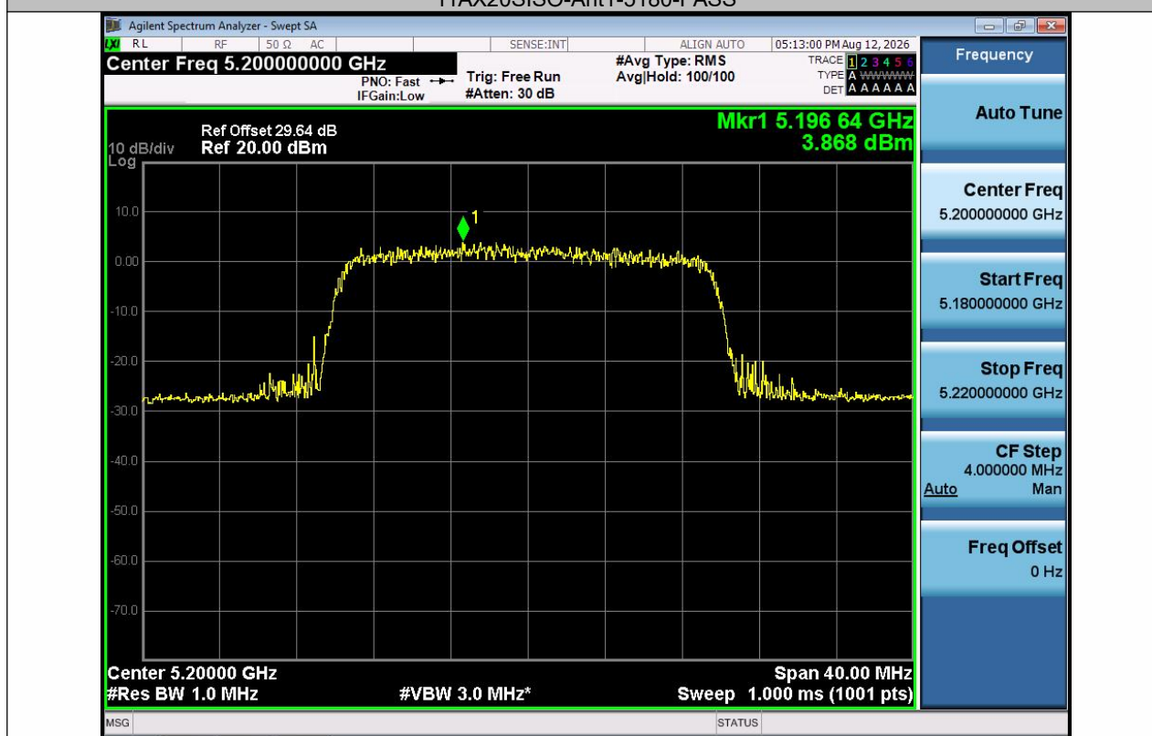
11AX20SISO-Ant1-5200-PASS
