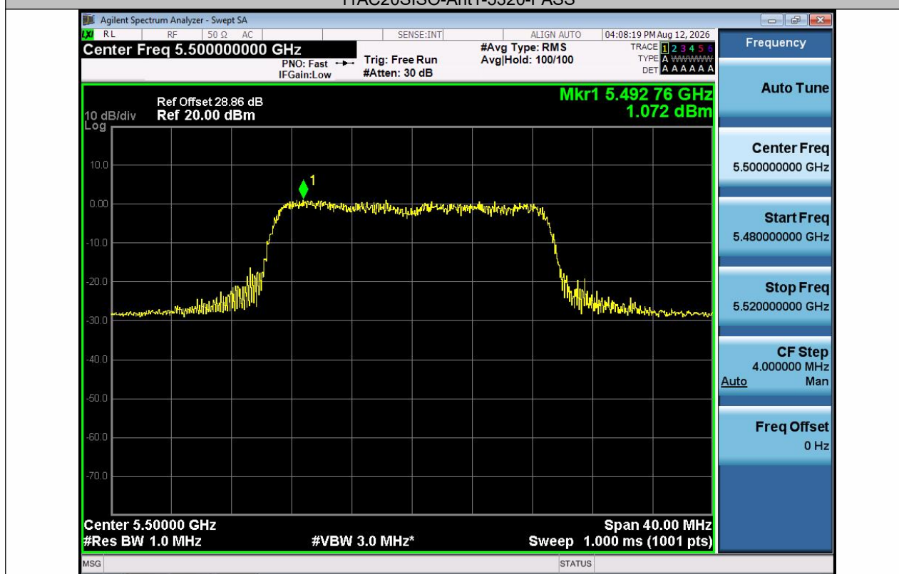
11AC20SISO-Ant1-5500-PASS
