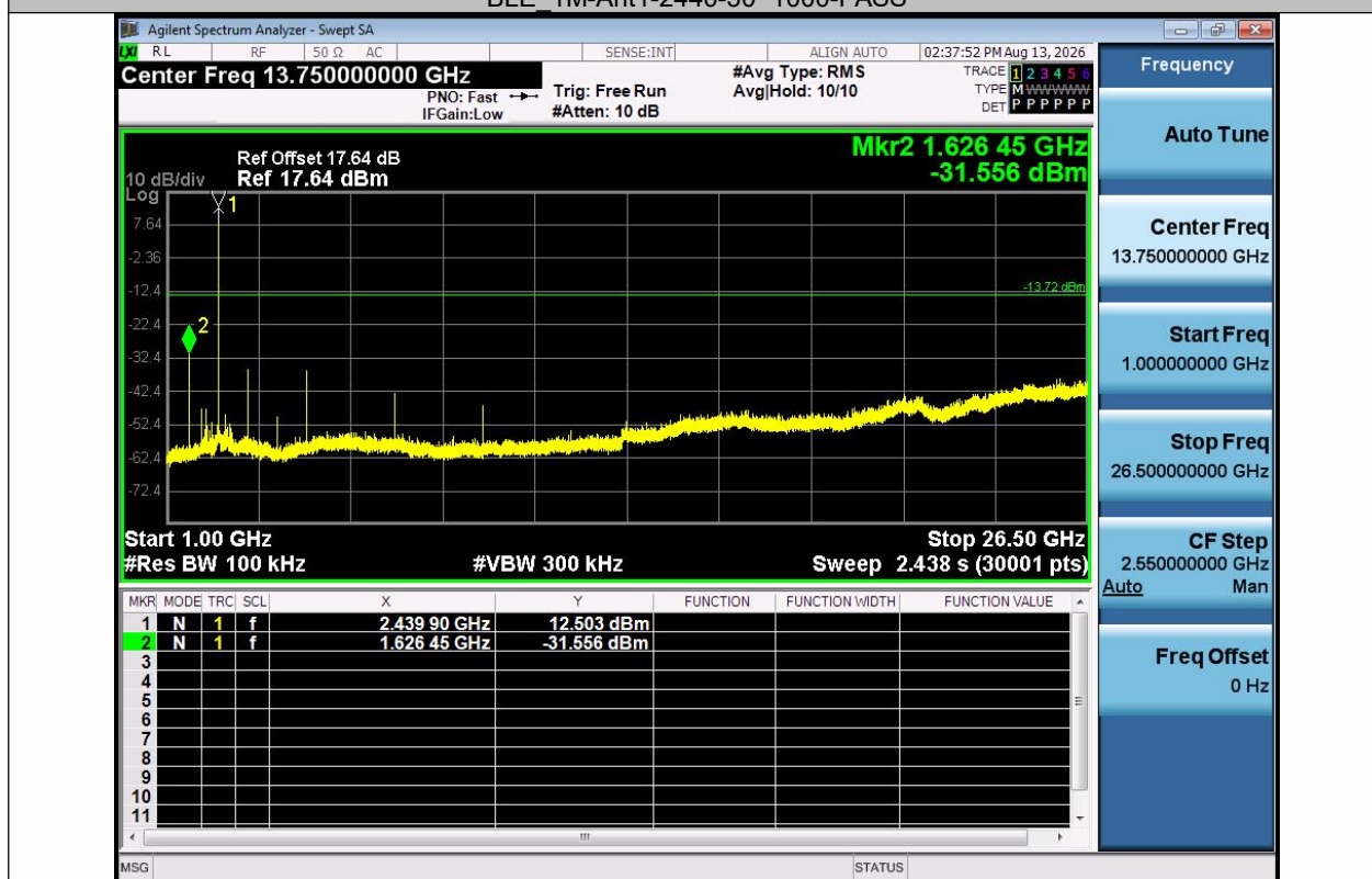
BLE_1M-Ant1-2440-1000~26500-PASS
