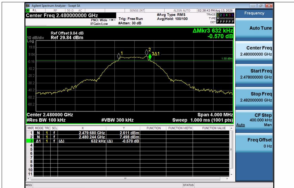
BLE_1M-Ant1-2480-PASS
