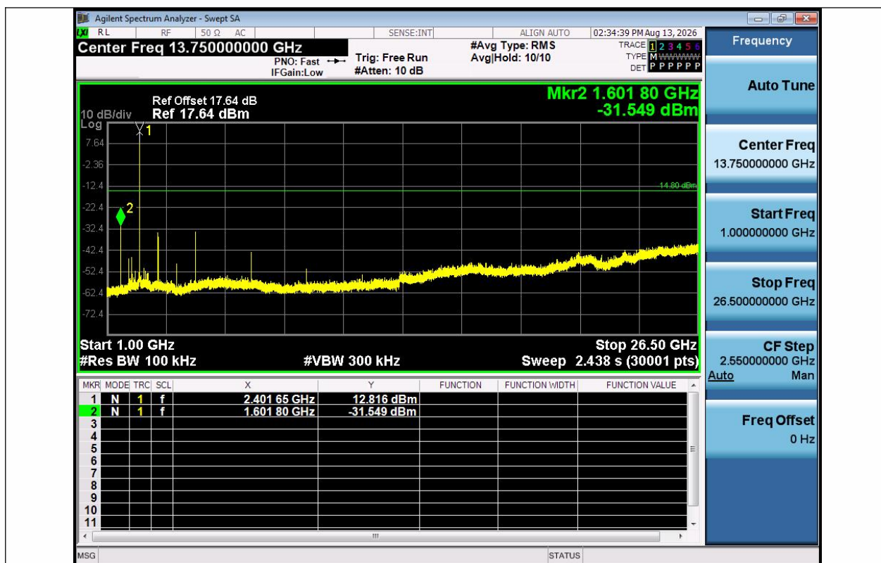
BLE_1M-Ant1-2402-1000~26500-PASS
