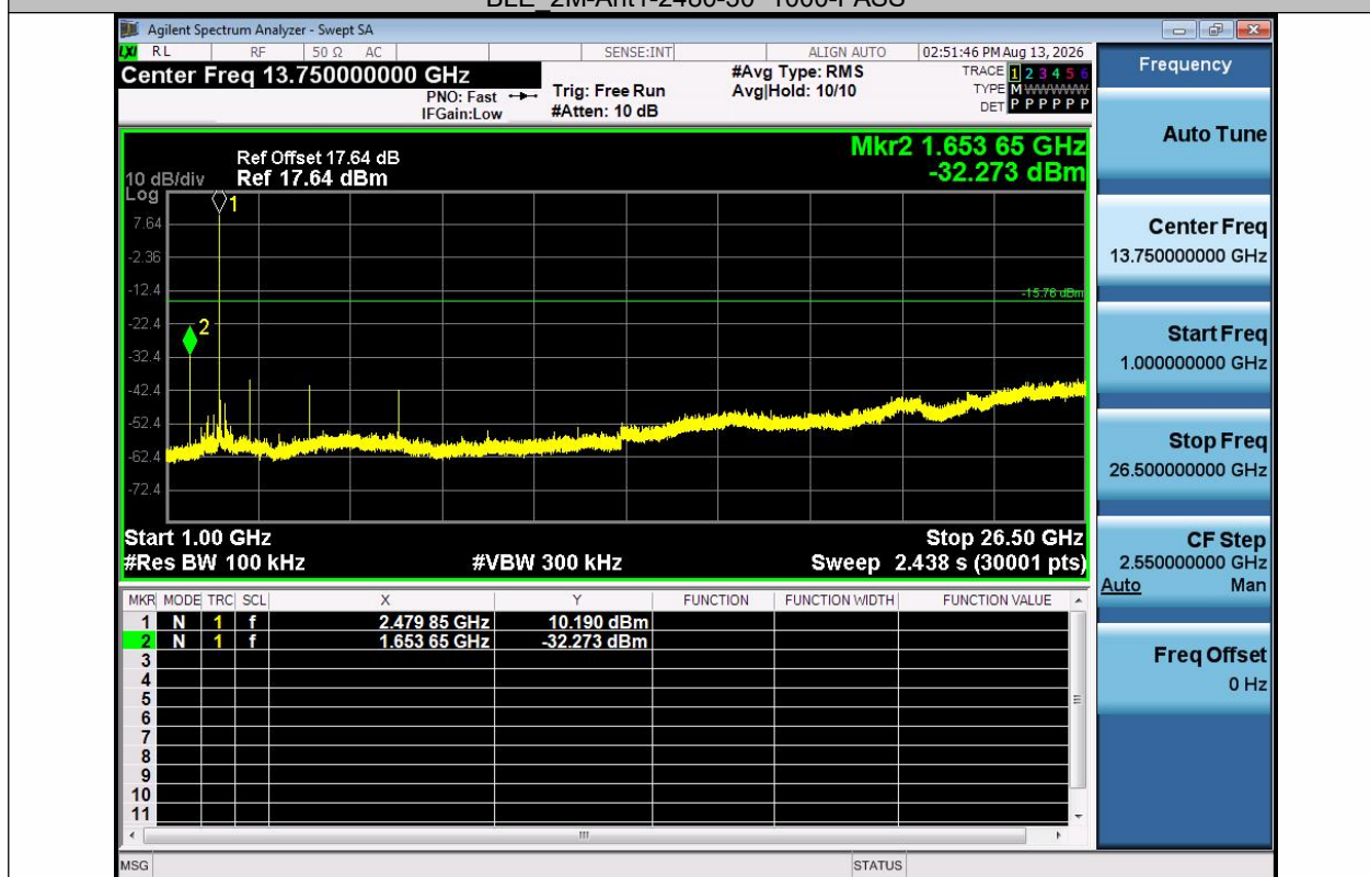
BLE_2M-Ant1-2480-1000~26500-PASS
