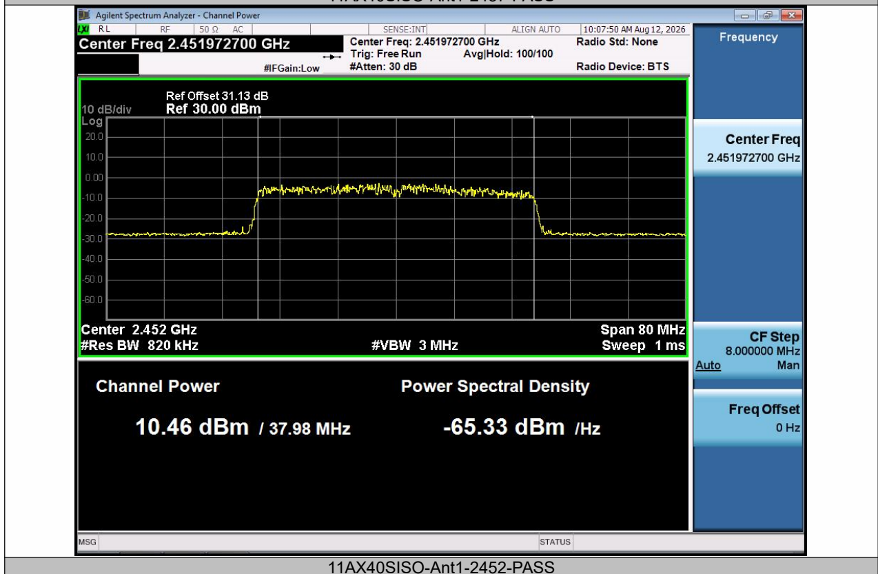
11AX40SISO-Ant1-2452-PASS
