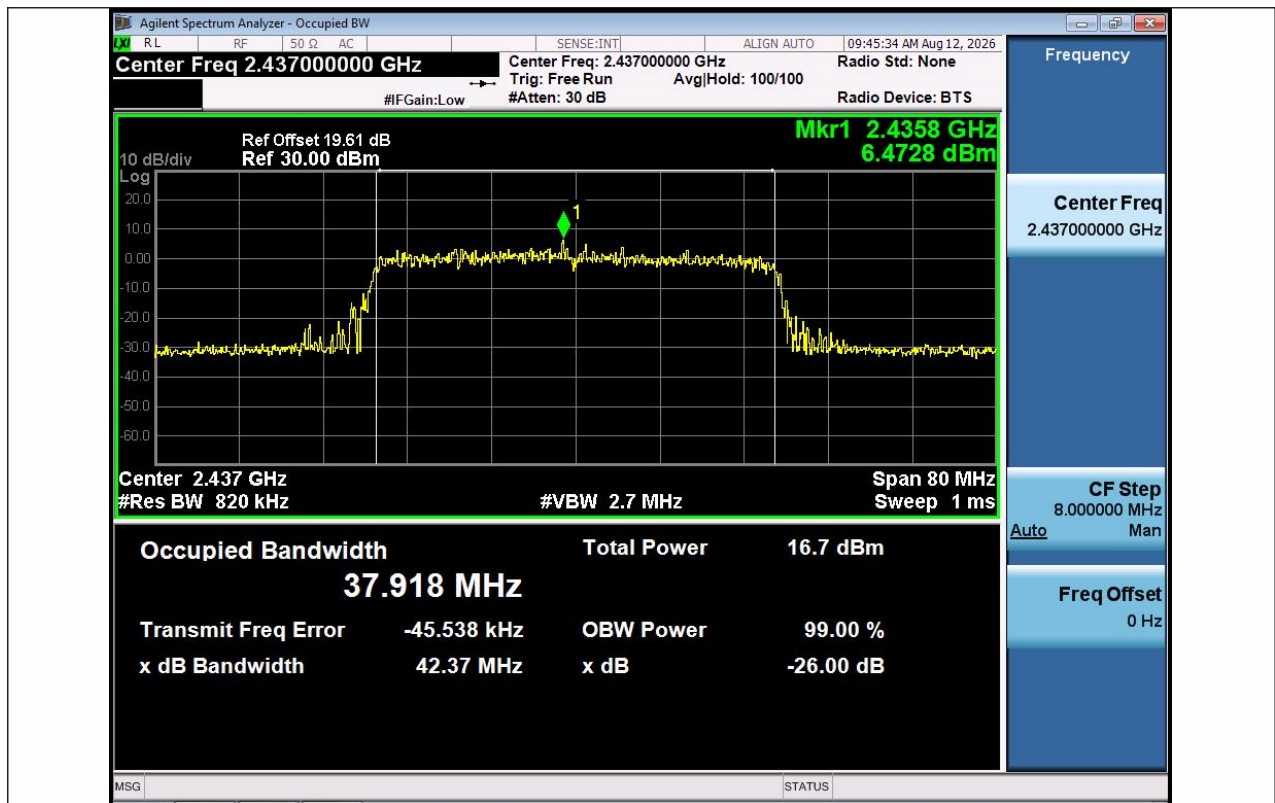
11AX40SISO-Ant1-2437
