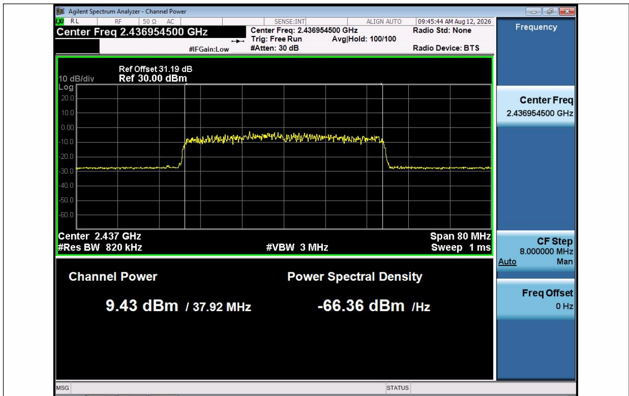
11AX40SISO-Ant1-2437-PASS
