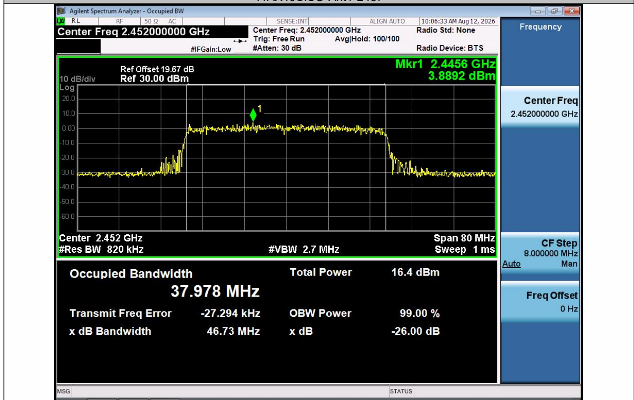
11AX40SISO-Ant1-2452
