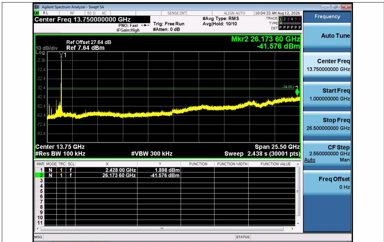
11AX40SISO-Ant1-2437-1000~26500-PASS
