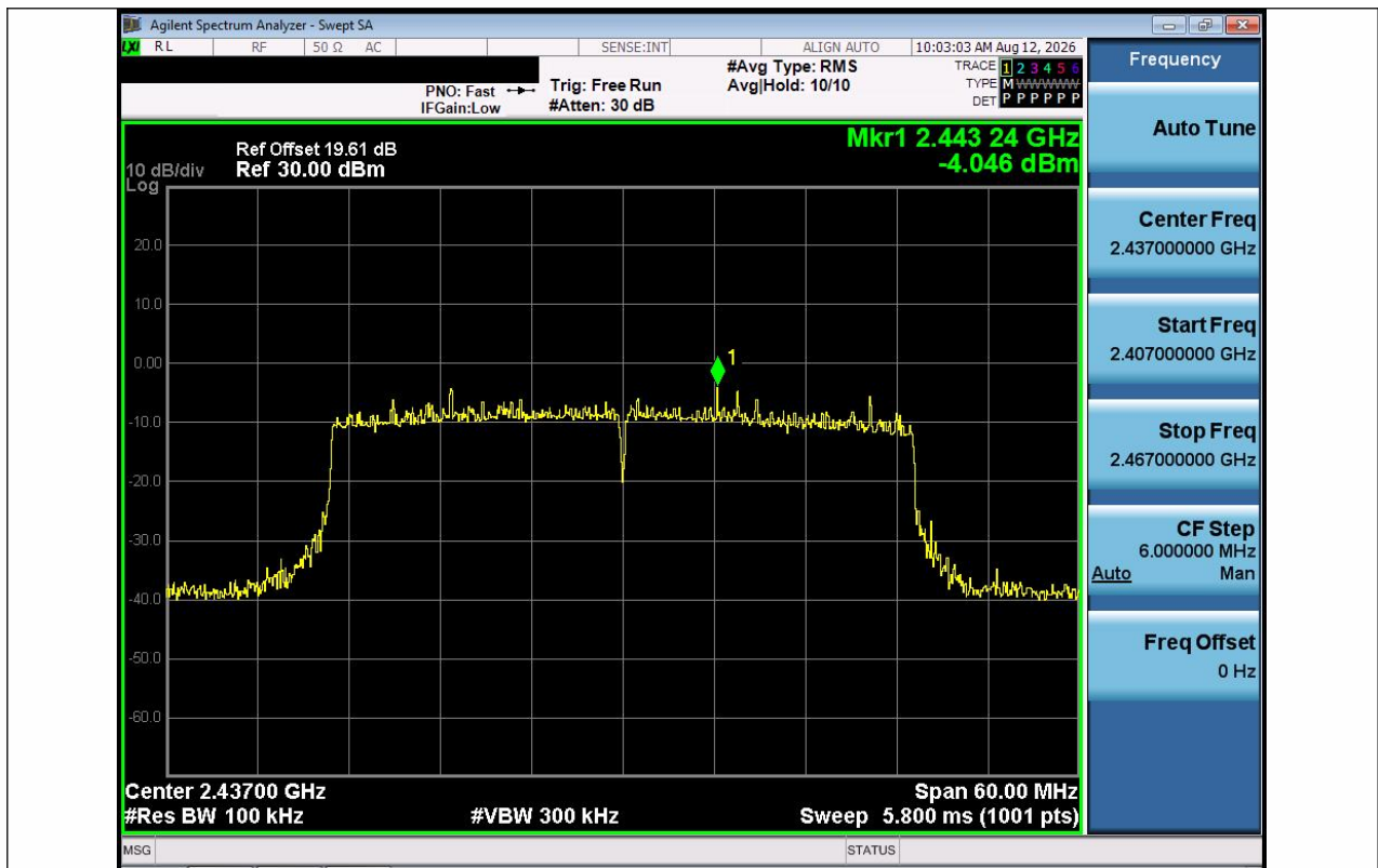
11AX40SISO-Ant1-2437-0~Reference-PASS
