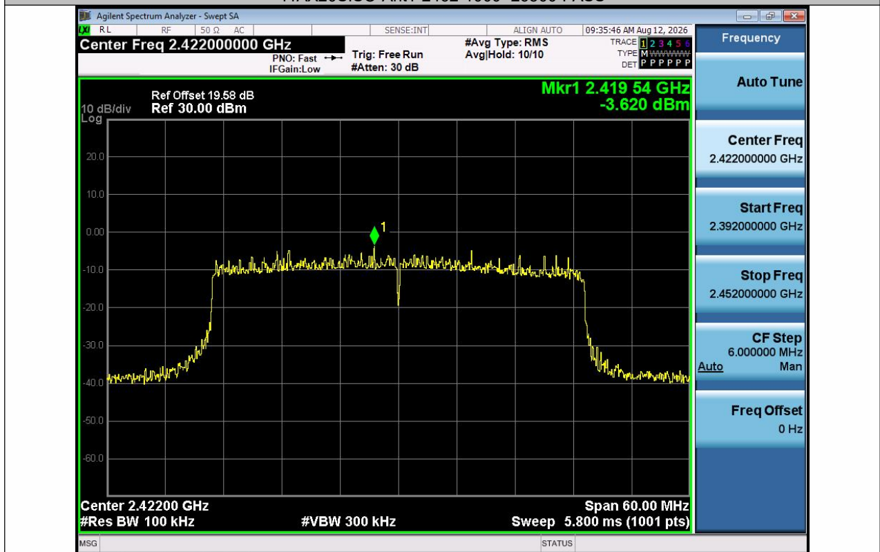
11AX40SISO-Ant1-2422-0~Reference-PASS
