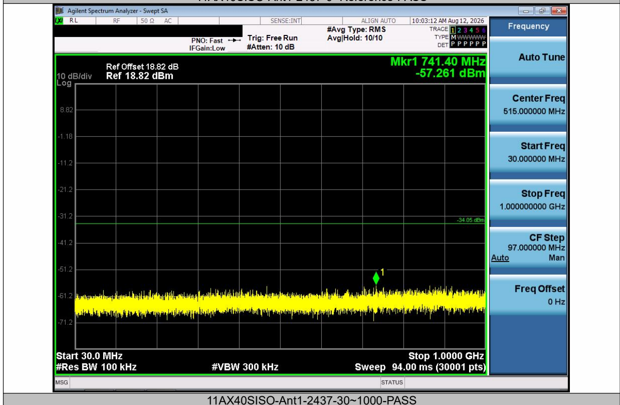
11AX40SISO-Ant1-2437-30~1000-PASS
