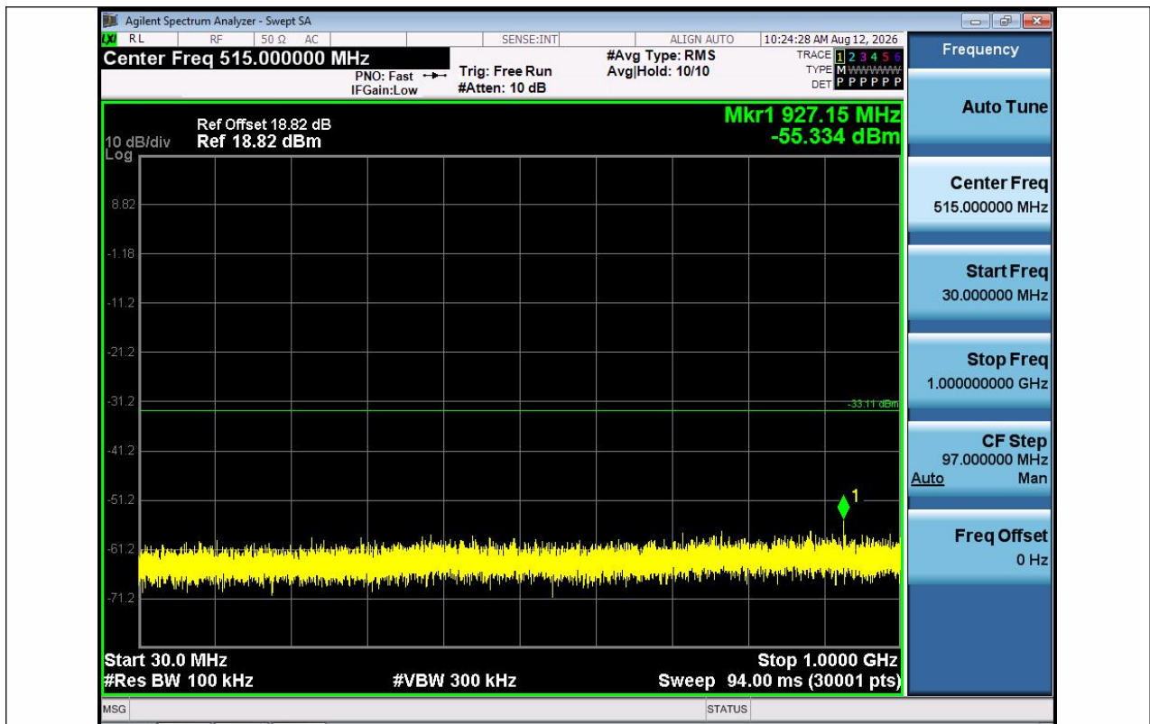
11AX40SISO-Ant1-2452-30~1000-PASS
