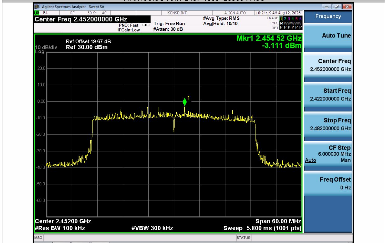
11AX40SISO-Ant1-2452-0~Reference-PASS
