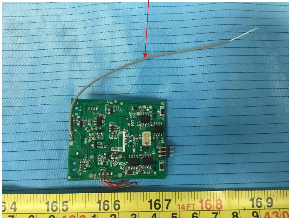
2.4GHz receiver antenna
