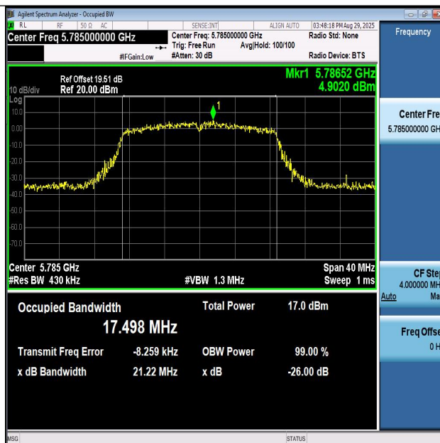
11N20SISO-Ant1-5785
