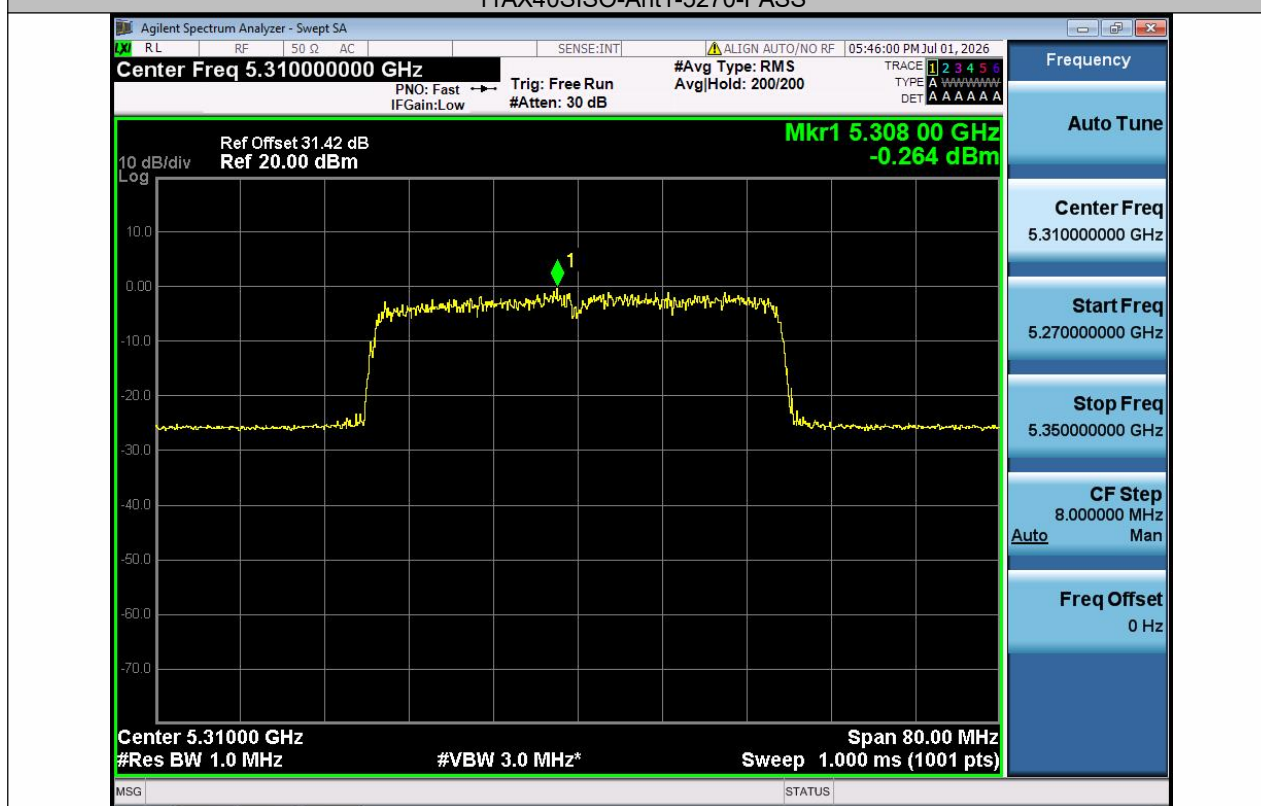
11AX40SISO-Ant1-5310-PASS
