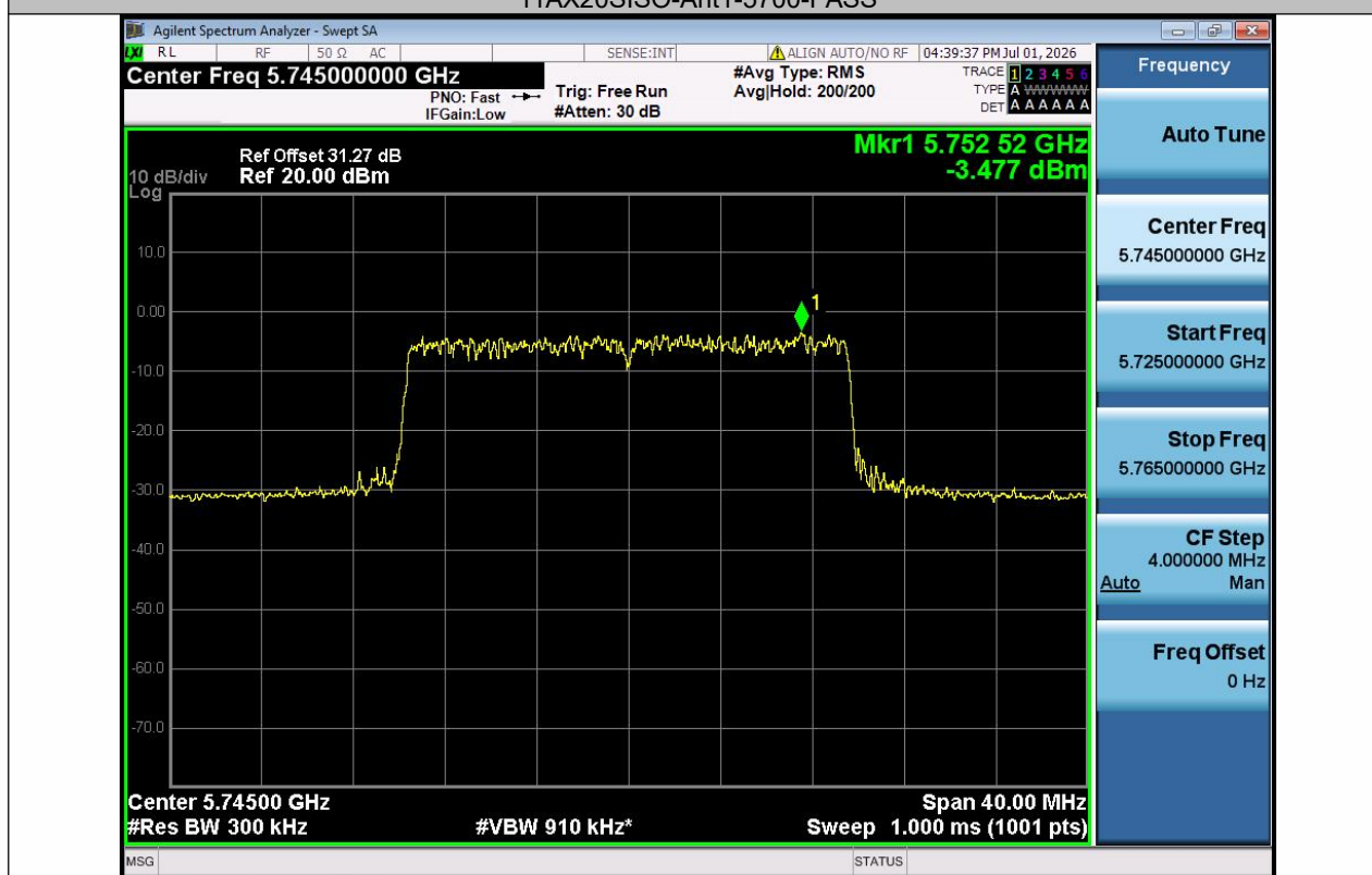
11AX20SISO-Ant1-5745-PASS
