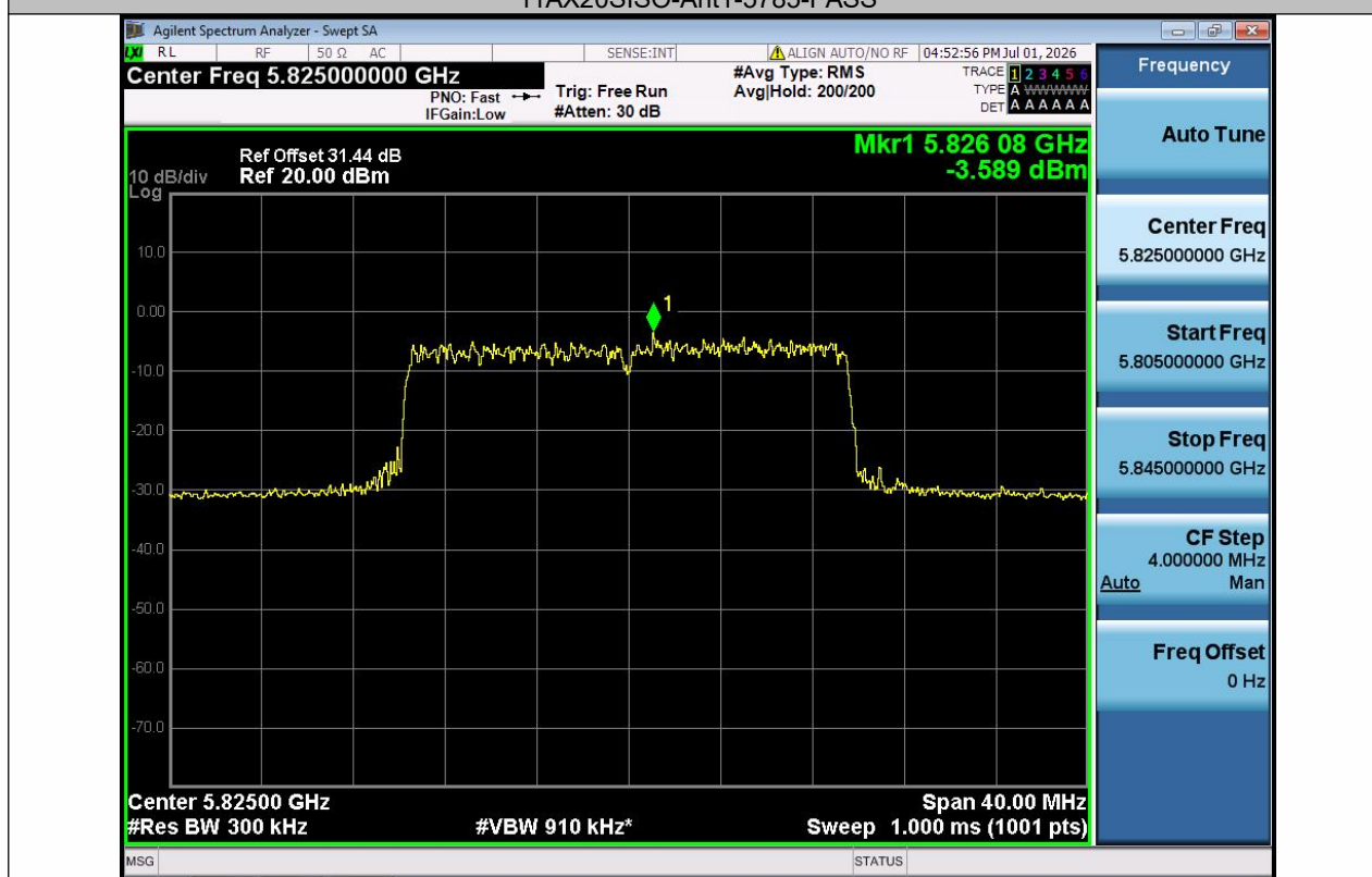
11AX20SISO-Ant1-5825-PASS
