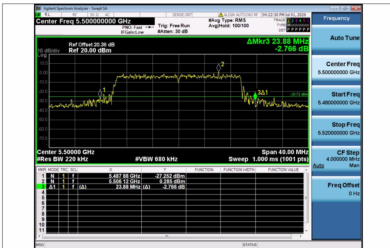
11AX20SISO-Ant1-5500
