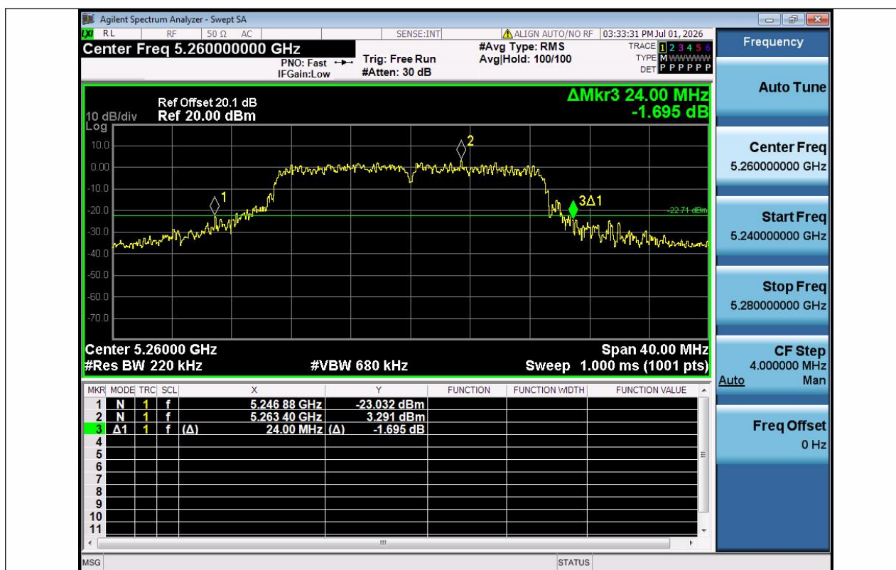
11AC20SISO-Ant1-5260
