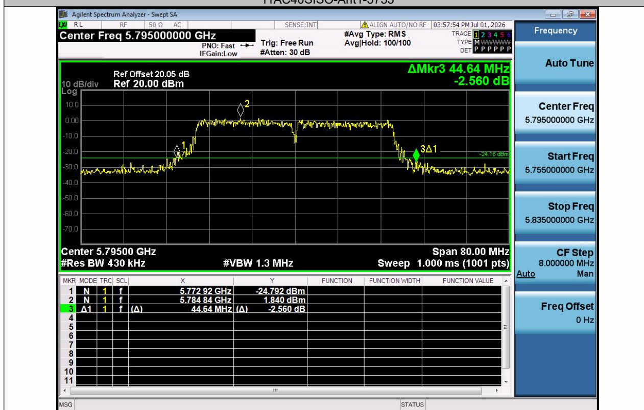
11AC40SISO-Ant1-5795
