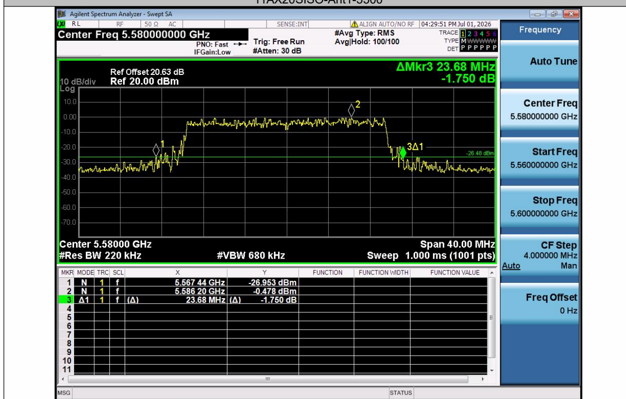
11AX20SISO-Ant1-5580
