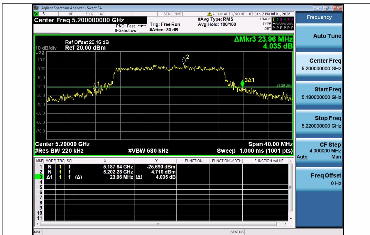
11AC20SISO-Ant1-5200
