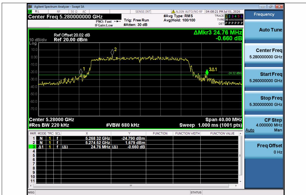
11AX20SISO-Ant1-5280
