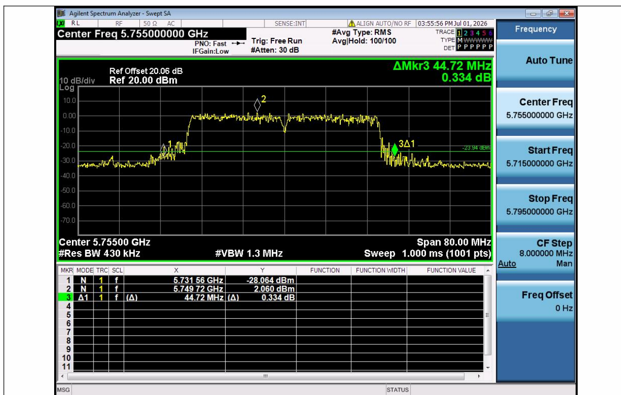
11AC40SISO-Ant1-5755
