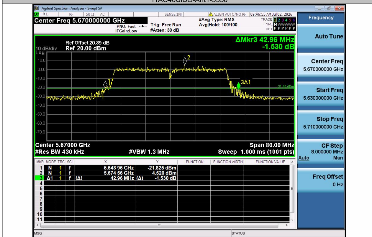
11AC40SISO-Ant1-5670
