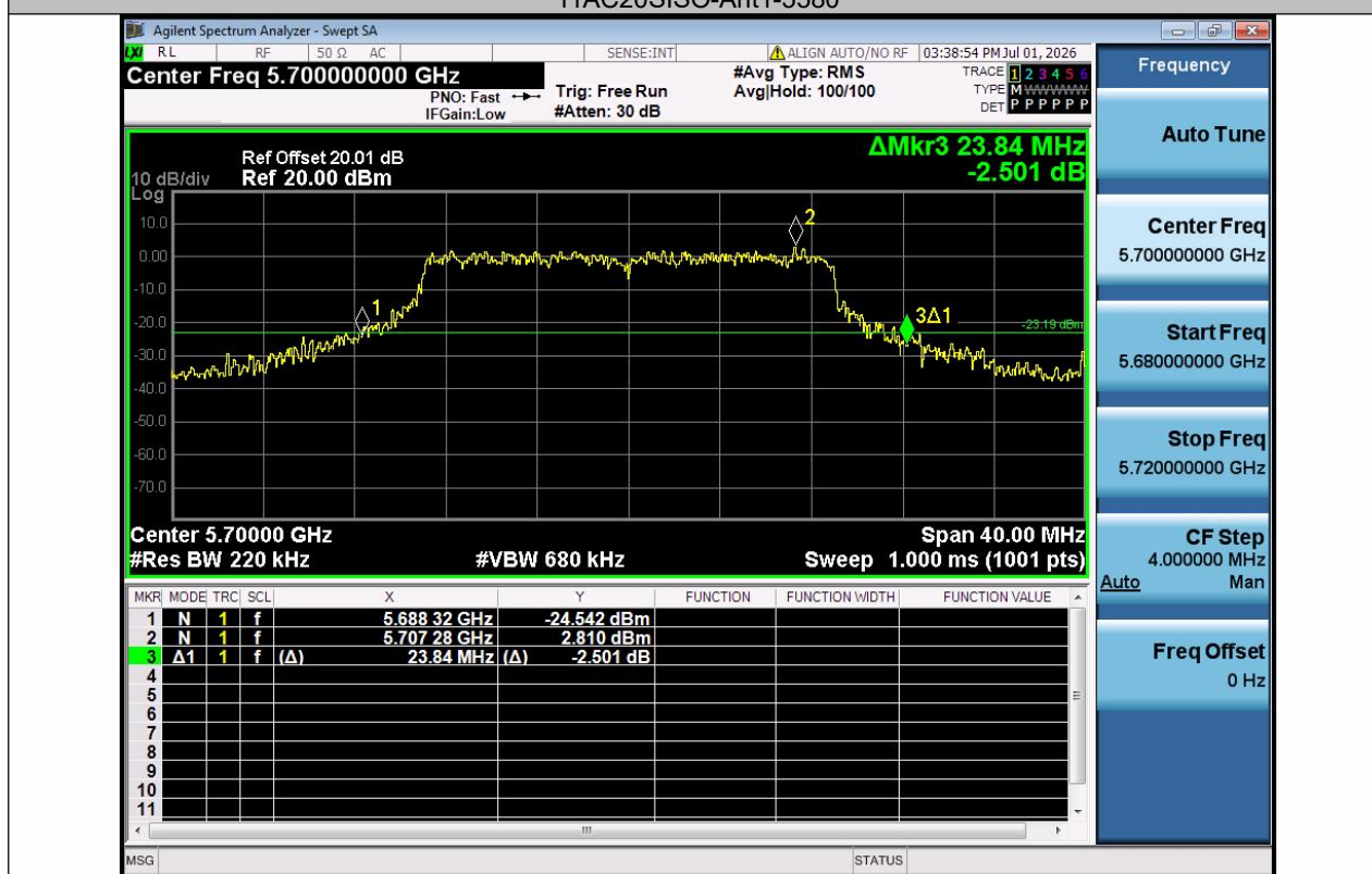
11AC20SISO-Ant1-5700
