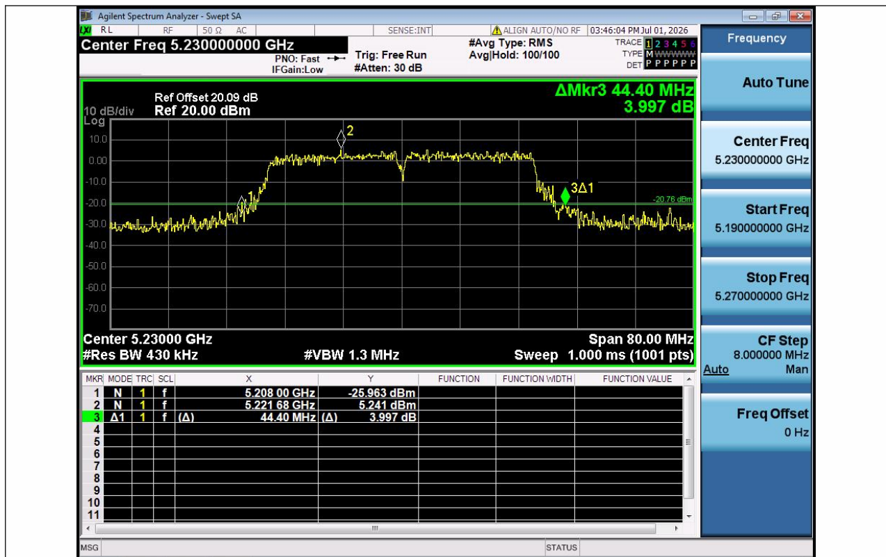
11AC40SISO-Ant1-5230
