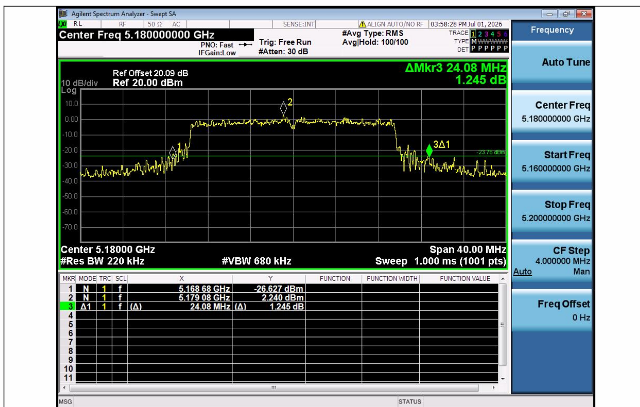
11AX20SISO-Ant1-5180
