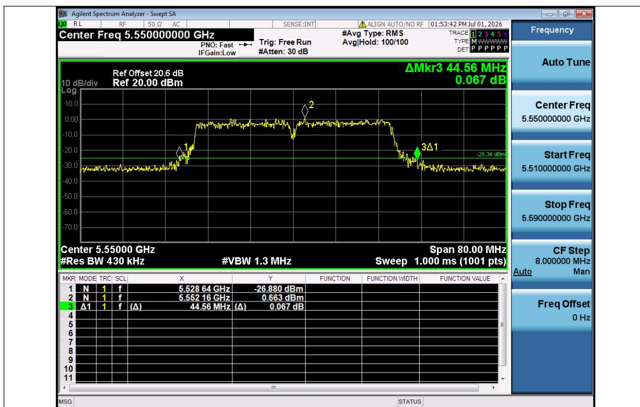
11AC40SISO-Ant1-5550
