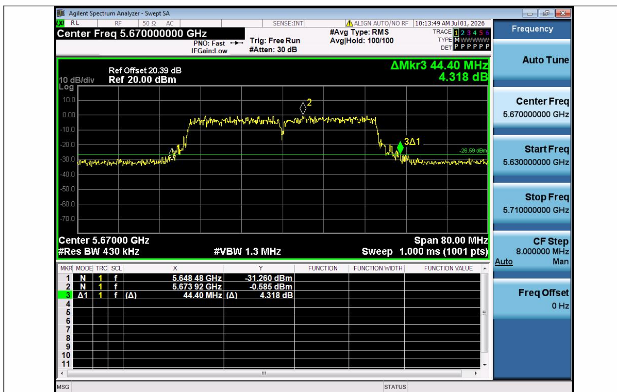
11N40SISO-Ant1-5670
