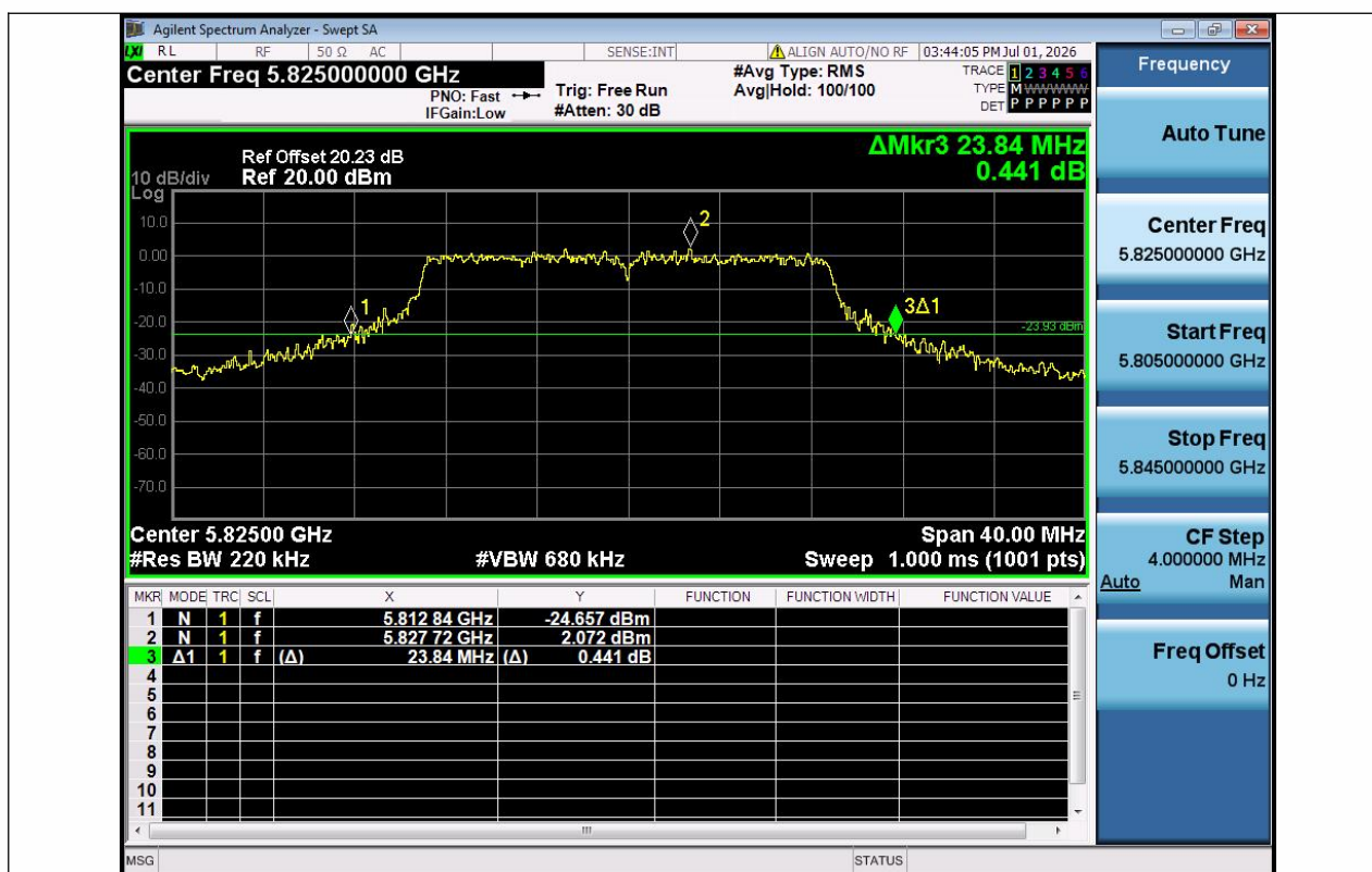
11AC20SISO-Ant1-5825
