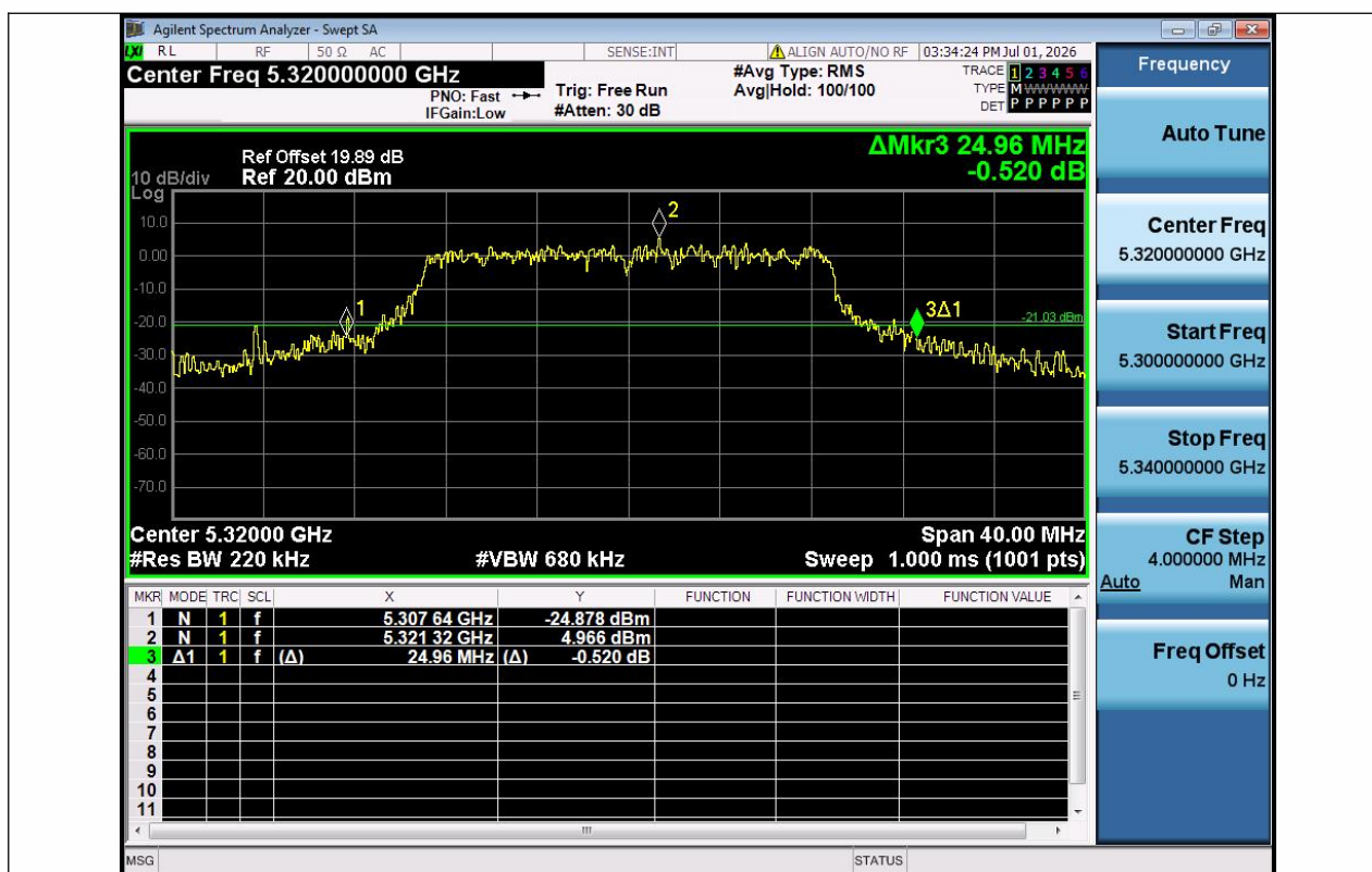
11AC20SISO-Ant1-5320
