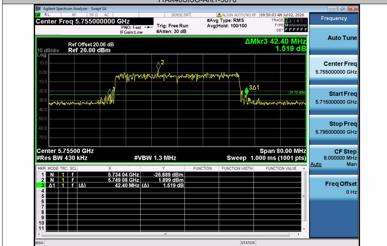
11AX40SISO-Ant1-5755
