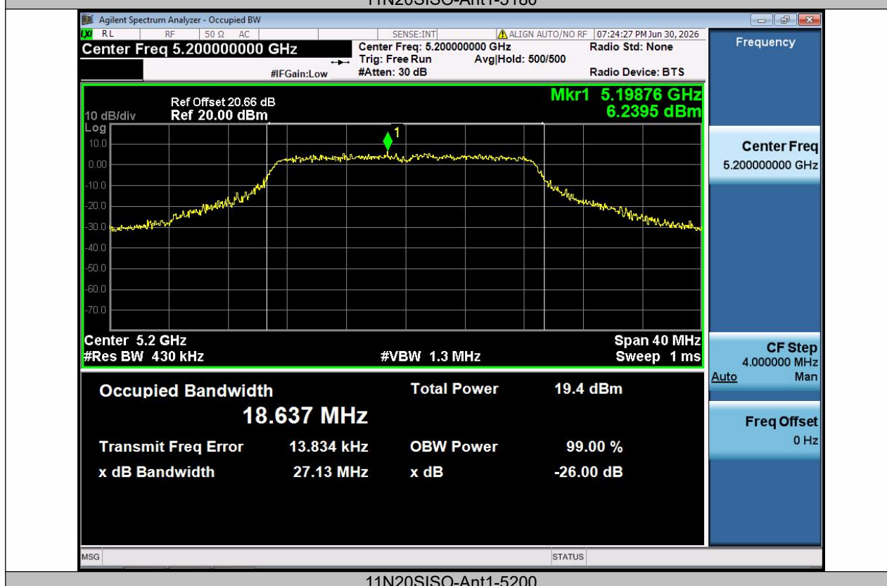
11N20SISO-Ant1-5200
