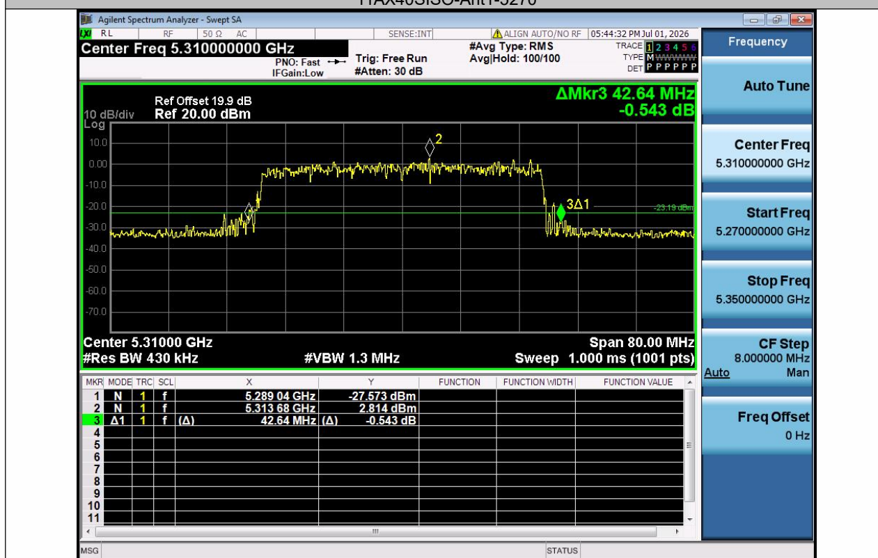
11AX40SISO-Ant1-5310
