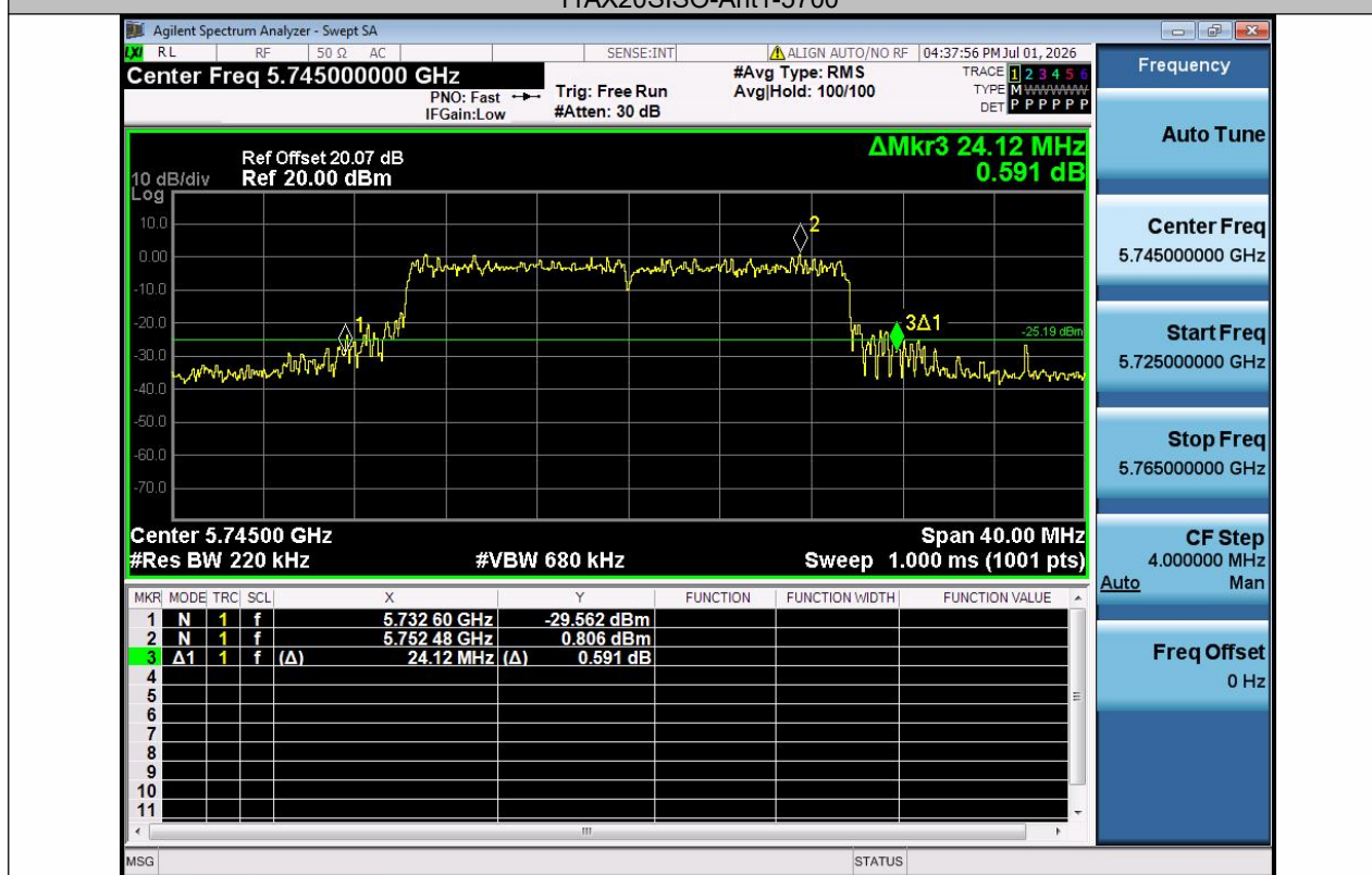
11AX20SISO-Ant1-5745
