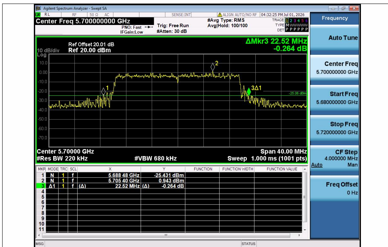
11AX20SISO-Ant1-5700
