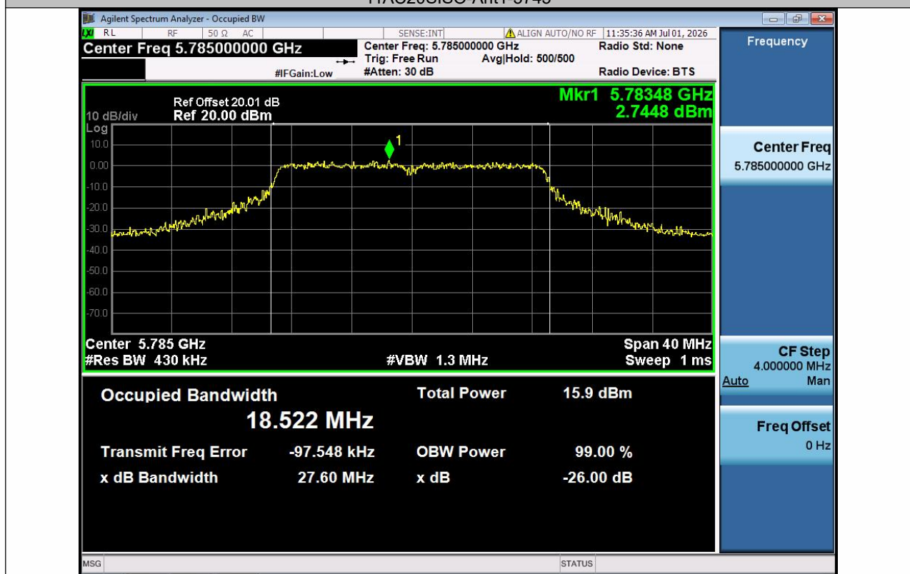
11AC20SISO-Ant1-5785
