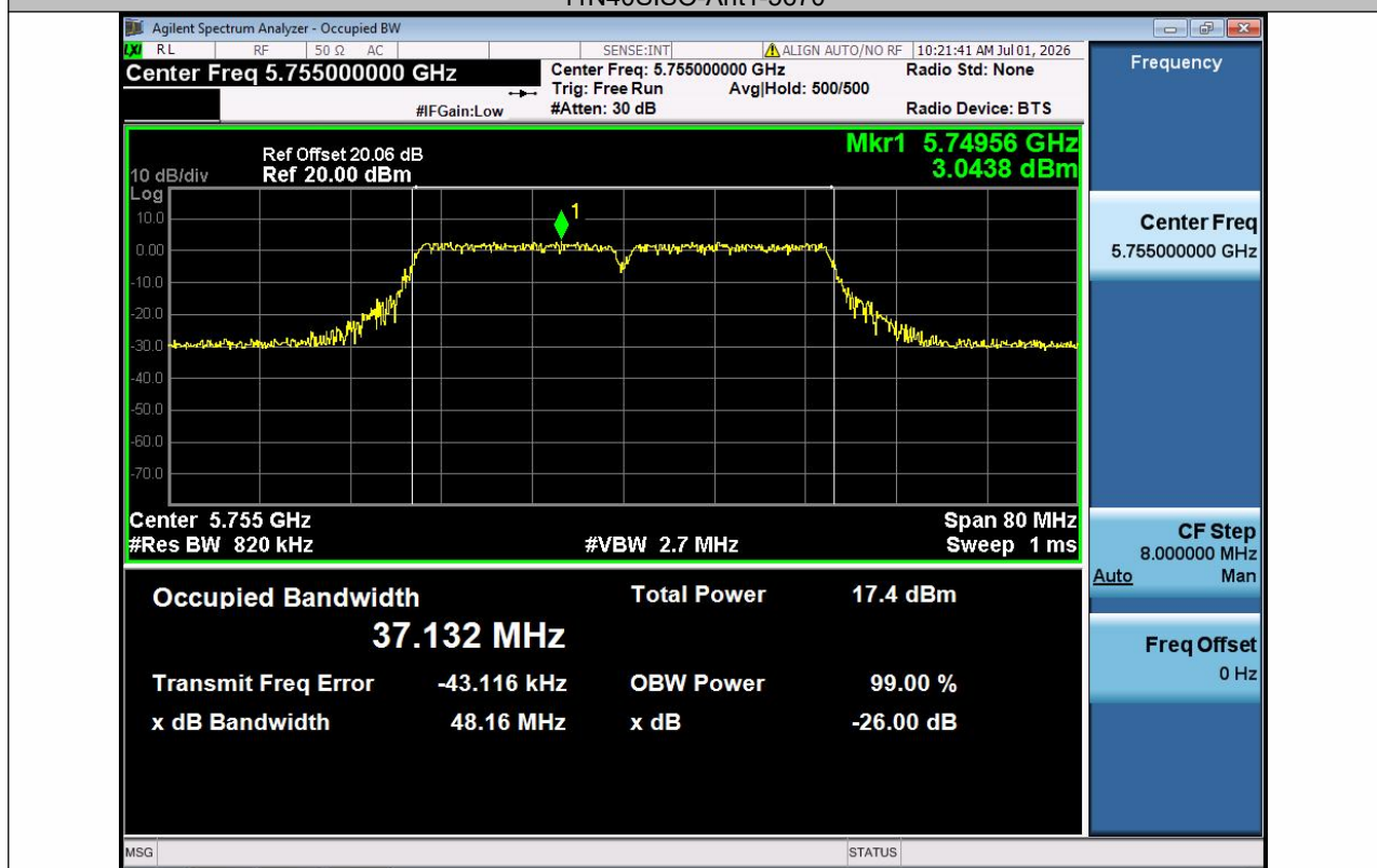
11N40SISO-Ant1-5755
