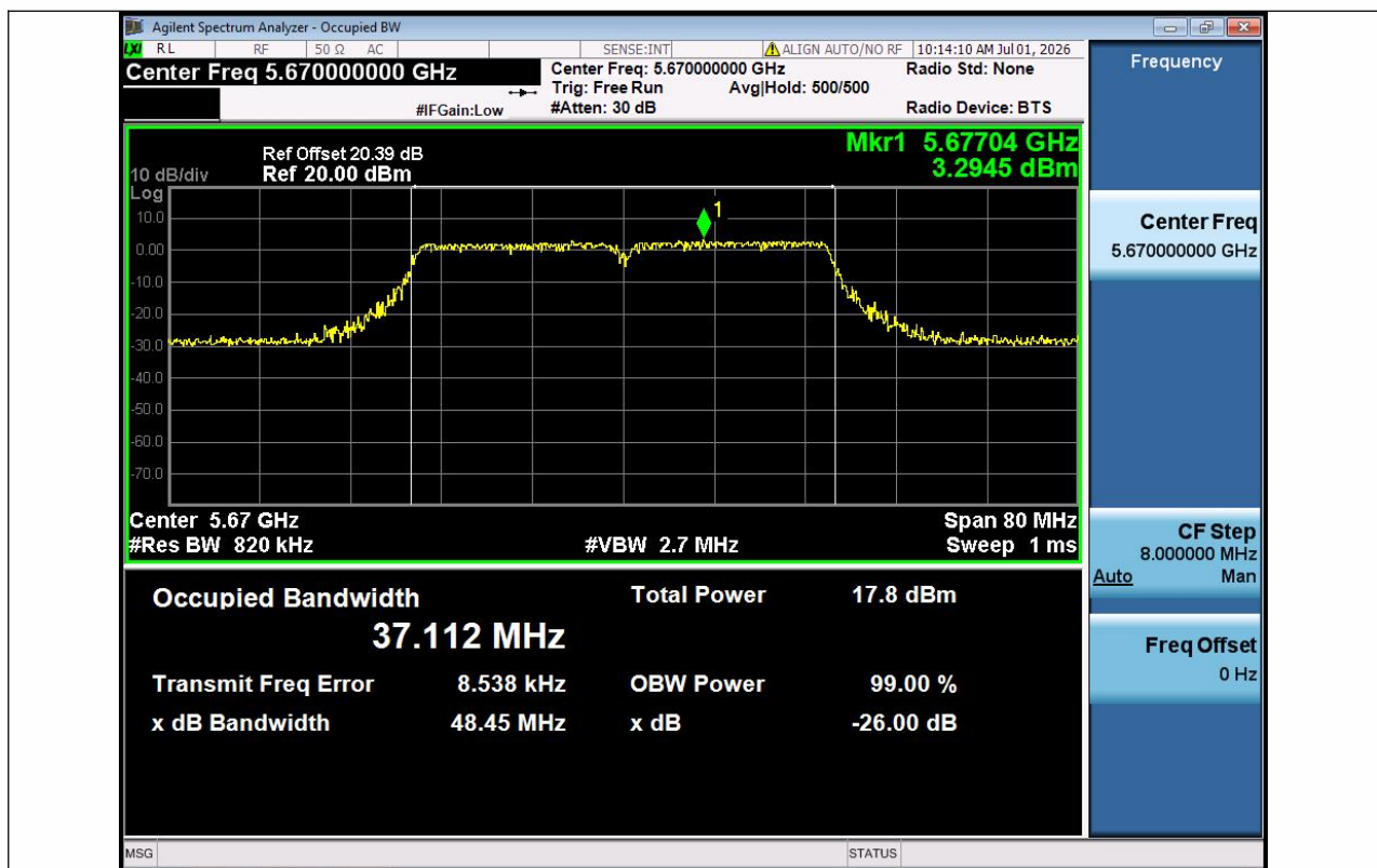
11N40SISO-Ant1-5670
