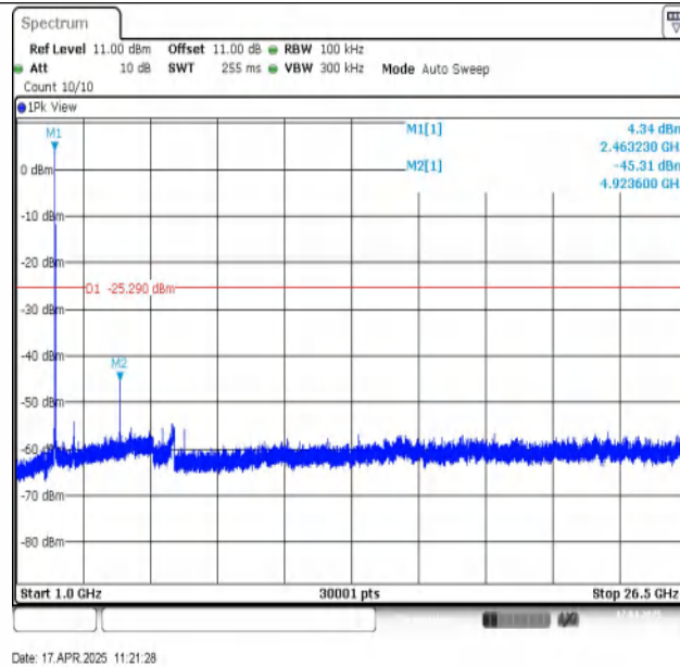
11B-Ant1-2462-1000~26500-PASS
