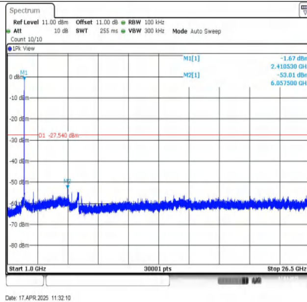
11N20SISO-Ant1-2412-1000~26500-PASS
