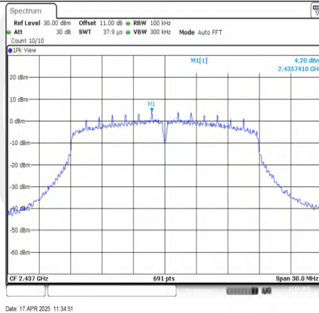
11N20SISO-Ant1-2437-0~Reference-PASS
