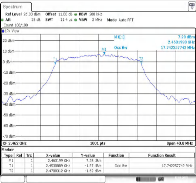
11N20SISO-Ant1-2462
