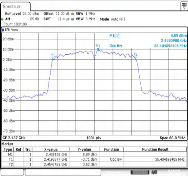
11N40SISO-Ant1-2437
