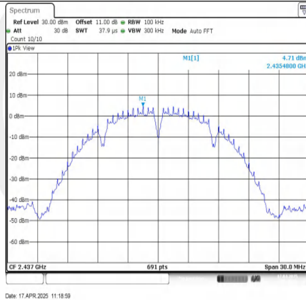
11B-Ant1-2437-0~Reference-PASS
