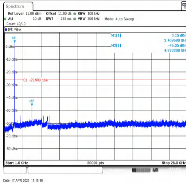
11B-Ant1-2412-1000~26500-PASS
