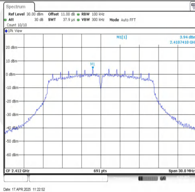
11G-Ant1-2412-0~Reference-PASS
