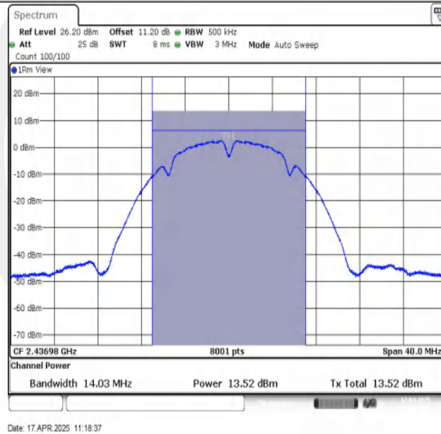
11B-Ant1-2437-PASS
