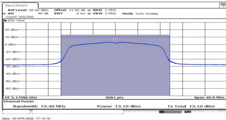
11A-Ant1-5180
