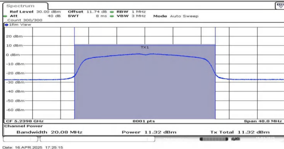
11N20SISO-Ant1-5240
