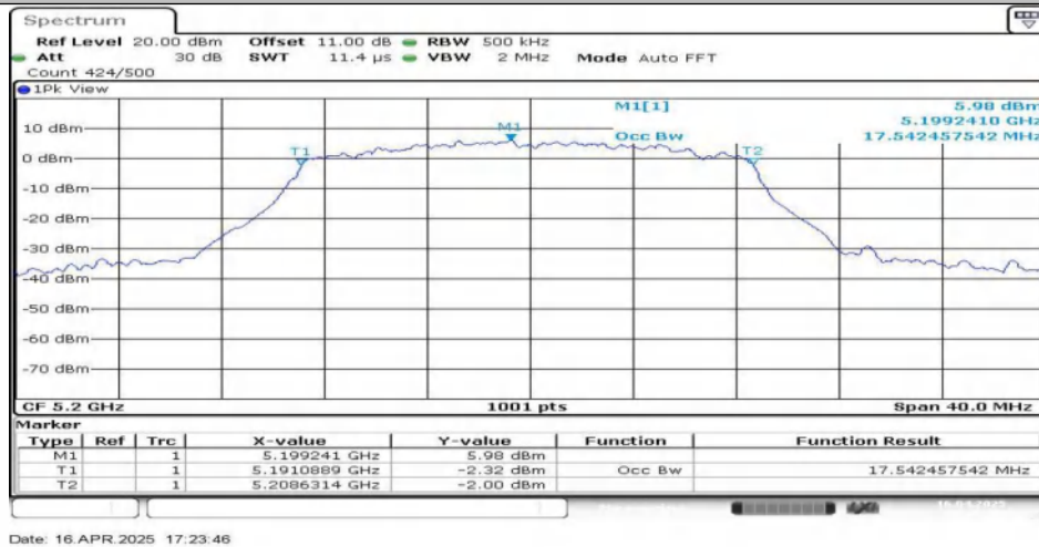
11N20SISO-Ant1-5200
