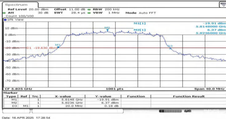
11N20SISO-Ant1-5825
