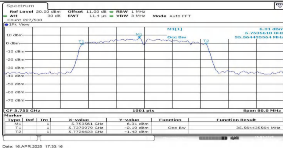
11N40SISO-Ant1-5755
