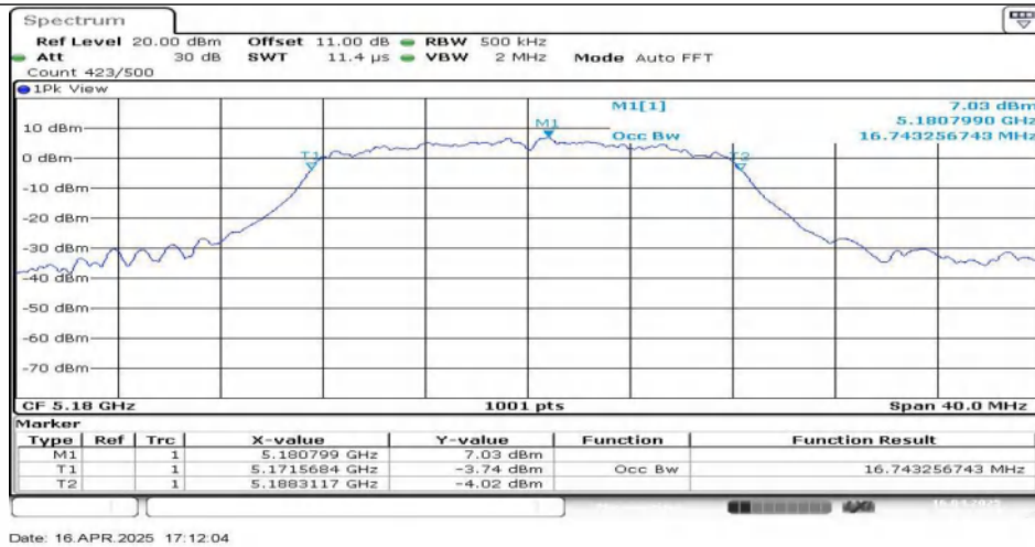
11A-Ant1-5180
