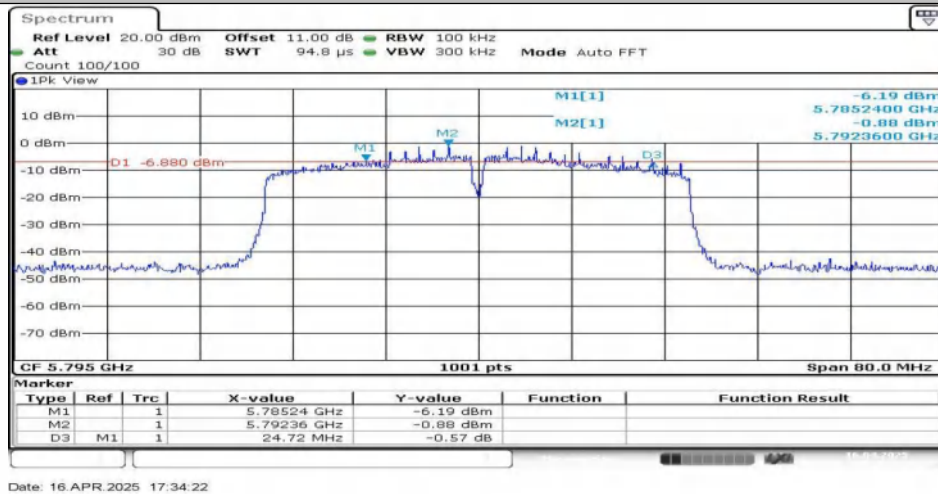
11N40SISO-Ant1-5795
