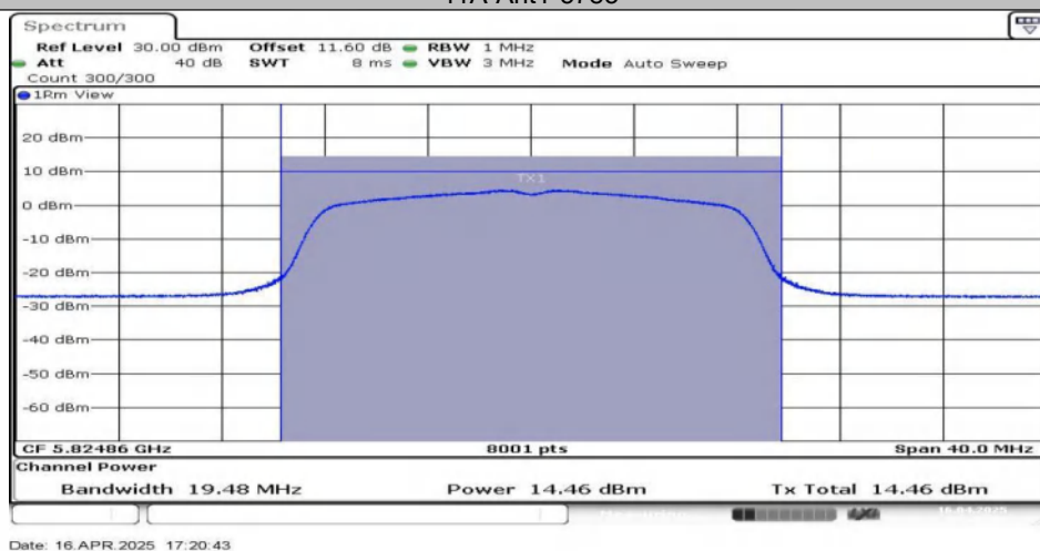
11A-Ant1-5825
