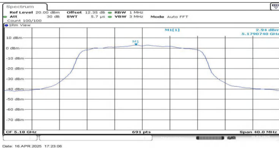
11N20SISO-Ant1-5180
