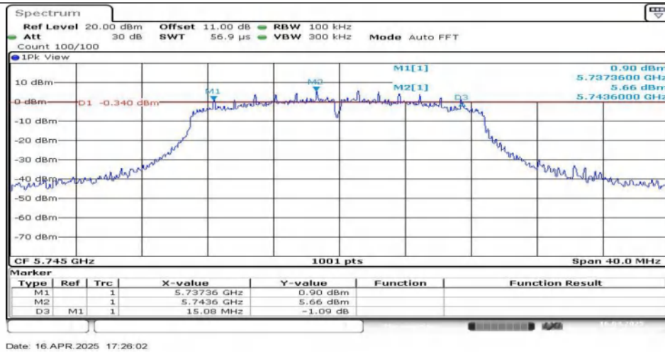
11N20SISO-Ant1-5745
