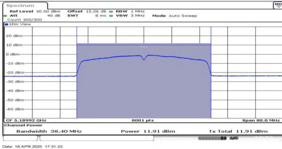
11N40SISO-Ant1-5190
