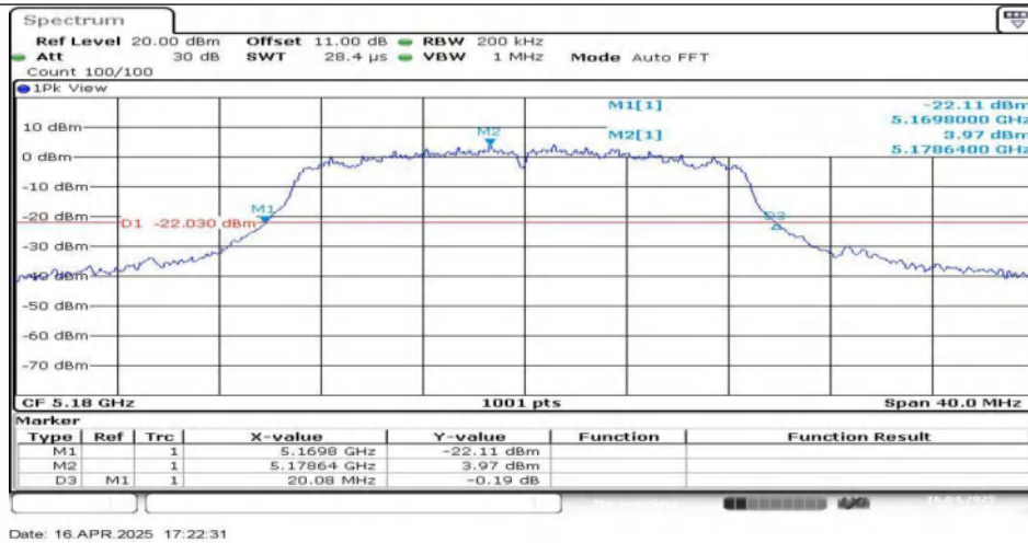
11N20SISO-Ant1-5180
