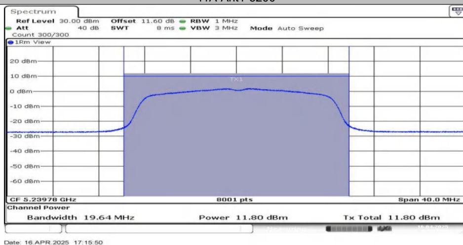
11A-Ant1-5240
