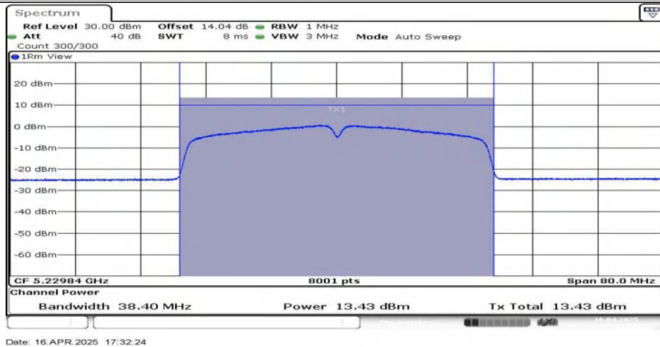
11N40SISO-Ant1-5230
