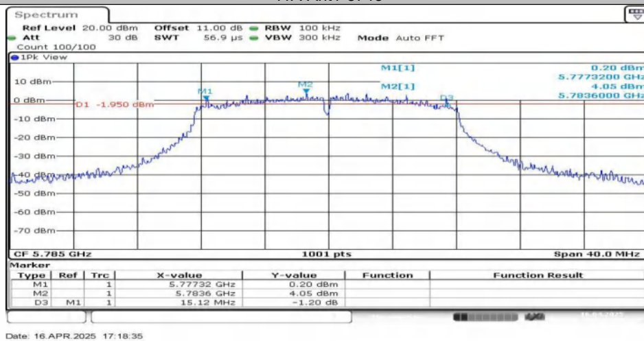
11A-Ant1-5785
