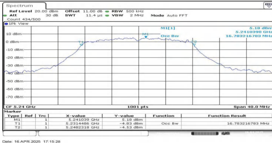
11A-Ant1-5240
