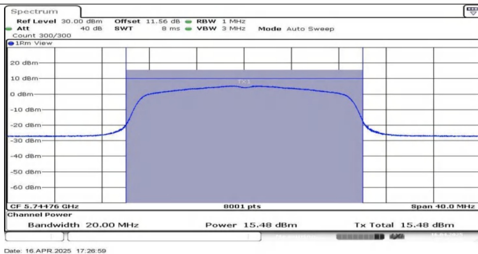
11N20SISO-Ant1-5745
