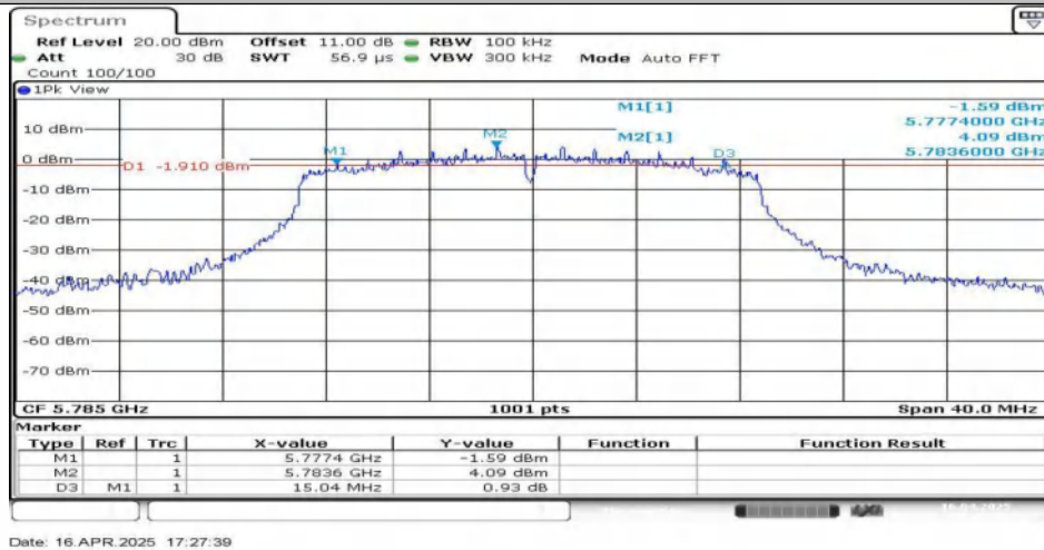
11N20SISO-Ant1-5785
