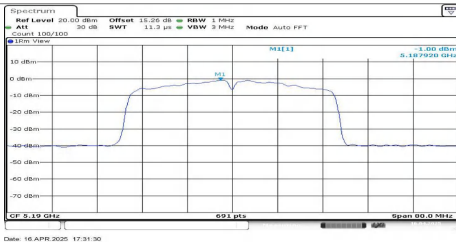
11N40SISO-Ant1-5190
