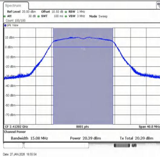
11G-Ant1-2412-PASS
