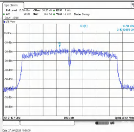
11N40SISO-Ant1-2437-PASS
