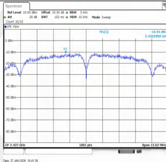
11B-Ant1-2437-PASS
