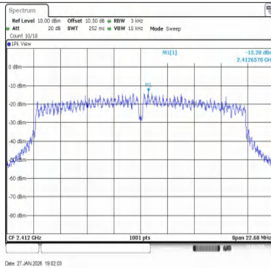
11N20SISO-Ant1-2412-PASS
