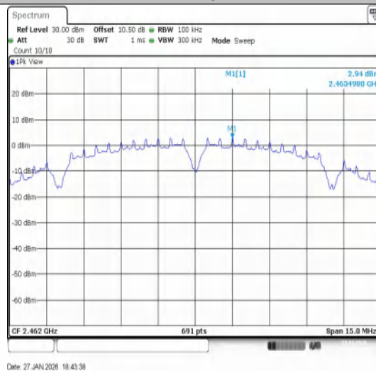
11B-Ant1-2462-PASS
