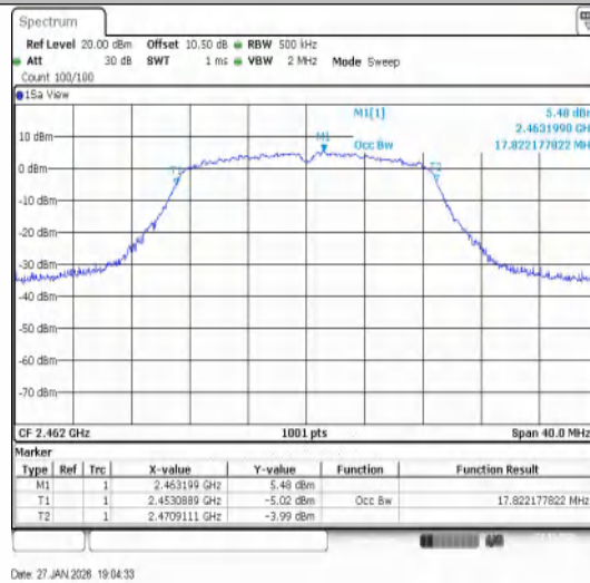
11N20SISO-Ant1-2462
