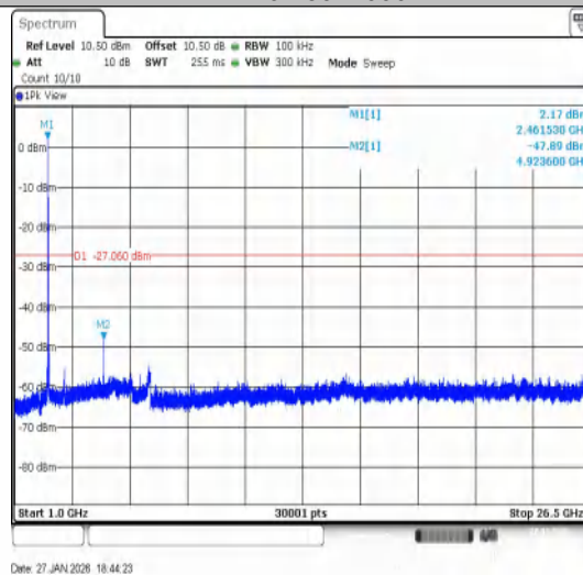
11B-Ant1-2462-1000~26500-PASS
