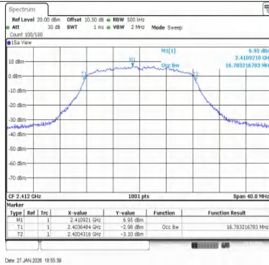
11G-Ant1-2412
