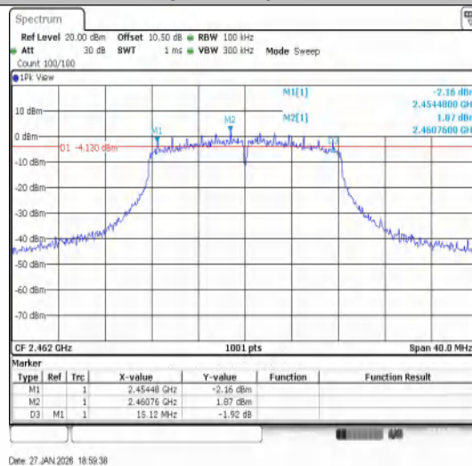
11G-Ant1-2462-PASS
