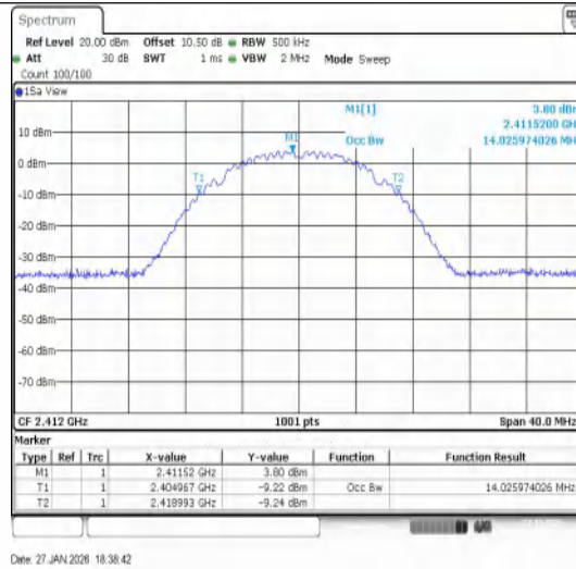
11B-Ant1-2412
