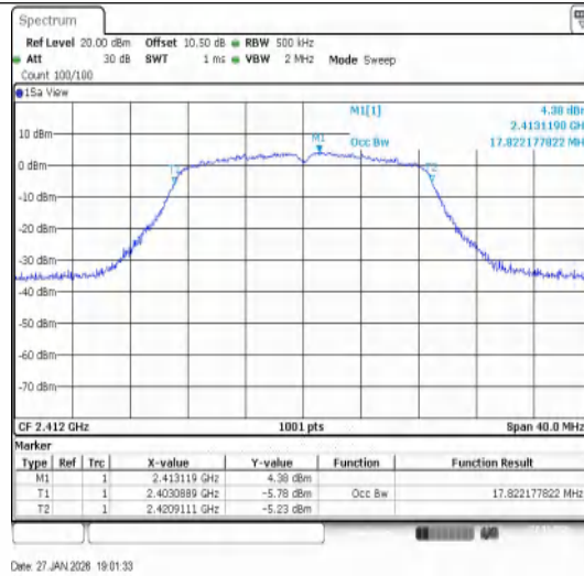
11N20SISO-Ant1-2412
