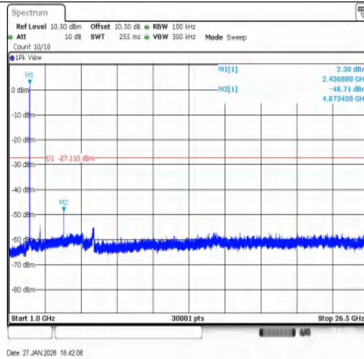
11B-Ant1-2437-1000~26500-PASS
