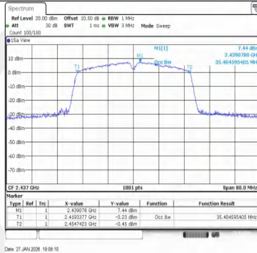
11N40SISO-Ant1-2437
