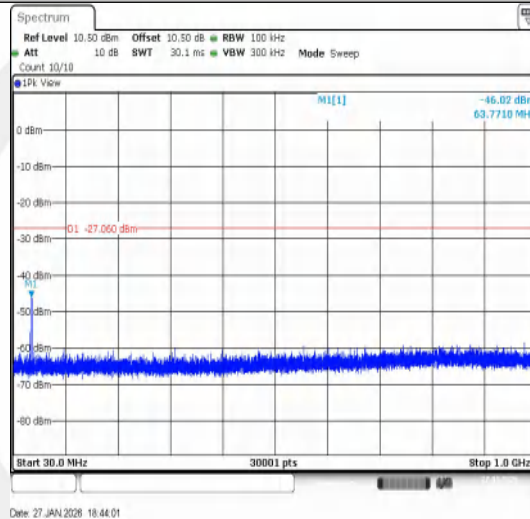
11B-Ant1-2462-30~1000-PASS
