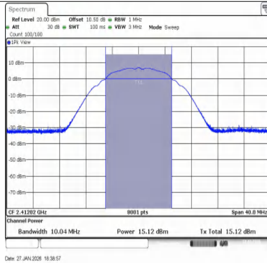
11B-Ant1-2412-PASS
