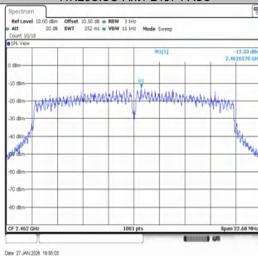
11N20SISO-Ant1-2462-PASS
