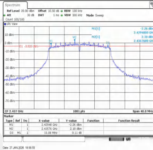
11G-Ant1-2437-PASS
