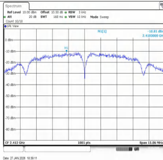
11B-Ant1-2412-PASS
