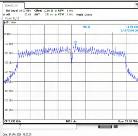
11N20SISO-Ant1-2437-PASS
