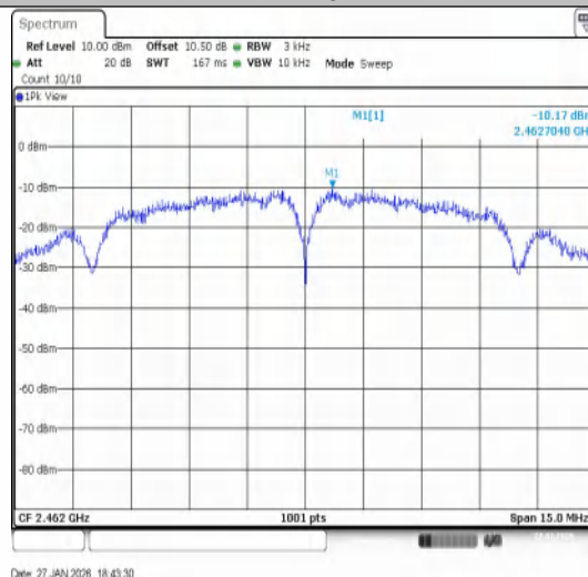
11B-Ant1-2462-PASS
