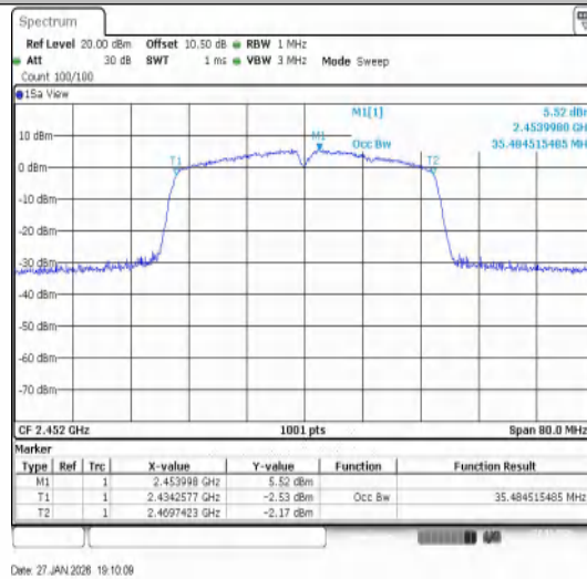
11N40SISO-Ant1-2452
