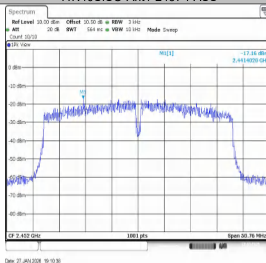
11N40SISO-Ant1-2452-PASS
