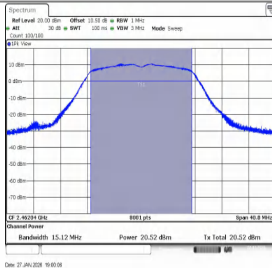
11G-Ant1-2462-PASS
