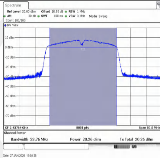
11N40SISO-Ant1-2437-PASS
