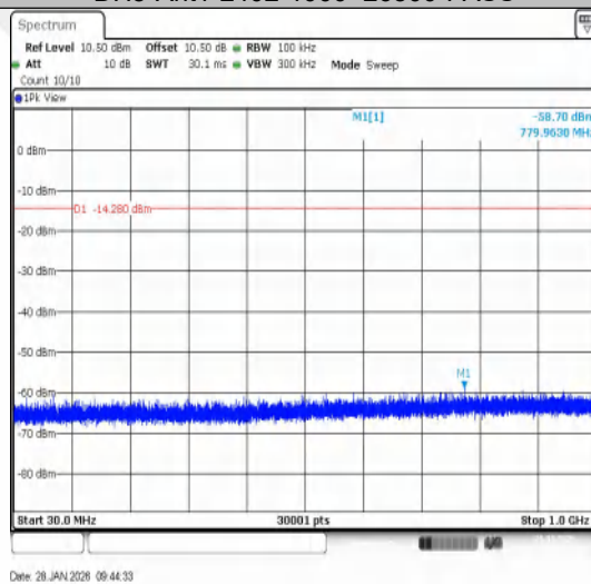
DH5-Ant1-2441-30~1000-PASS
