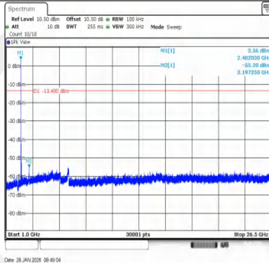
2DH5-Ant1-2402-1000~26500-PASS
