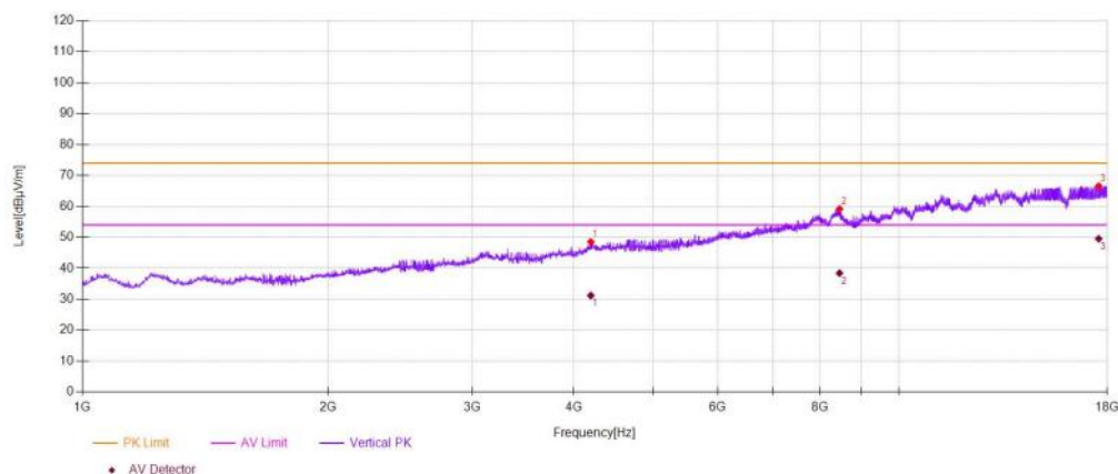
Antenna Polarization:Vertical
