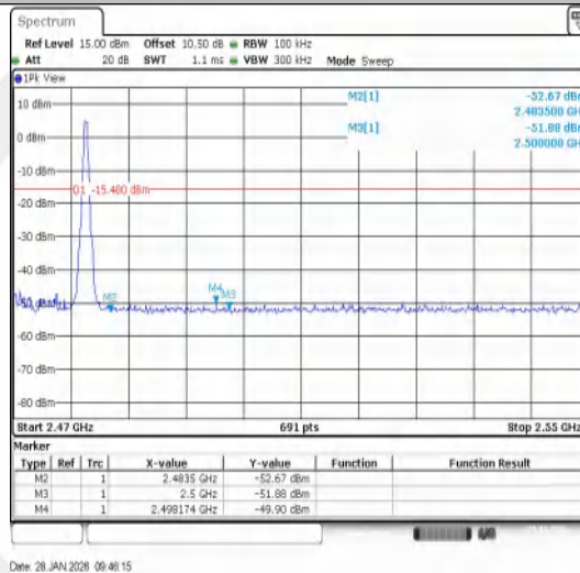
DH5-Ant1-2480-PASS
