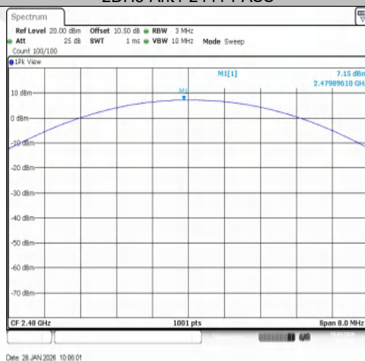
2DH5-Ant1-2480-PASS
