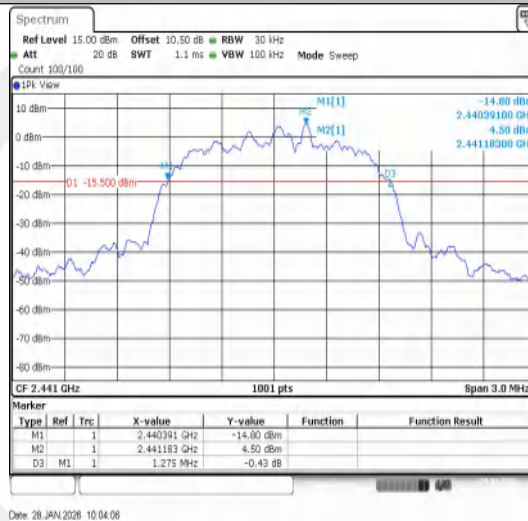
2DH5-Ant1-2441
