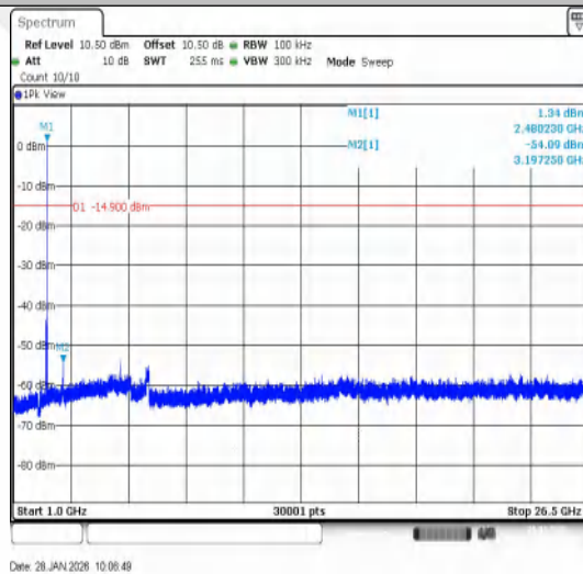
2DH5-Ant1-2480-1000~26500-PASS
