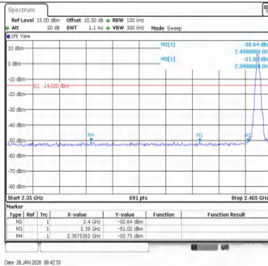
DH5-Ant1-2402-PASS
