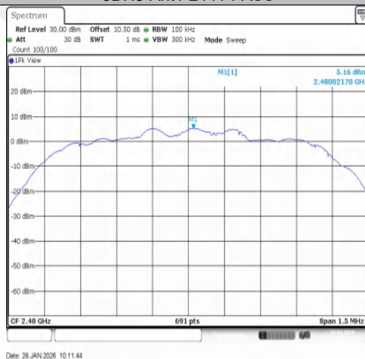
3DH5-Ant1-2480-PASS
