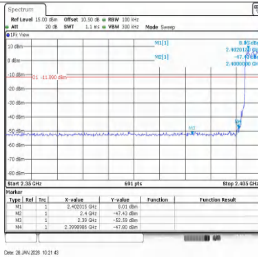
2DH5-Ant1-Hop_2402-PASS
