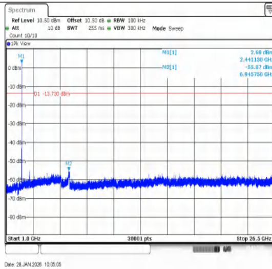
2DH5-Ant1-2441-1000~26500-PASS
