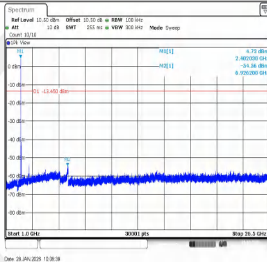
3DH5-Ant1-2402-1000~26500-PASS
