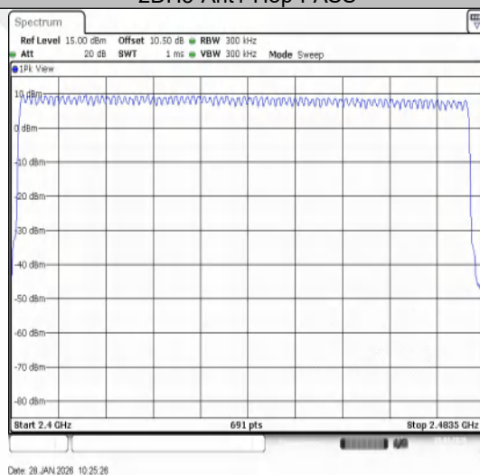
3DH5-Ant1-Hop-PASS
