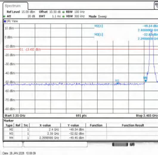
3DH5-Ant1-2402-PASS
