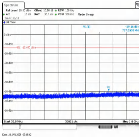
2DH5-Ant1-2402-30~1000-PASS
