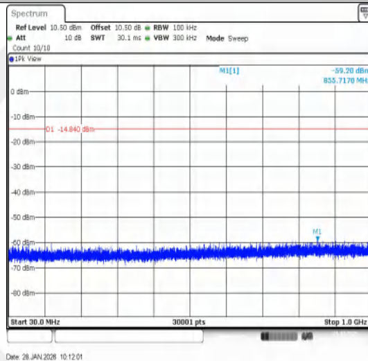
3DH5-Ant1-2480-30~1000-PASS
