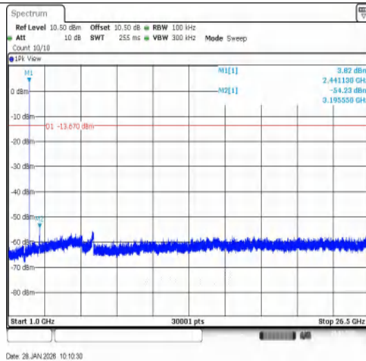
3DH5-Ant1-2441-1000~26500-PASS
