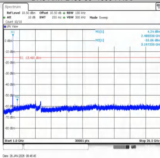
DH5-Ant1-2480-1000~26500-PASS
