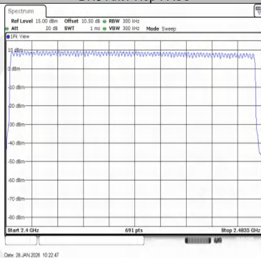
2DH5-Ant1-Hop-PASS
