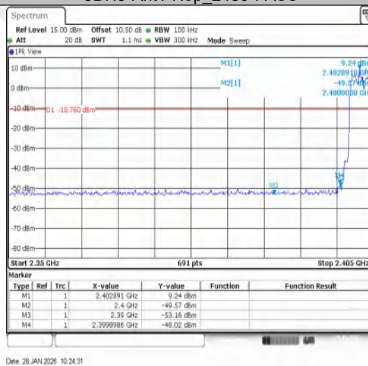
3DH5-Ant1-Hop_2402-PASS
