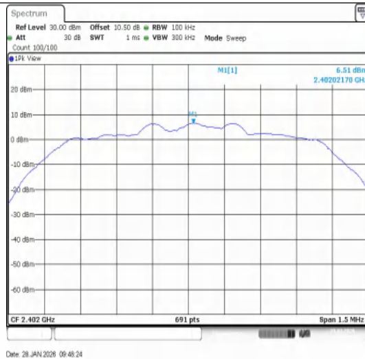
2DH5-Ant1-2402-PASS
