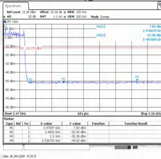
3DH5-Ant1-Hop_2480-PASS
