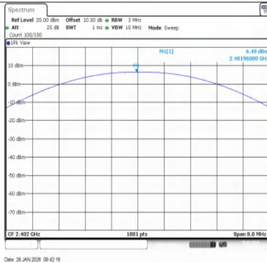
DH5-Ant1-2402-PASS
