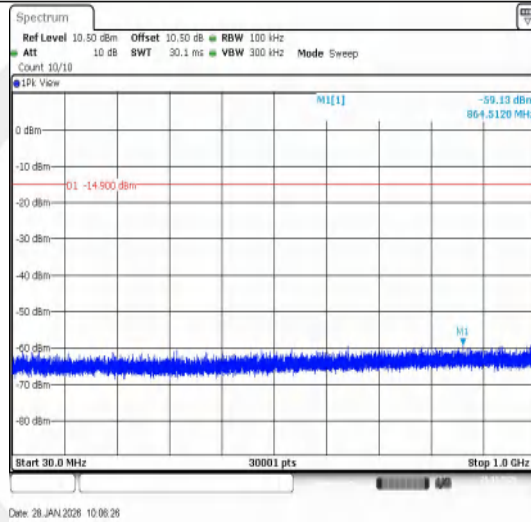
2DH5-Ant1-2480-30~1000-PASS
