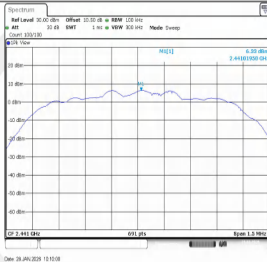
3DH5-Ant1-2441-PASS
