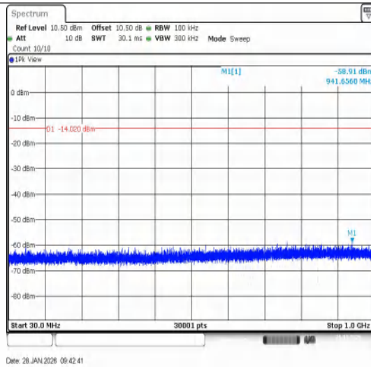
DH5-Ant1-2402-30~1000-PASS
