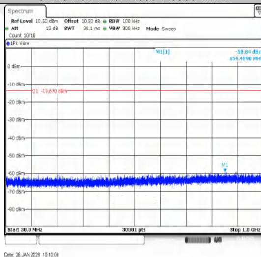
3DH5-Ant1-2441-30~1000-PASS
