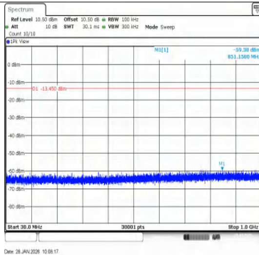
3DH5-Ant1-2402-30~1000-PASS
