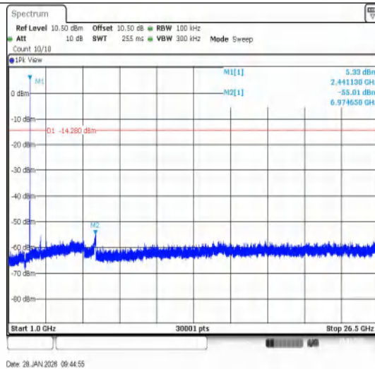
DH5-Ant1-2441-1000~26500-PASS
