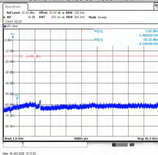
3DH5-Ant1-2480-1000~26500-PASS
