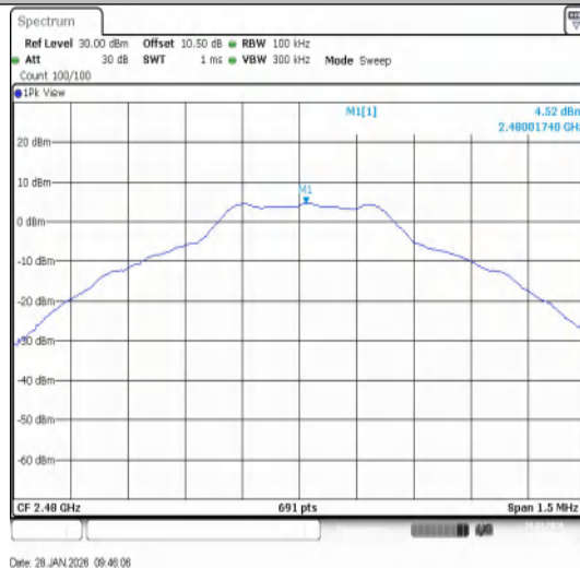
DH5-Ant1-2480-PASS
