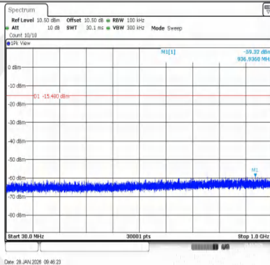
DH5-Ant1-2480-30~1000-PASS
