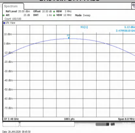
DH5-Ant1-2480-PASS
