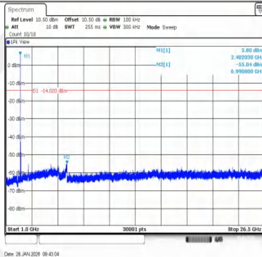
DH5-Ant1-2402-1000~26500-PASS
