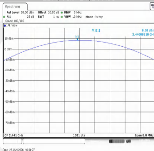
2DH5-Ant1-2441-PASS
