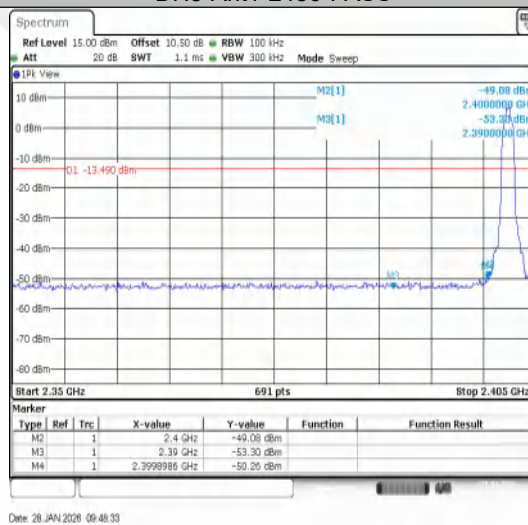
2DH5-Ant1-2402-PASS
