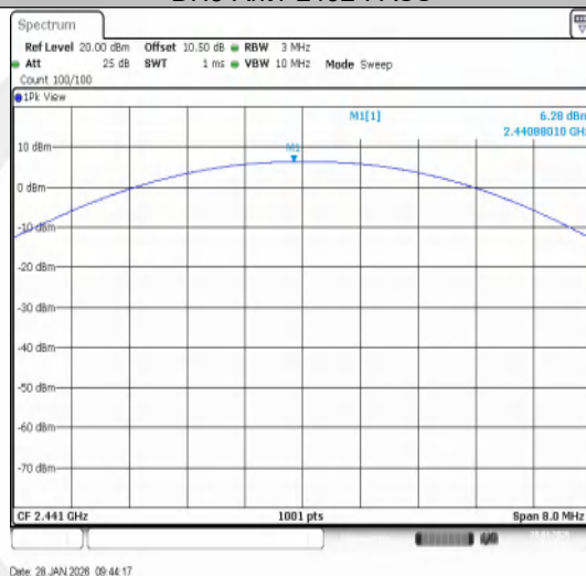
DH5-Ant1-2441-PASS
