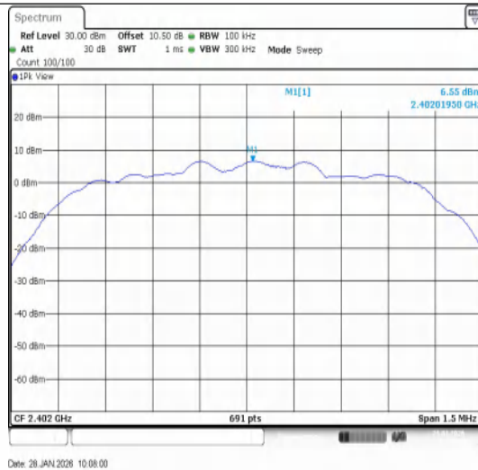
3DH5-Ant1-2402-PASS
