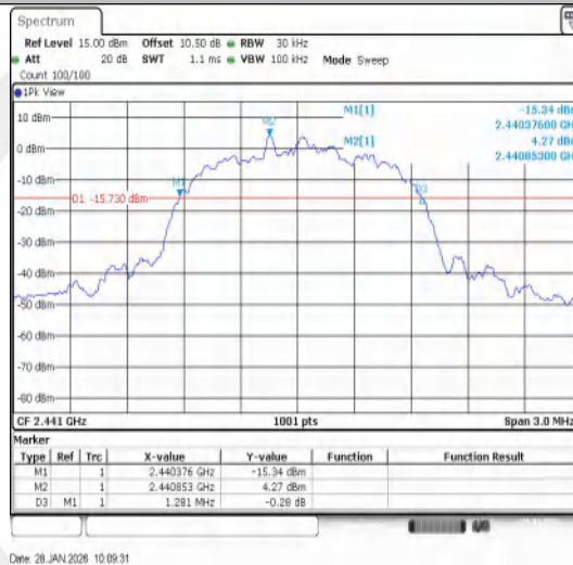
3DH5-Ant1-2441
