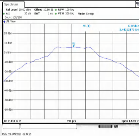
DH5-Ant1-2441-PASS
