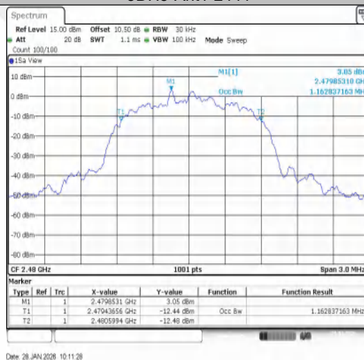
3DH5-Ant1-2480
