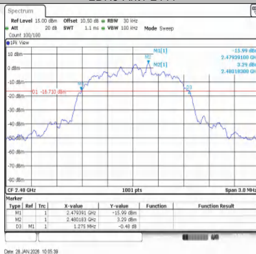
2DH5-Ant1-2480
