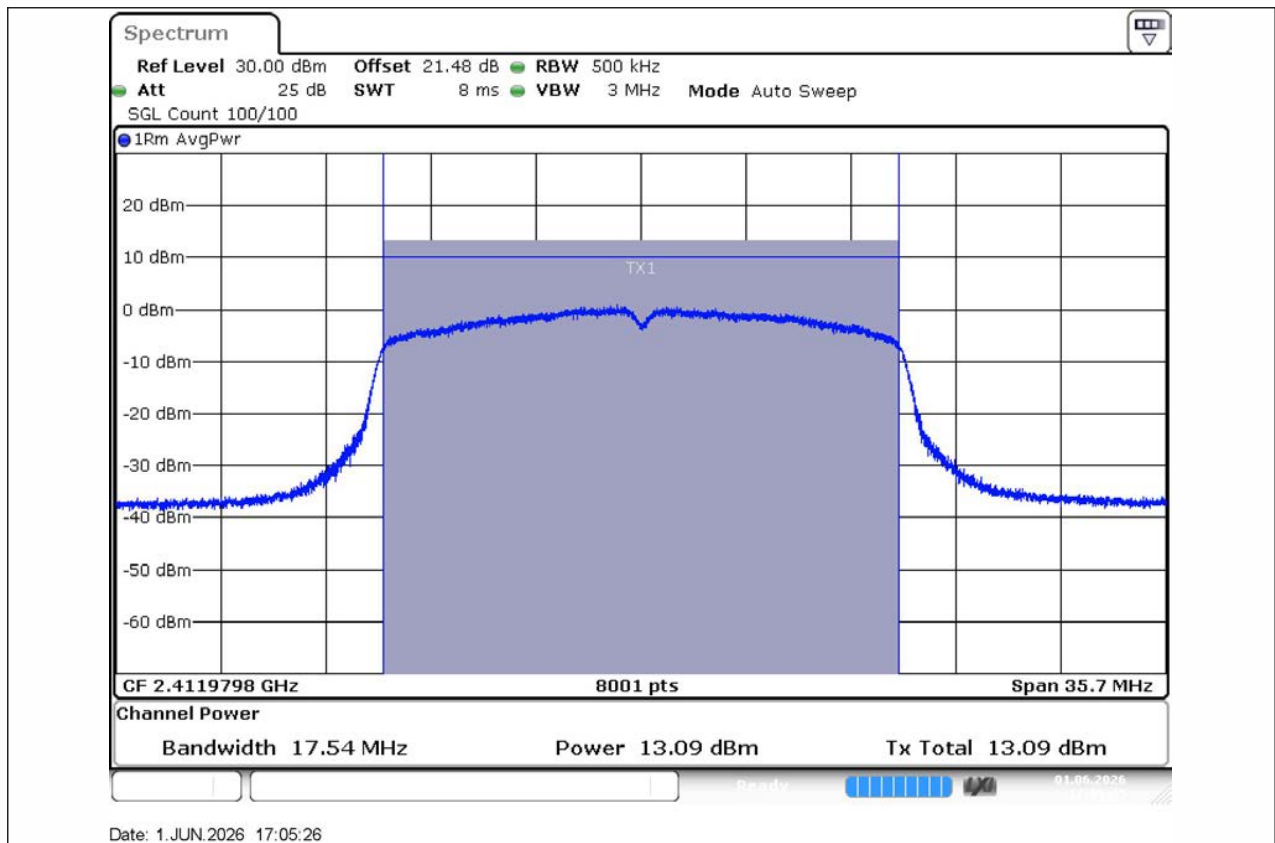
11N20SISO-Ant1-2412-PASS
