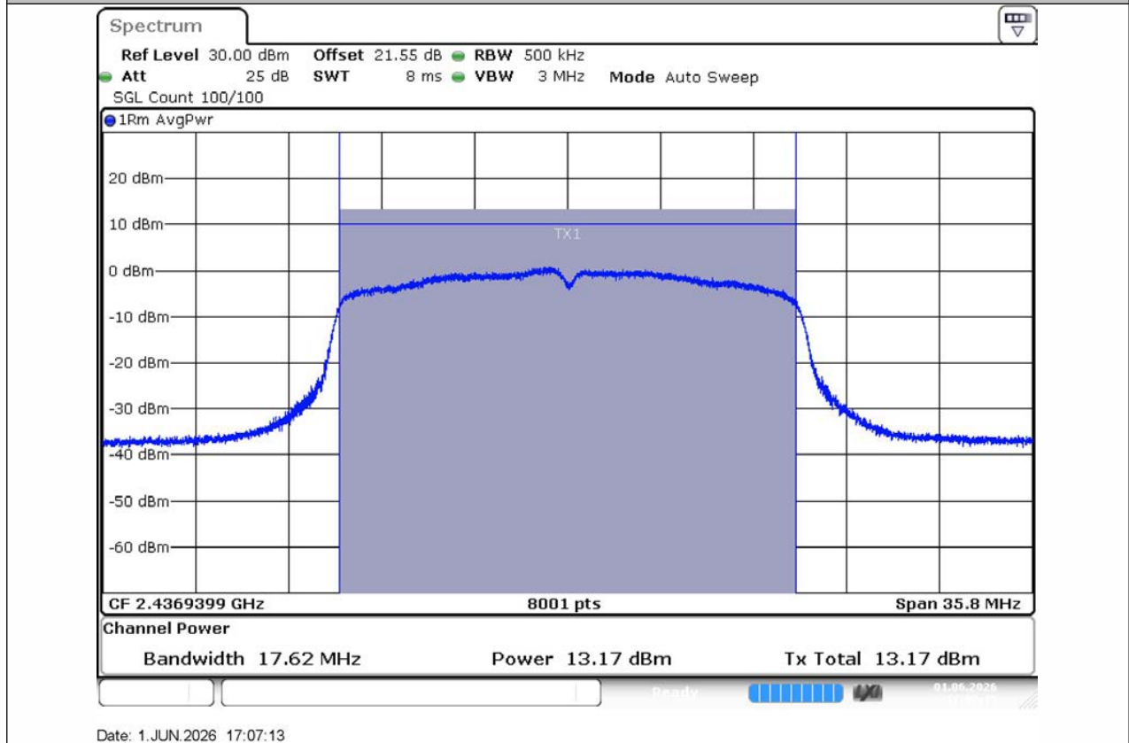
11N20SISO-Ant1-2437-PASS
