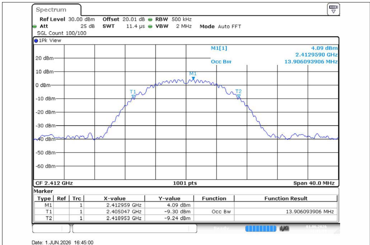
11B-Ant1-2412
