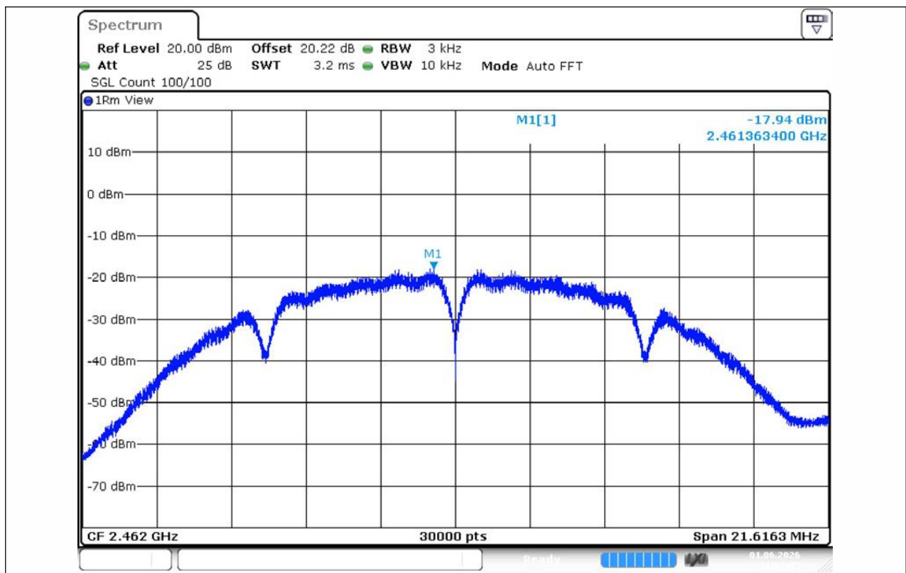
11B-Ant1-2462-PASS
