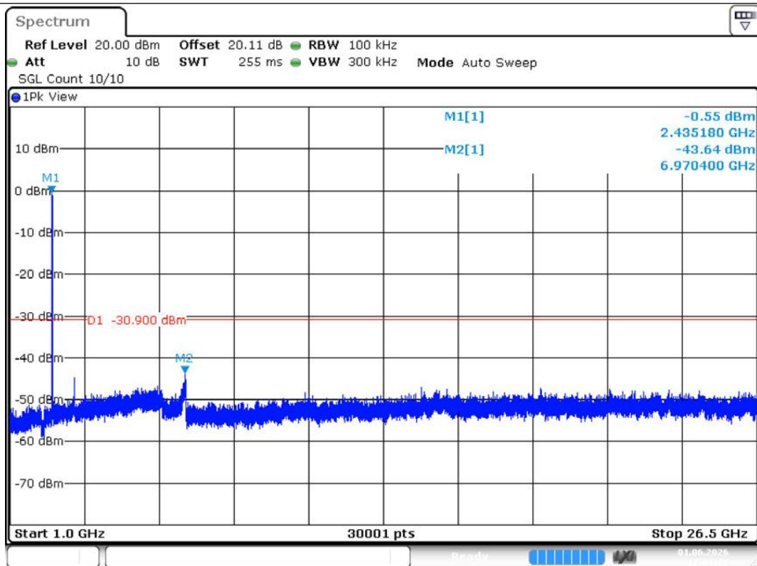
11G-Ant1-2437-1000~26500-PASS
