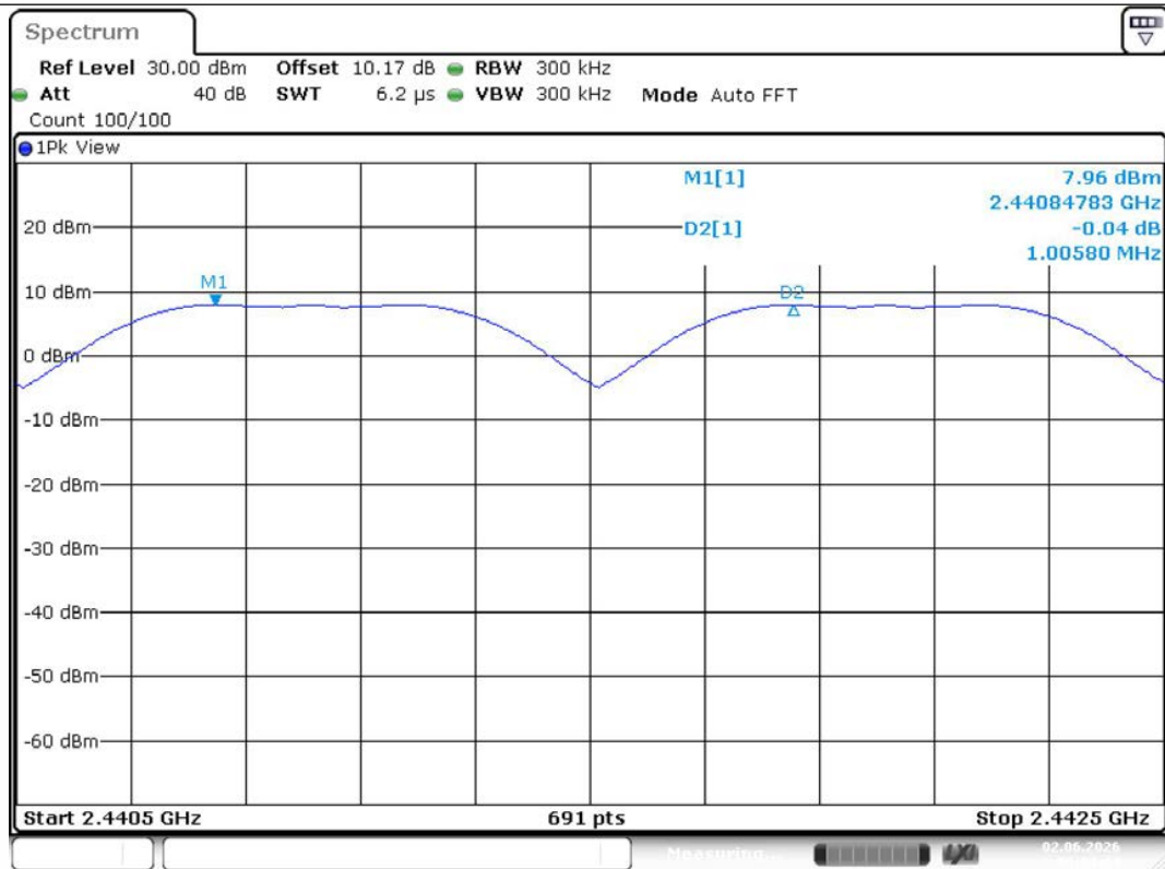
DH5-Ant1-Hop-PASS
