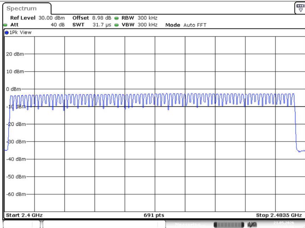
DH5-Ant1-Hop-PASS
