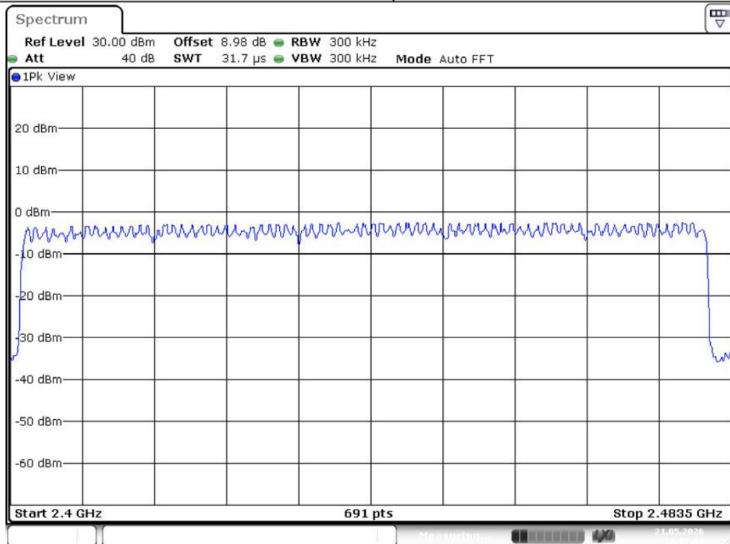
DH5-Ant1-Hop-PASS
