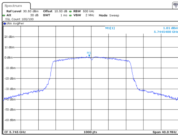
802.11ac20_5745MHz_Chain 0
