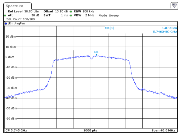
802.11ac20_5745MHz_Chain 1
