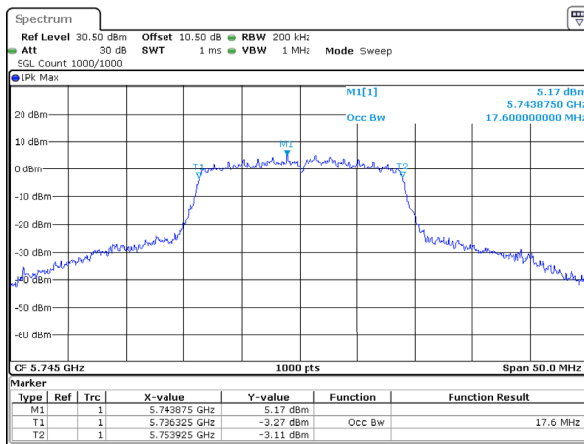
802.11ac20_5745MHz_Chain 0
