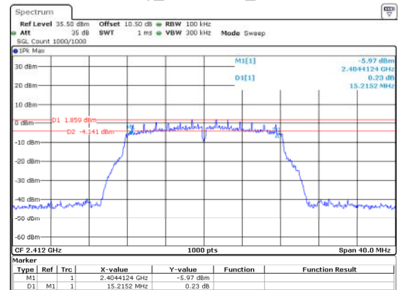
802.11g_2412MHz_Chain 1
