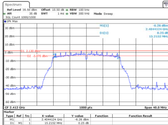
802.11g_2412MHz_Chain 0
