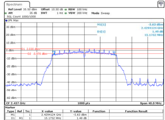
802.11g_2437MHz_Chain 0
