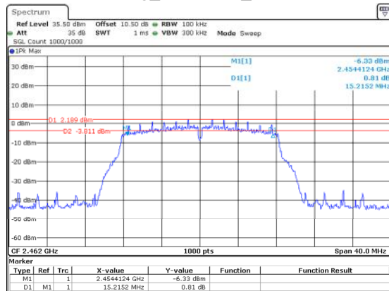
802.11g_2462MHz_Chain 0
