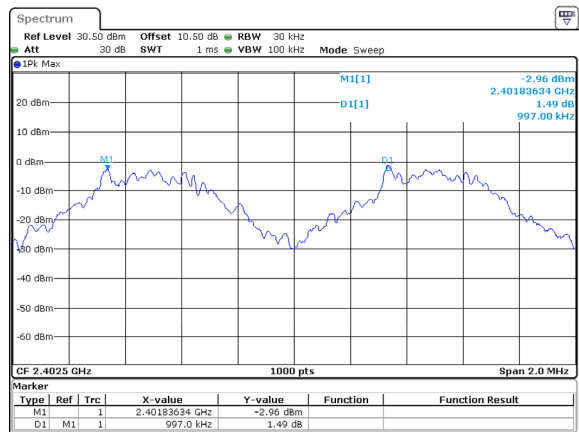
DH1_Low 0.997MHz
