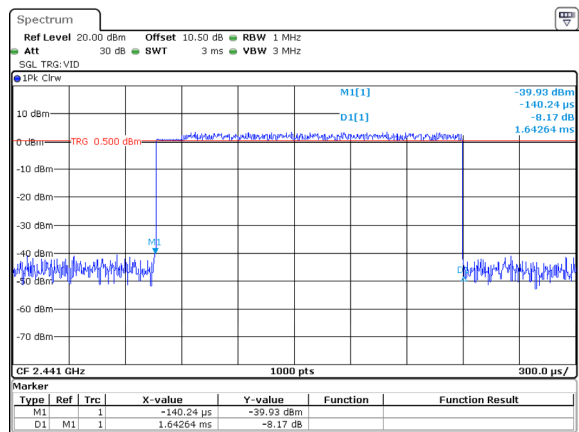
3DH3_Hopping 1.643ms
