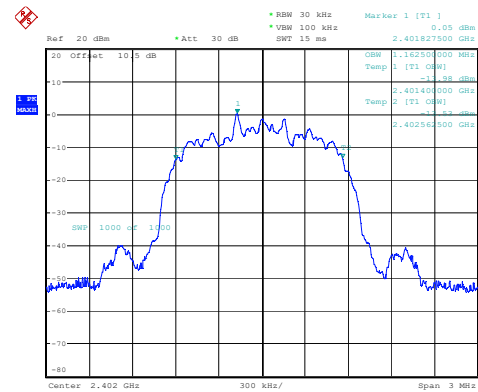
2DH1_Low 1.163MHz
