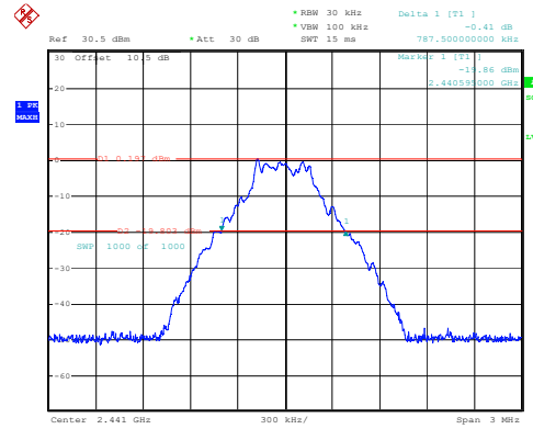
DH1_Middle 0.788MHz
