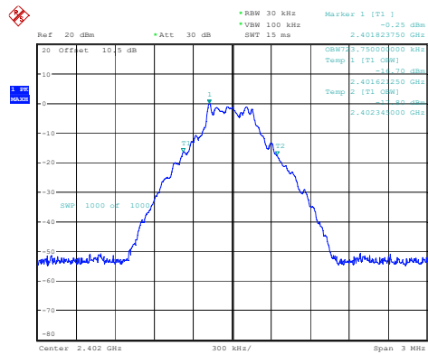
DH1_Low 0.724MHz
