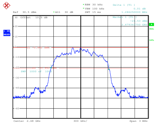
3DH1_High 1.286MHz
