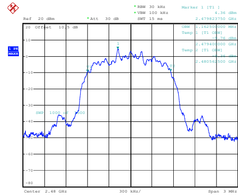
2DH1_High 1.163MHz
