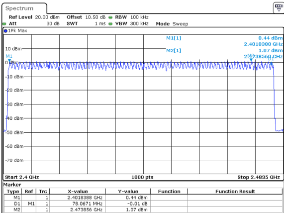
2DH1_Hopping 79
