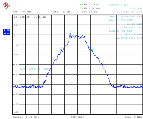
DH1_High 0.724MHz
