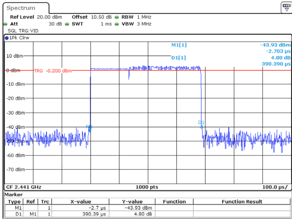
2DH1_Hopping 0.390ms
