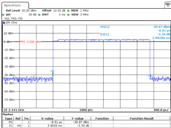
2DH5_Hopping 2.903ms
