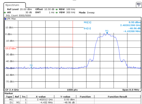
2DH1_Low
