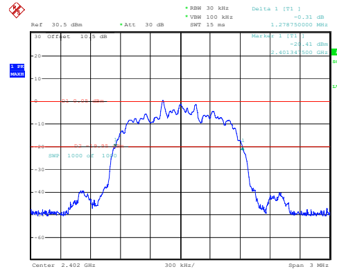
2DH1_Low 1.279MHz
