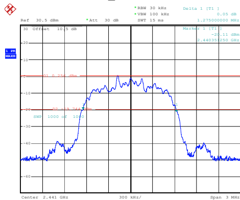
2DH1_Middle 1.275MHz
