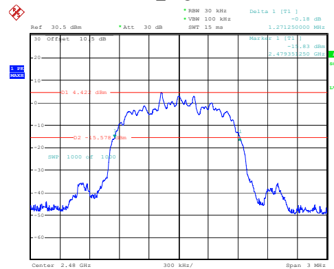
2DH1_High 1.271MHz
