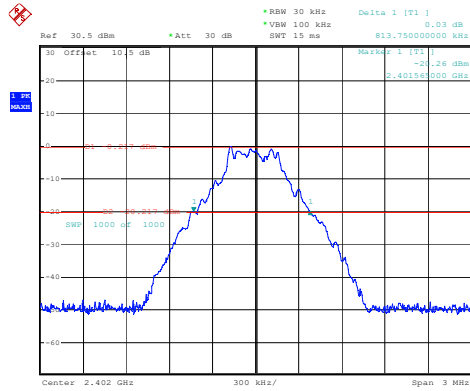
DH1_Low 0.814MHz
