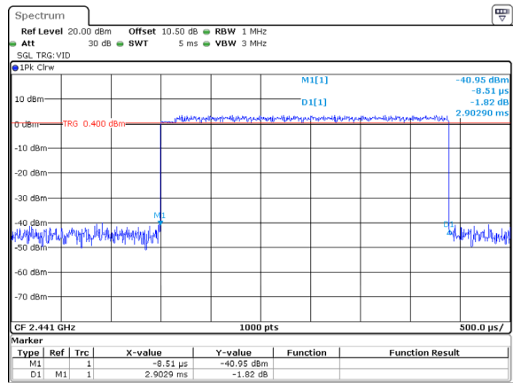
3DH5_Hopping 2.903ms
