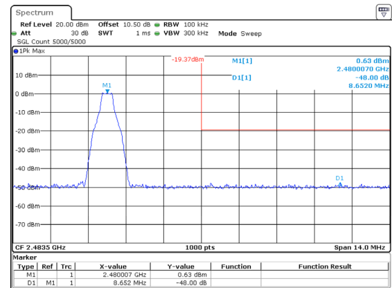
DH1_High
