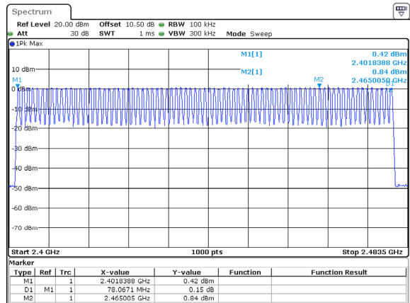
DH1_Hopping 79
