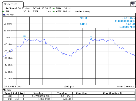
DH1_High 1.003MHz
