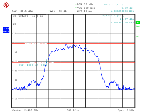
3DH1_Low 1.286MHz
