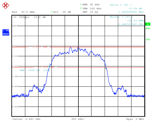
3DH1_Middle 1.283MHz
