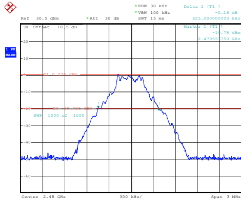
DH1_High 0.825MHz
