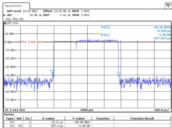
3DH1_Hopping 0.397ms
