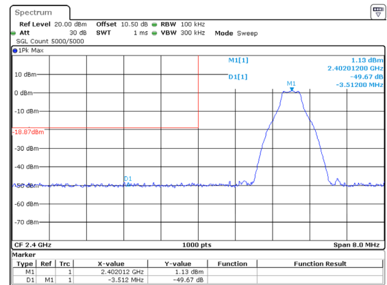
DH1_Low
