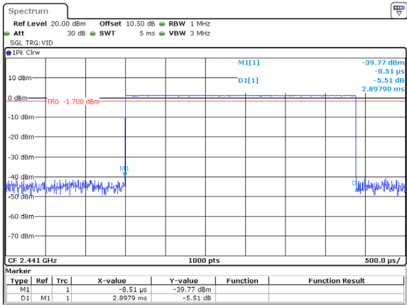
DH5_Hopping 2.898ms
