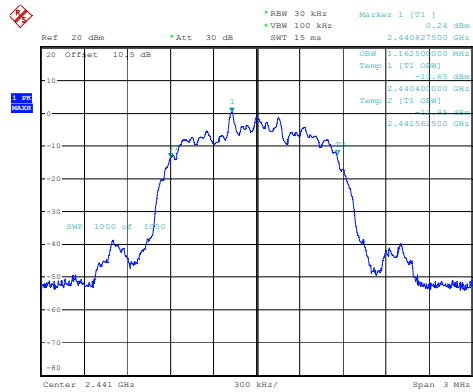
2DH1_Middle 1.163MHz
