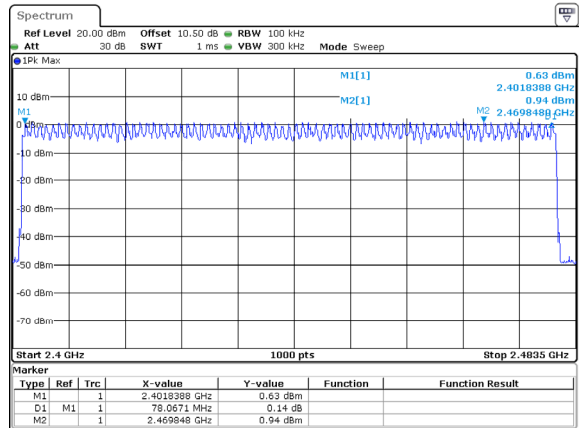
3DH1_Hopping 79
