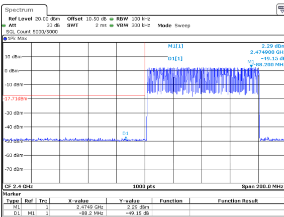
DH1_Hopping_Lower
