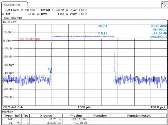
DH1_Hopping 0.393ms
