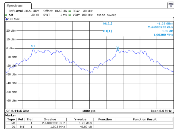
DH1_Middle 1.003MHz
