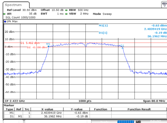
802.11n40_2422MHz_Chain 0
