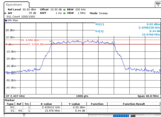
802.11g_2437MHz_Chain 0
