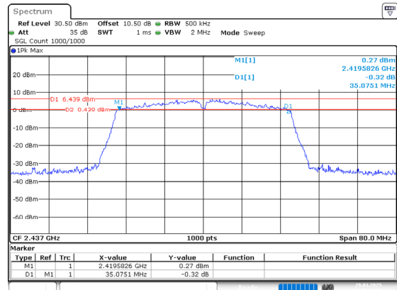
802.11n40_2437MHz_Chain 0
