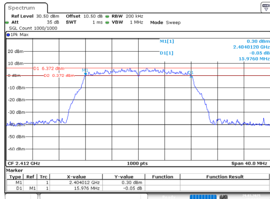
802.11g_2412MHz_Chain 0
