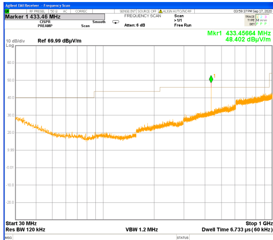
Plot # 5. Vertical polarization
