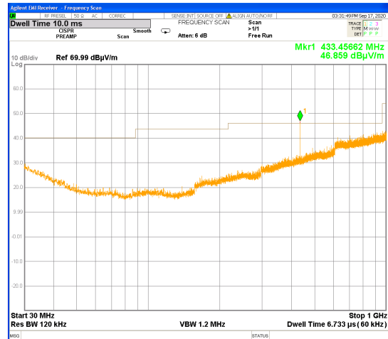
Plot # 3. Horizontal polarization
