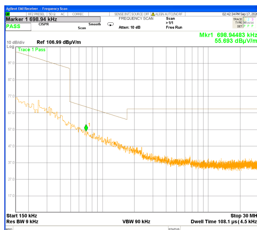
Plot # 1. Spurious emissions scan 0.15 MHz – 30 MHz.
