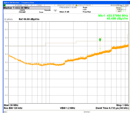
Plot # 6. Horizontal polarization
