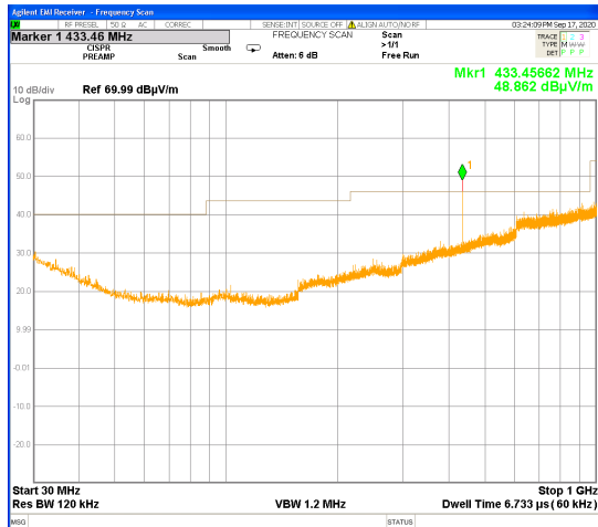
Plot # 2. Vertical polarization
