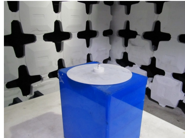
Radiated emissions test set outside human body simulator. General view
