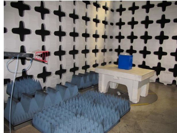
Radiated emissions test set in 1-5GHz freq. range outside human body simulator.
