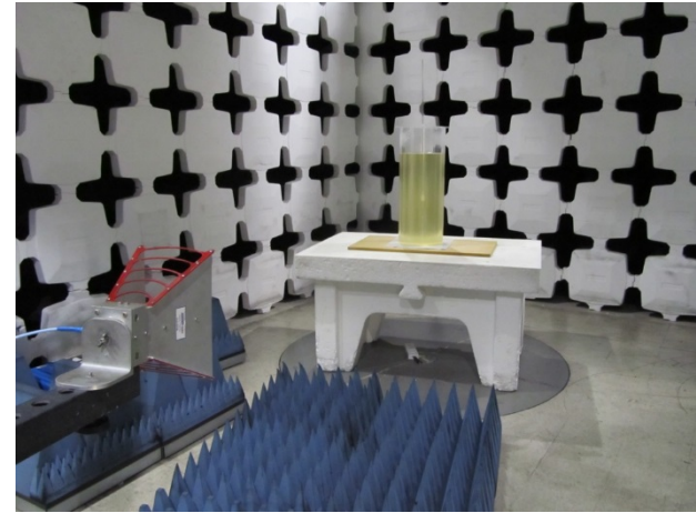
Radiated emissions test set in 1-5GHz freq. range inside human body simulator.
