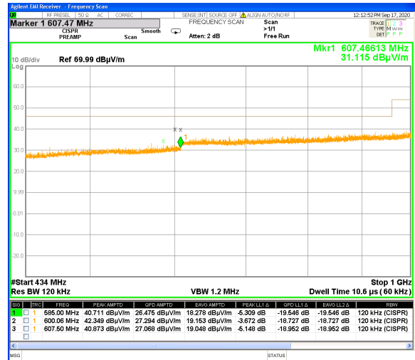
Plot # 5. Spurious emissions scan 434.0 MHz – 1000 MHz.
