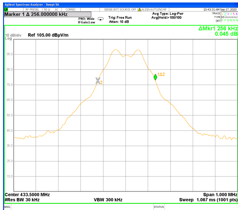
Plot # 12. Occupied bandwidth test result
