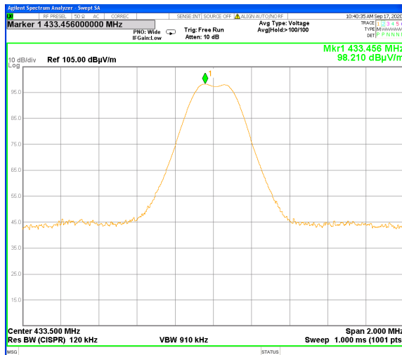
Plot # 1. Left side transmitter.
