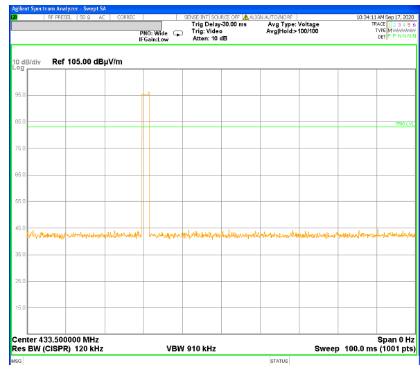
Plot # 10. Transmission in 100 msec.
