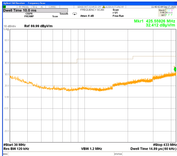
Plot # 4. Spurious emissions scan 30 MHz – 433.0 MHz.
