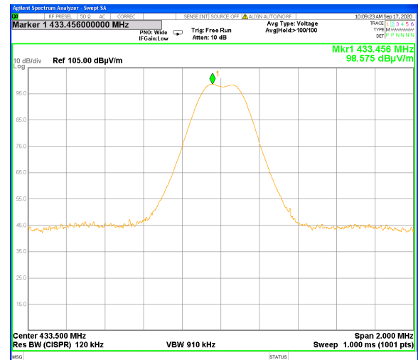
Plot # 2. Right side transmitter
