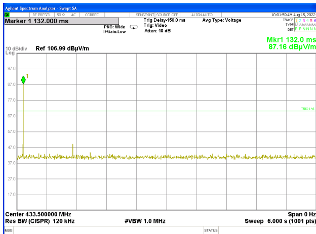
Plot # 11. Transmission in 6 sec.
