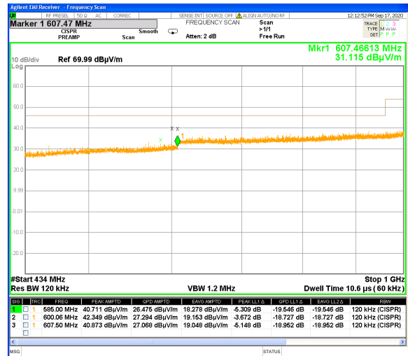
Plot # 5. Spurious emissions scan 434.0 MHz – 1000 MHz.
