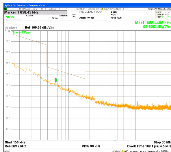
Plot # 3. Spurious emissions scan 0.15 MHz – 30 MHz.
