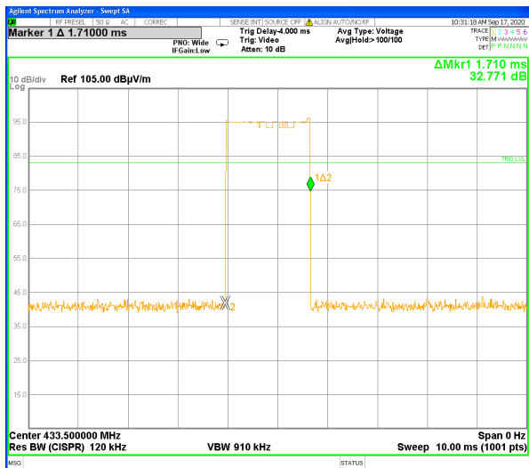
Plot # 9. Transmission duration test.
