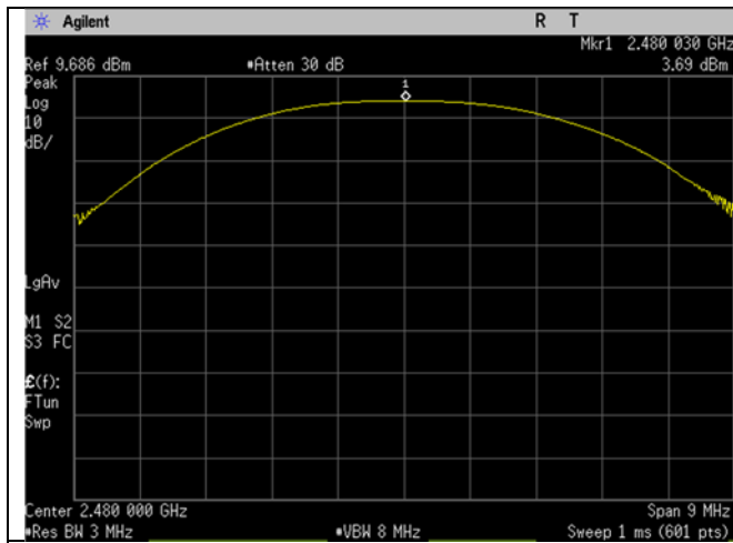
High Ch_2480MHz_1MBit_Output Power
