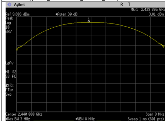
Mid Ch_2440MHz_1MBit_Output Power
