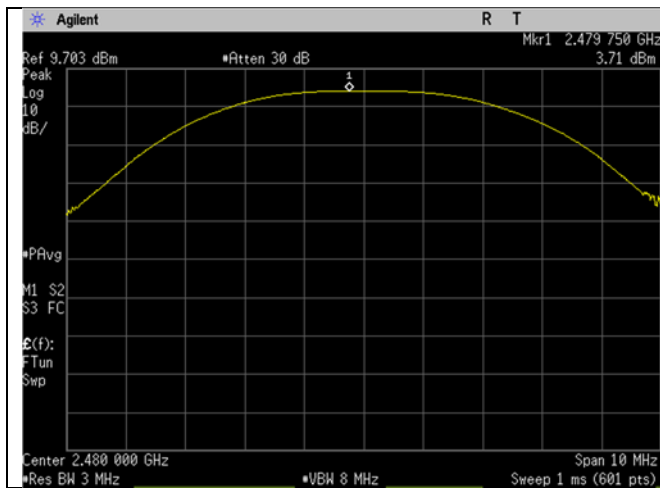
High Ch_2480MHz_2MBit_Output Power
