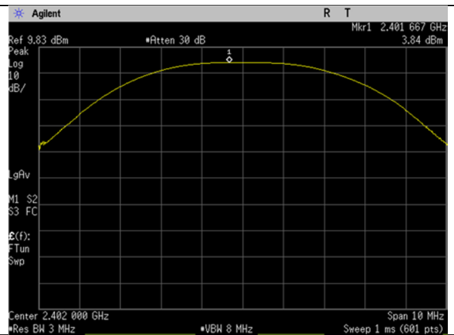
Low Ch_2402MHz_2MBit_Output Power
