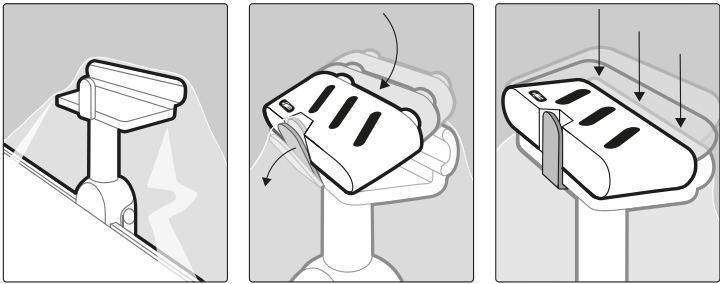
Figure 9 AltaTrack Docking Top attached to the AltaTrack docking base
