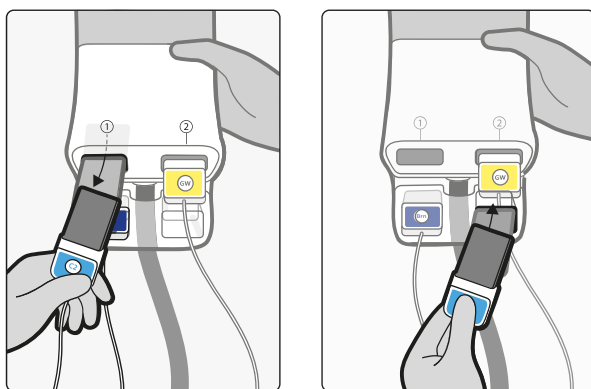
Figure 50 Disconnecting a device connector from the AltaTrack connection box
