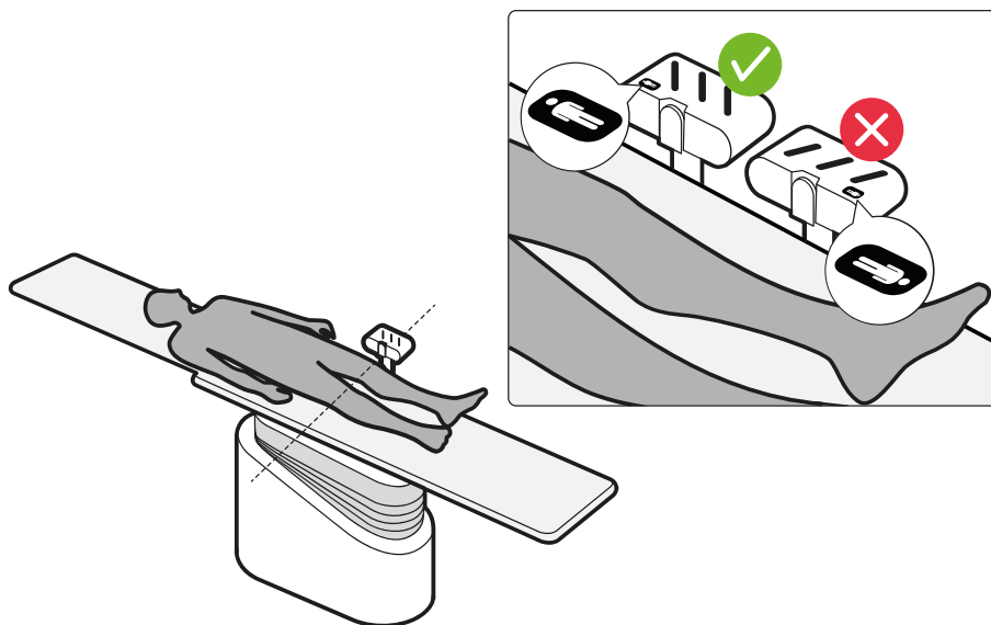
Figure 20 AltaTrack Docking Top orientation
