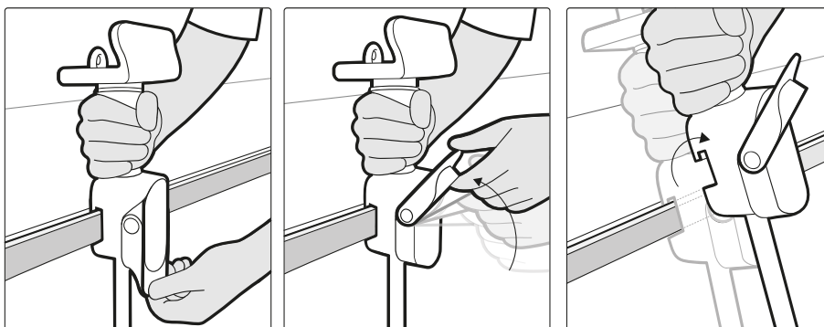
Figure 55 Removing the AltaTrack docking base
