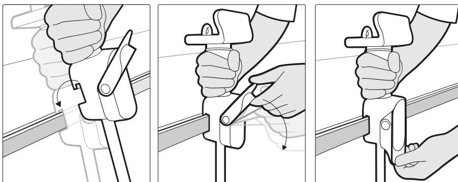
Figure 17 Attaching the AltaTrack docking base to the table accessory rail
