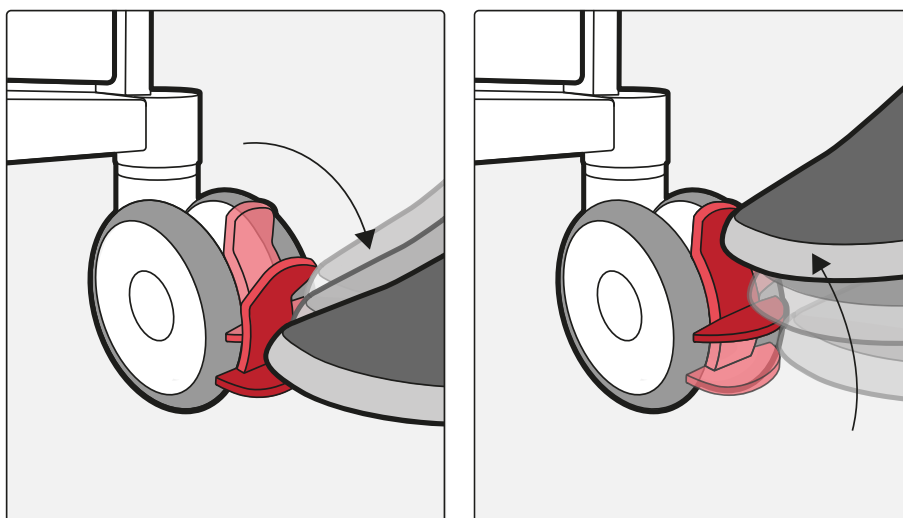
Figure 13 AltaTrack trolley brakes: applying the brake (left) and releasing the brake (right)
