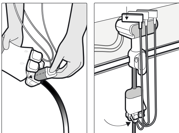
Figure 35 Setting up an additional device connector
