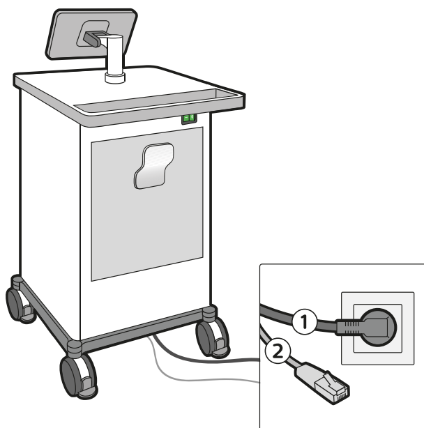
Figure 14 AltaTrack trolley cables
