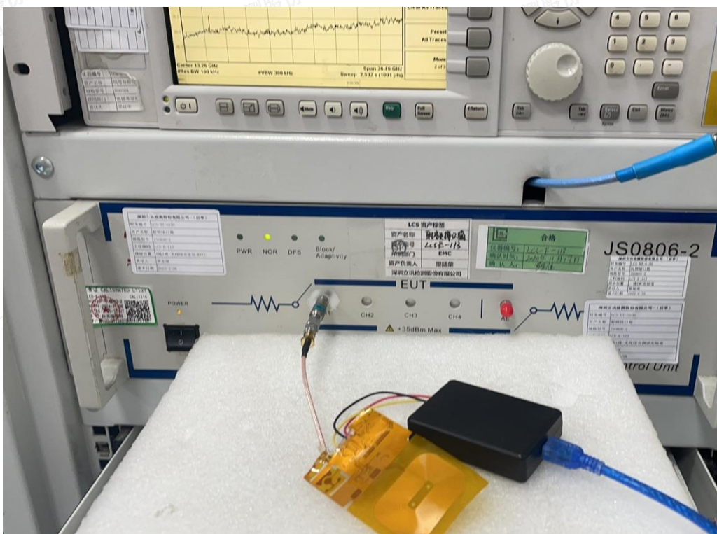
Fig. 3 RF Conducted
