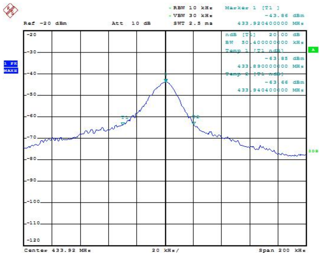
20dB Bandwidth Test Plot
