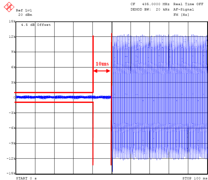
Transmitter Frequency Behavior @ 12.5 KHz Channel Separation-----On – Off
